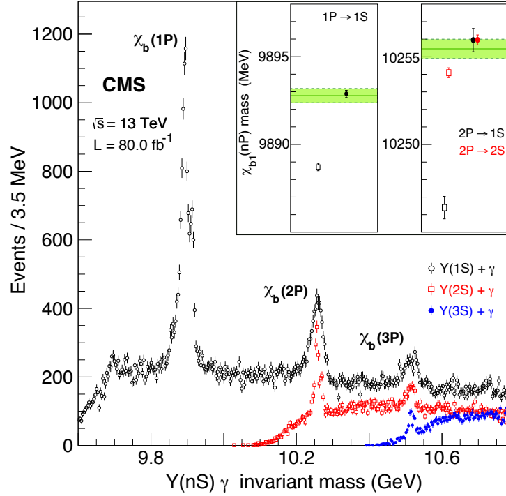
Figure 3: The invariant mass distributions of the \chi_{bJ} \rightarrow Y(nS) \gamma candidates ( n = 1, 2, 3 ), after the PES correction. The inset shows the \chi_{b1}(1P) and \chi_{b1}(2P) masses fitted before (open squares) and after (filled circles) the PES correction, with vertical bars representing the statistical uncertainties. The world-average values [33] are shown by the horizontal bands, with dashed lines representing their total uncertainties.
