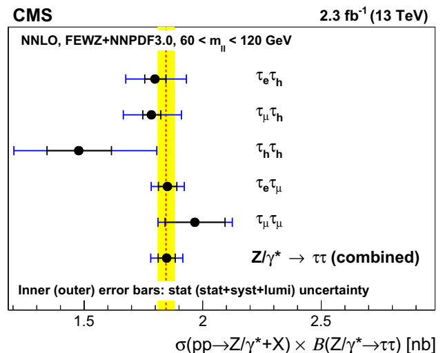
Fig. 12 The inclusive cross section \sigma(\text{pp} \rightarrow Z/\gamma^* + X) \mathcal{B}(Z/\gamma^* \rightarrow \tau\tau) measured in individual channels, and in the combination of all final states, compared to the theoretical prediction [60]
