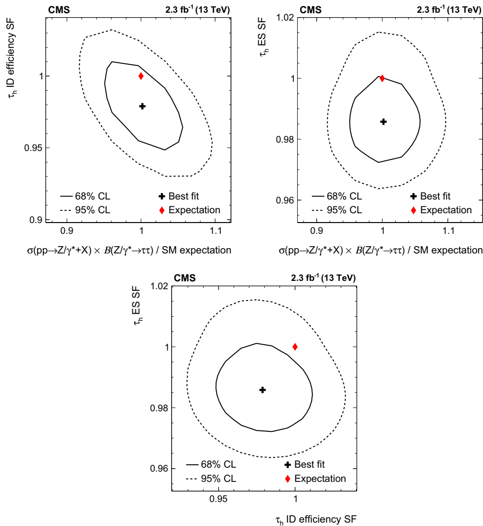
Fig. 13 Likelihood contours for the joint parameter estimation of (upper left) \sigma(pp \rightarrow Z/\gamma^* + X) B(Z/\gamma^* \rightarrow \tau\tau) and the \tau_h ID efficiency, (upper right) \sigma(pp \rightarrow Z/\gamma^* + X) B(Z/\gamma^* \rightarrow \tau\tau) and \tau_h ES, and (lower) the \tau_h ES and the \tau_h ID efficiency, at 68 and 95% confi-
