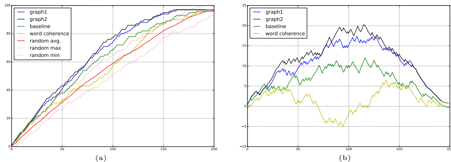
Figure 3: Semantic topics discovered (y-axis) per model topics examined (x-axis): (a) absolute number of topics discovered and (b) the average difference between the number of topics discovered when using ordering based on a topic coherence measure and random ordering.
