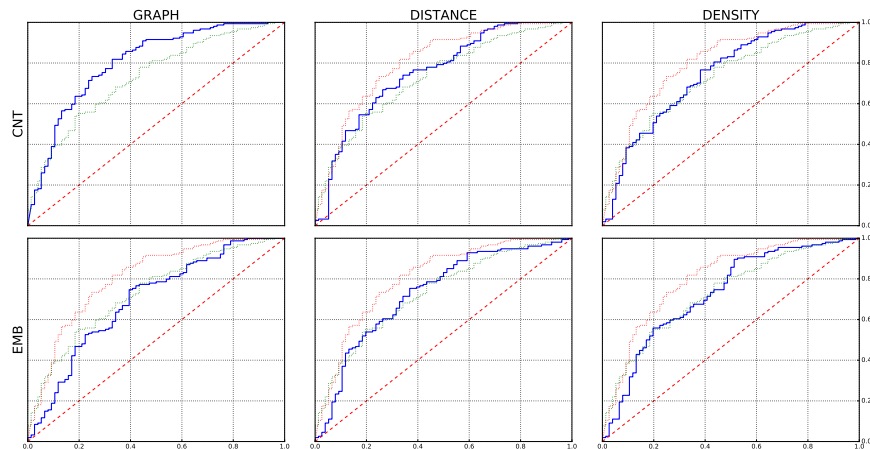
Figure 2: ROC curves of the best-performing coherence measures from the Table 4. The curve of the baseline measure is plotted in green on each plot. The curve of the measure from the top-performing category (top left) is plotted in red on other measures’ plots.
