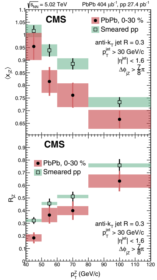
FIG. 3. The mean value of the x_{jZ} distribution (top) and the average number of jet partners per Z boson R_{jZ} (bottom), as a function of p_T^Z . Vertical lines (bands) indicate statistical (systematic) uncertainties.
