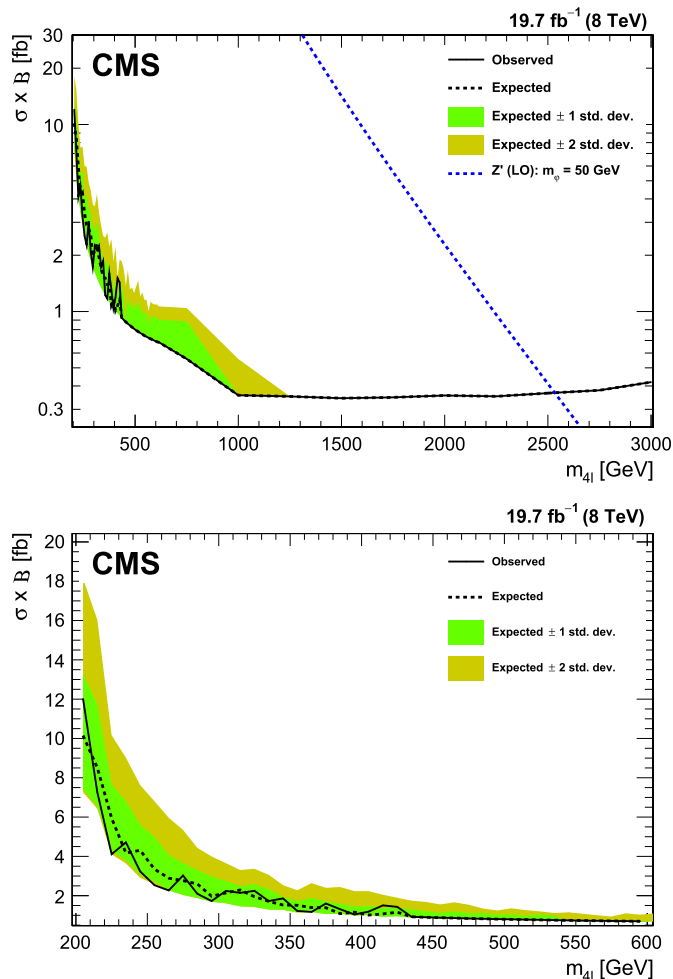
Fig. 3. The 95% CL upper limit on the cross section times branching fraction as a function of m_{4\ell} for the combination of the five channels: full mass range (top) and expanded view of the low mass region (bottom). The shaded green (yellow) band indicates the one (two) sigma uncertainty in the expected limits. The blue dashed line represents the theoretical predictions for the benchmark model [29] for m_\phi = 50 GeV. (For interpretation of the references to colour in this figure legend, the reader is referred to the web version of this article.)
