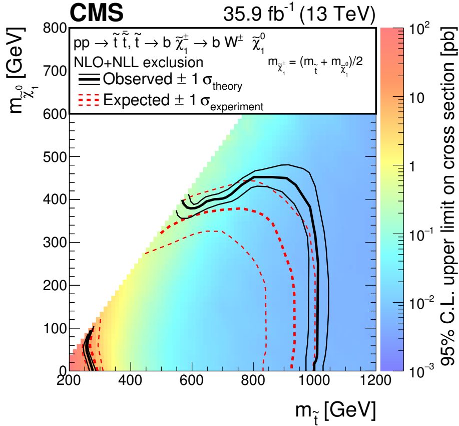
Figure 6. The exclusion limit at 95% CL for direct top squark pair production with decay \tilde{t}\tilde{t} \rightarrow b\tilde{\chi}_1^+\tilde{b}\tilde{\chi}_1^- , \tilde{\chi}_1^\pm \rightarrow W^\pm\tilde{\chi}_1^0 . The mass of the chargino is chosen to be (m_{\tilde{t}} + m_{\tilde{\chi}_1^0})/2 . The interpretation is done in the two-dimensional space of m_{\tilde{t}} vs. m_{\tilde{\chi}_1^0} . The color indicates the 95% CL upper limit on the cross section times branching fraction at each point in the m_{\tilde{t}} vs. m_{\tilde{\chi}_1^0} plane. The area between the thick black curves represents the observed exclusion region at 95% CL assuming 100% branching fraction, while the dashed red lines indicate the expected limits at 95% CL and their \pm 1\sigma experimental standard deviation uncertainties. The thin black lines show the effect of the theoretical uncertainties ( \sigma_{\text{theory}} ) in the signal cross section.
