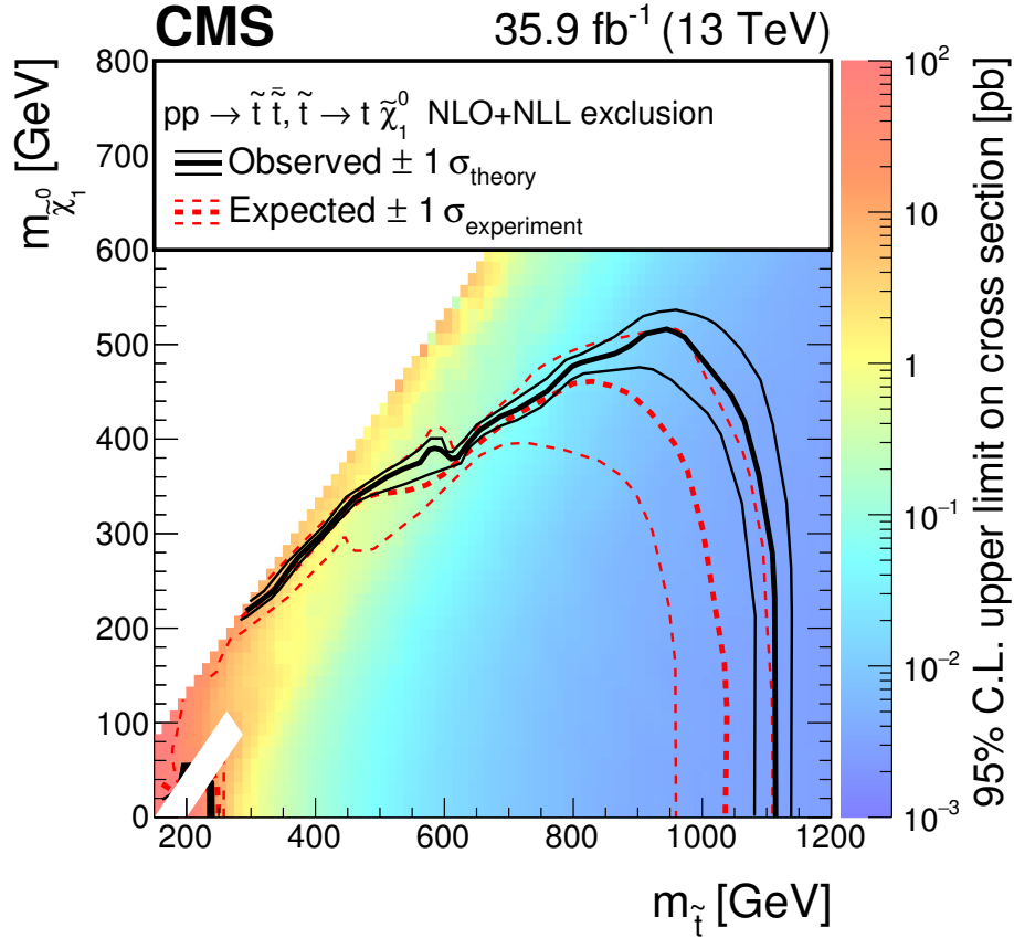
Figure 5. The exclusion limits at 95% CL for direct top squark pair production with decay \tilde{t}\tilde{t} \rightarrow t\tilde{\chi}_1^0 \bar{t}\tilde{\chi}_1^0 . The interpretation is done in the two-dimensional space of m_{\tilde{t}} vs. m_{\tilde{\chi}_1^0} . The color indicates the 95% CL upper limit on the cross section times branching fraction at each point in the m_{\tilde{t}} vs. m_{\tilde{\chi}_1^0} plane. The area below the thick black curve represents the observed exclusion region at 95% CL assuming 100% branching fraction, while the dashed red lines indicate the expected limits at 95% CL and their \pm 1\sigma experimental standard deviation uncertainties. The thin black lines show the effect of the theoretical uncertainties ( \sigma_{\text{theory}} ) in the signal cross section. The white out region is discussed in section 7.
