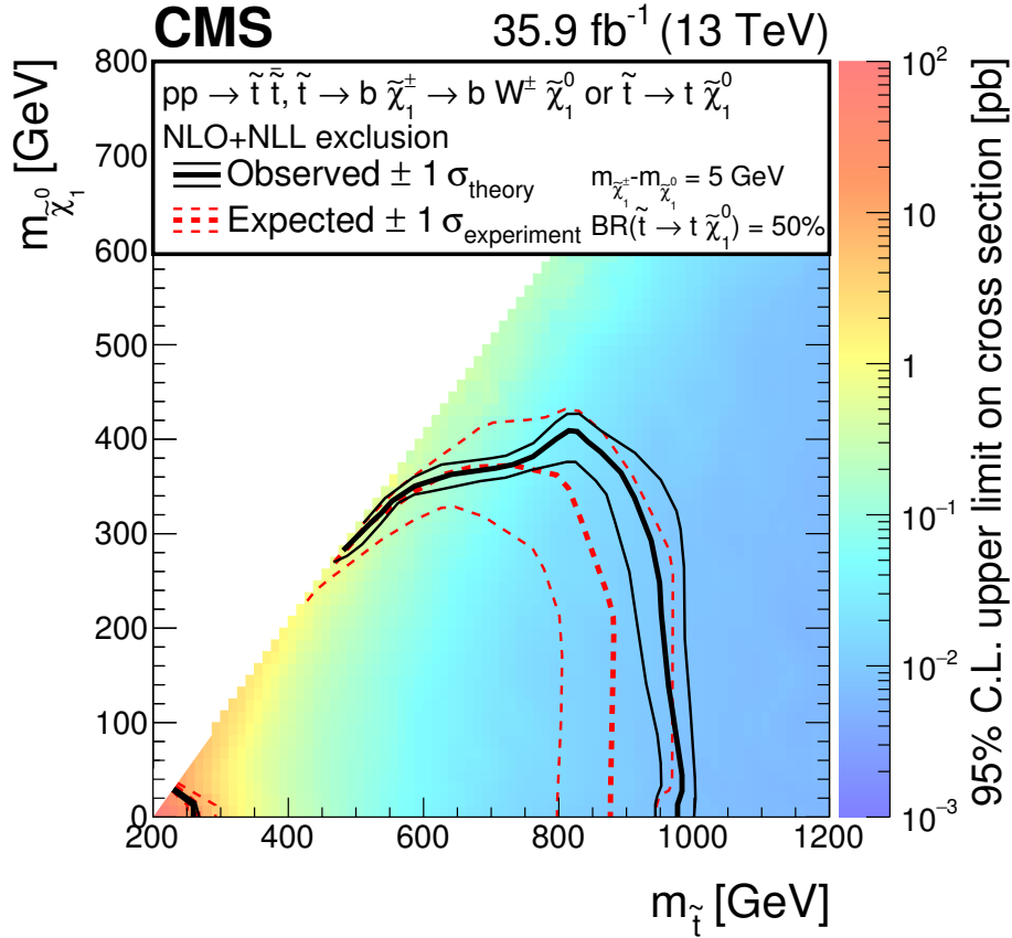
Figure 7. The exclusion limit at 95% CL for direct top squark pair production with decay \tilde{t}\tilde{t} \rightarrow b\tilde{\chi}_1^+\tilde{t}\tilde{\chi}_1^0, \tilde{\chi}_1^\pm \rightarrow W^\pm\tilde{\chi}_1^0 . The mass splitting of the chargino and neutralino is fixed to 5 GeV. The interpretation is done in the two-dimensional space of m_{\tilde{t}} vs. m_{\tilde{\chi}_1^0} . The color indicates the 95% CL upper limit on the cross section at each point in the m_{\tilde{t}} vs. m_{\tilde{\chi}_1^0} plane. The area between the thick black curves represents the observed exclusion region at 95% CL, while the dashed red lines indicate the expected limits at 95% CL and their \pm 1\sigma experimental standard deviation uncertainties. The thin black lines show the effect of the theoretical uncertainties ( \sigma_{\text{theory}} ) in the signal cross section.
