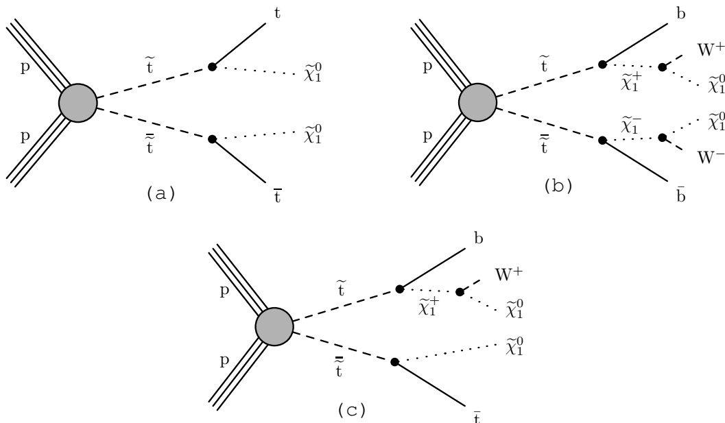
Figure 1. Simplified-models diagrams corresponding to top squark pair production, followed by the specific decay modes targeted in this paper. (a) pp \rightarrow \tilde{t}\tilde{t} \rightarrow t\tilde{\chi}_1^0 \bar{t}\tilde{\chi}_1^0 ; (b) pp \rightarrow \tilde{t}\tilde{t} \rightarrow b\tilde{\chi}_1^+ \bar{b}\tilde{\chi}_1^- ; (c) pp \rightarrow \tilde{t}\tilde{t} \rightarrow b\tilde{\chi}_1^+ \bar{t}\tilde{\chi}_1^0 . Charge-conjugate decays are implied.
