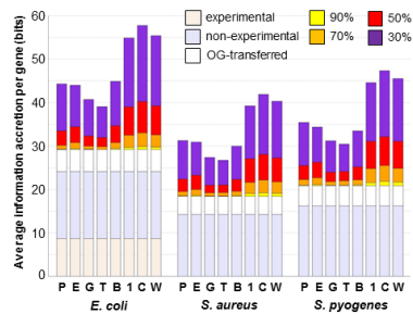
Fig. 5. Average information accretion per gene of known vs. newly predicted functional annotations. Three example genomes are shown. Darker colors show increase in predictions with decreasing stringency (numbers denote precision, Pr, threshold employed). Method/scheme name is denoted by the first letter of its name, except CGN=G.
