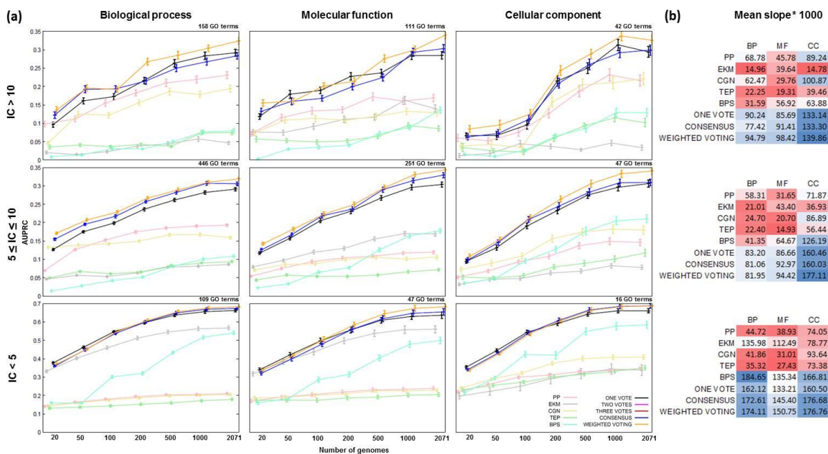
Fig. 6. Accuracy of classifiers increases with addition of genomic data. (a) X-axes represent the number of randomly sampled genomes (of the 2,071 total); approx. log scale. Y-axes represents classifiers' AUPRCs (in cross-validation) averaged over the selected subset of GO terms and error bars standard error of the mean. IC, information content. (b) Slopes of the regression lines for a prediction method/integration scheme, as average over the slopes of segments connecting points in plot; complete table with slopes in Table S3.
