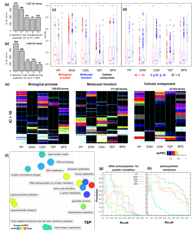
Fig. 2. Complementarity between the AFP methods. (a, b) The number of GO terms learnable by one, two or more classifiers. (c, d) Distributions of classifiers’ AUPRCs scores for GO terms, stratified by GO domain and by information content (IC); lower IC scores denote more general terms. (e) Complementarity patterns in high-IC domains, where rows represent GO terms, columns represent prediction methods and brighter colors relate to higher accuracy, as AUPRC score (in cross-validation). (f) Examples of GO terms learned by TEP better than by the rest of the classifiers. Excess AUPRC for a GO term (color) is computed by subtracting the AUPRC of the best-performing other classifier from the TEP AUPRC, for a particular GO. (g, h) Precision-recall curves for two selected GO terms where the TEP method performs well. PP, phyletic profiles; EKM, empirical kernel map; CGN, conserved gene neighborhoods; TEP, translation efficiency profiles; BPS, biophysical and protein sequence properties.
