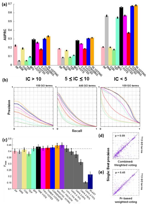
Fig. 3. Comparison of predictive performance between individual methods and integration schemes. (a) Average AUPRC scores for the Biological process GO domain computed from precision-recall (PR) curves, obtained in cross-validation. Error bars are standard error of the mean. IC, information content; lower IC denotes more general GO terms. (b) PR curves computed by averaging individual Biological process GO term PR curves, stratified by IC. (c) The F_{max} accuracy measure on the CAFA 2 E. coli validation set. Error bars are standard deviation by bootstrapping the set of benchmark genes. (d, e) Cross-validation AUPRC scores of the individual Biological process GO terms, while comparing the ‘best precision’ vs. the ‘weighted voting’ scheme (d) and a Pr-based weighted voting scheme in (e). p-values are by Wilcoxon test.
