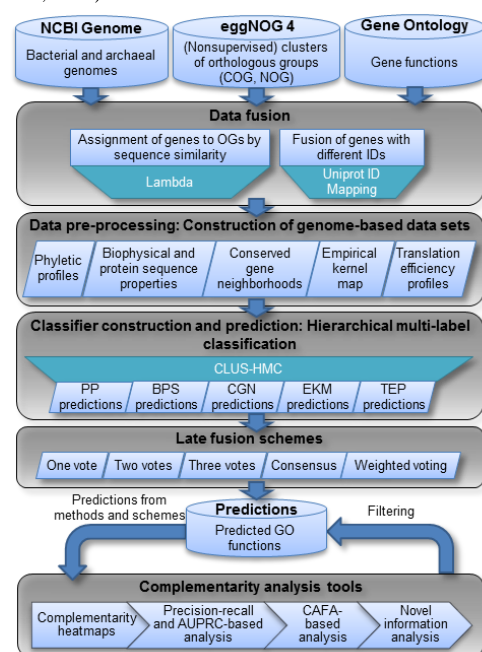
Fig. 1. A pipeline for automated function prediction from genomic data.
