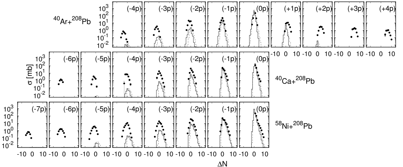
FIG. 7: Total experimental cross section for ^{40}\text{Ar} , ^{40}\text{Ca} , and ^{58}\text{Ni} induced reactions on the ^{208}\text{Pb} target, at beam energies E_{\text{lab}} = 6.4, 6.2, and 6 MeV/A, respectively, (points) and the GRAZING calculations with (full line) and without (dashed line) neutron evaporation.
