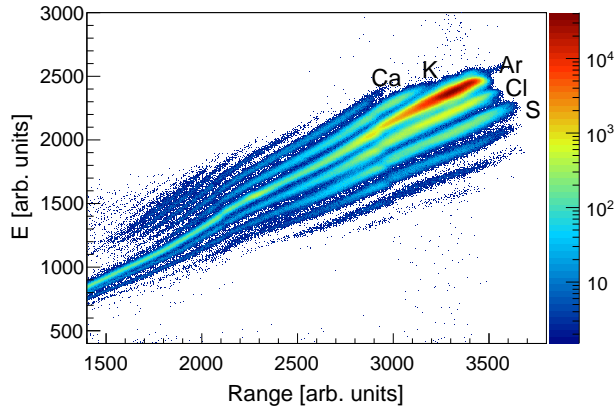
FIG. 1: (Color online) Matrix of Range versus energy E for the ^{40}\text{Ar}+^{208}\text{Pb} reaction at E_{\text{lab}} = 6.4 MeV/A and at \theta_{\text{lab}} = 54^\circ . The Range has been determined using the angle and position information of the ions entering the ionization chamber, together with the different IC sub-anodes information. The most intense band corresponds to Ar ions, with proton pick-up and proton stripping channels visible above and below Ar.
