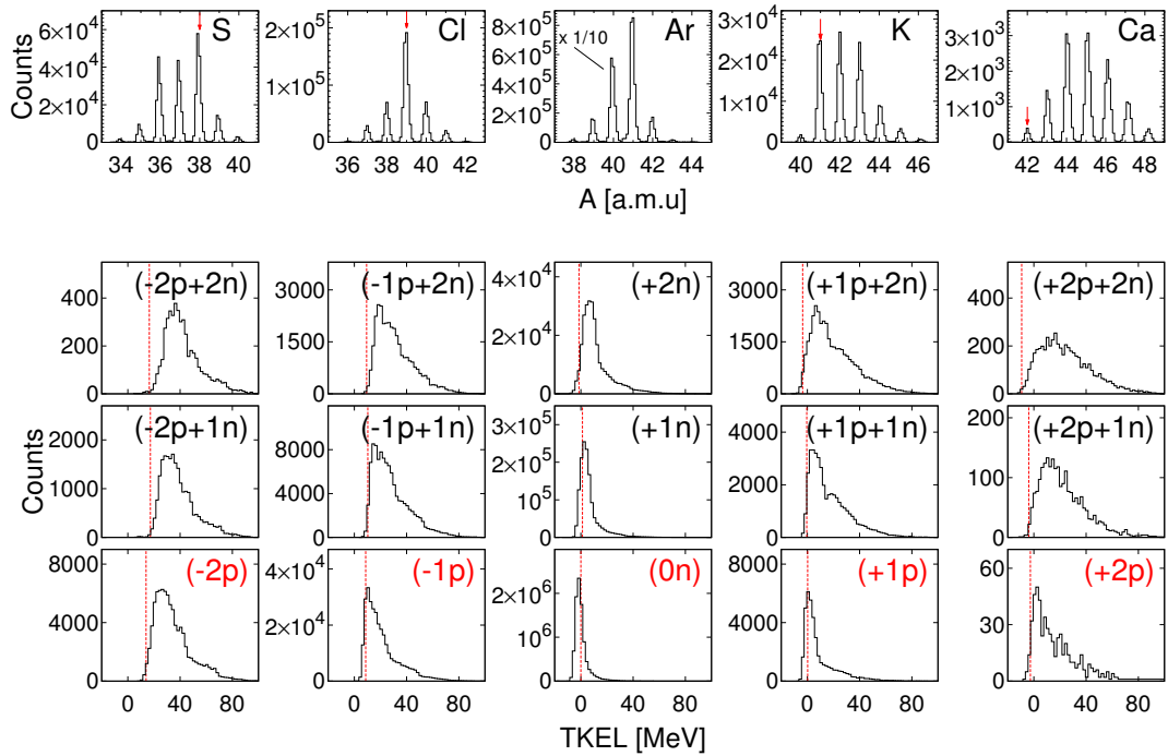
FIG. 3: (Color online) Experimental TKEL spectra for the indicated transfer channels at \theta_{\text{lab}} = 54^\circ . The vertical dashed lines represent the ground state Q values. In the top row the mass spectra for each Z are also depicted, with the red arrows indicating the pure proton transfer channels. The ^{40}\text{Ar} peak has been scaled down by a factor 10 to better display the behaviour of the transfer channels.
