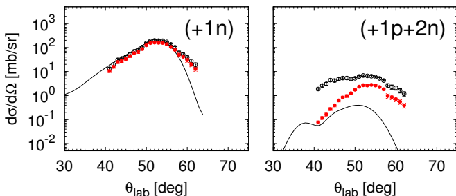
FIG. 6: (Color online) Experimental angular distributions of the (+1n) and (+1p+2n) channels integrated over the full TKEL range (black empty points) and integrated over the quasi-elastic part with the \text{TKEL} \leq 20 MeV (red full points). The results of the GRAZING calculations are also plotted (curves).
