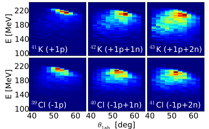
FIG. 4: (Color online) Wilczynski plots, kinetic energy E in the laboratory system versus \theta_{\text{lab}} , for selected channels in the ^{40}\text{Ar}+^{208}\text{Pb} reaction. The plots have been obtained by matching the measured events at the three PRISMA angular and magnetic settings.
