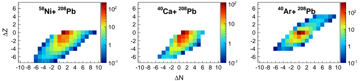
FIG. 8: (Color online) Angle and energy integrated total cross section for ^{40}\text{Ar} , ^{40}\text{Ca} , and ^{58}\text{Ni} projectiles on the ^{208}\text{Pb} target, at energies E_{\text{lab}} = 6.4, 6.2, and 6 MeV/A, respectively. The cross section values of the elastic(+inelastic) channel, with \Delta N and \Delta Z = 0 , have been scaled down by a factor 100 to better display the behaviour of the transfer channels.
