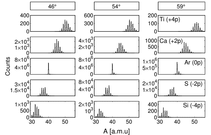
FIG. 2: Mass spectra for the transfer products measured in the ^{40}\text{Ar}+^{208}\text{Pb} reaction, spanning the range from (+4p) to (-4p) channels for even Z isotopes for the three measured angles.
