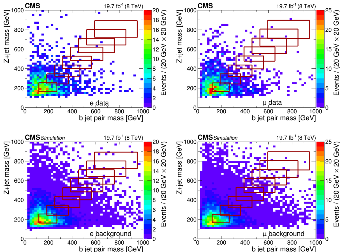
Figure 6. Distributions of the Z + jet mass versus b jet pair mass in data (top left and right), and estimated background (bottom left and right). The number of signal candidate events is counted in the rectangular boxes defined for each signal mass hypothesis, as discussed in section 3.
