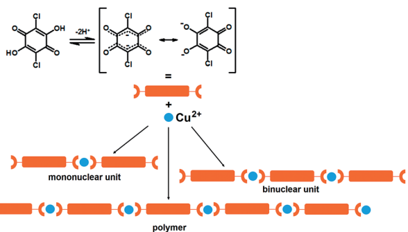
Scheme 1 Dissociation of chloranilic acid and schematic representation of its binding to copper(II) ions investigated in this work.
