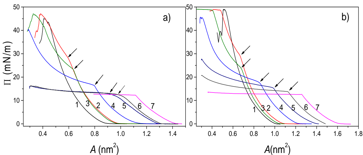
Figure 1: Surface pressure–area per molecule ( \pi - A ) isotherms of the investigated pure and mixed POPC/TO layers assembled on a water (a) and 0.55 M NaCl subphase (b). Curves 1-7 represent
