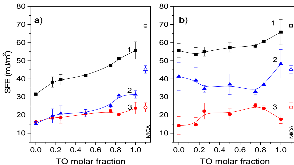
Figure 5: The total surface free energy (curves 1), and its respective polar (curves 2) and disperse (curves 3) components of pure and mixed POPC/TO monolayers, formed on a water (a) and on 0.55 M NaCl (b) subphase and transferred onto the mica substrate, presented as functions of the TO molar fraction. The symbols represent average measured values, lines the corresponding B-spline fit. Error bars represent the corresponding standard deviations. Values of SFE for pure mica (open symbols) are presented at right side of the panels.
