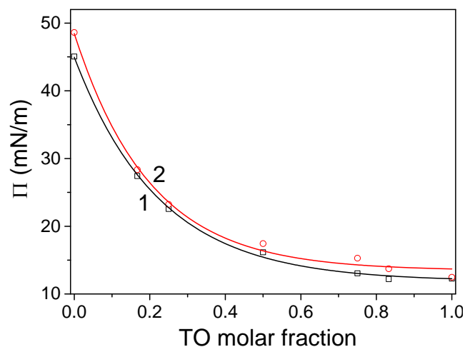
Figure 2: The envelope points of mixed monolayers assembled on water (1) and (2) electrolyte subphase. Symbols represent experimental values and line the corresponding fit with an exponential function. R^2 (water) = 0.9990, R^2 (electrolyte) = 0.9947. The corresponding error bars, i.e. the standard deviations fall within the size of the symbols (~2%).
