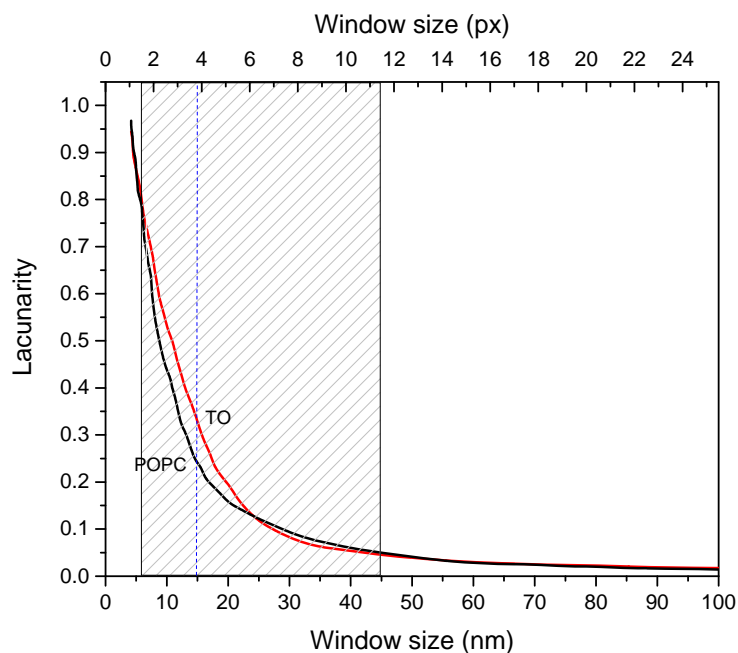
Figure 4: Lacunarity vs. window (scale) size for pure POPC and TO layers assembled at NaCl subphase. Shaded area corresponds to the scale range in which lacunarity of POPC and TO layers are different. Dashed line denotes scale corresponding to the highest difference in lacunarity.
