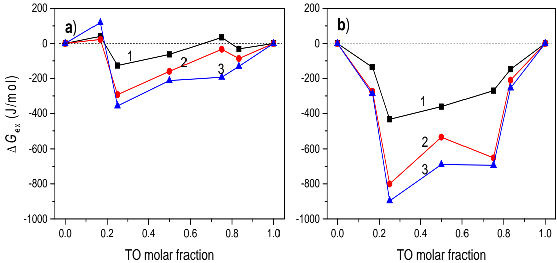
Figure 3: The excess Gibbs energy of mixing of POPC/TO assemble on the water (a) and on 0.55 M NaCl (b) subphases at surface pressures 5, 10 and 12.5 mN/m (curves 1-3, respectively).
