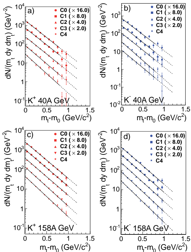
FIG. 1. (Color online) Transverse mass spectra at mid-rapidity from the combined dE/dx and TOF analysis for K^+ and K^- in Pb+Pb collisions at 40A GeV ( -0.1 < y < 0.1 ) and 158A GeV ( -0.2 < y < 0.2 ) beam energy. Lines show exponential fits for 0.0 \text{ GeV}/c^2 < m_T - m_0 < 0.8 \text{ GeV}/c^2 (40A GeV) and 0.0 \text{ GeV}/c^2 < m_T - m_0 < 1.0 \text{ GeV}/c^2 (158A GeV). Different centralities are scaled for clarity. The error bars indicate the statistical uncertainty.
