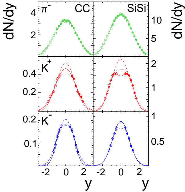
FIG. 8. (Color online) Rapidity spectra for \pi^- and K^\pm for semi-central C+C and Si+Si collisions at 40A GeV beam energy. Solid lines show free fits of double Gaussians. Open symbols are reflected at mid-rapidity. For K^\pm also double Gaussians with width \sigma and shift y_0 as for central Pb+Pb collisions at 40A GeV beam energy were fitted (short dashed line) as well as a single Gaussian with the same RMS_y (dashed line). The error bars indicate the statistical uncertainty.
