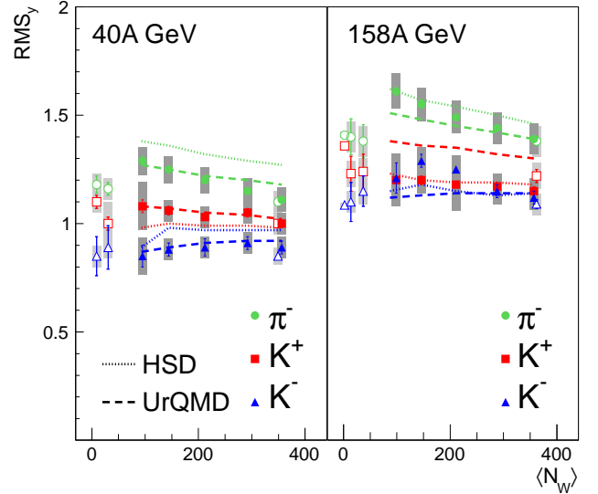
FIG. 9. (Color online) Width of the rapidity distribution described by the RMS values for \pi^- , K^+ and K^- versus mean number of participating nucleons. Open symbols show results from p+p, C+C, Si+Si and central Pb+Pb collisions. Except for the new results for C+C and Si+Si collisions at 40A GeV beam energy the data are taken from [2, 3, 8, 9]. Filled symbols represent the centrality selected Pb+Pb data. Lines show results from HSD [36] and UrQMD2.3 [37] simulations as indicated in the figure. The thin vertical bars indicate the statistical errors, which are mostly not visible. The thick shaded bars indicate the systematic errors.
