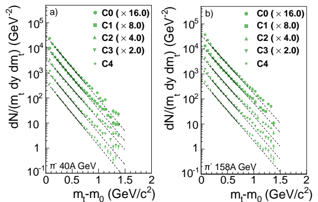
FIG. 2. (Color online) Transverse mass spectra at mid-rapidity ( 0 < y < 0.2 ) for \pi^- in Pb+Pb collisions at 40A GeV and 158A GeV beam energy. Lines show exponential fits for 0.2 \text{ GeV}/c^2 < m_T - m_0 < 0.7 \text{ GeV}/c^2 . Different centralities are scaled for clarity. The error bars indicate the statistical uncertainty.
