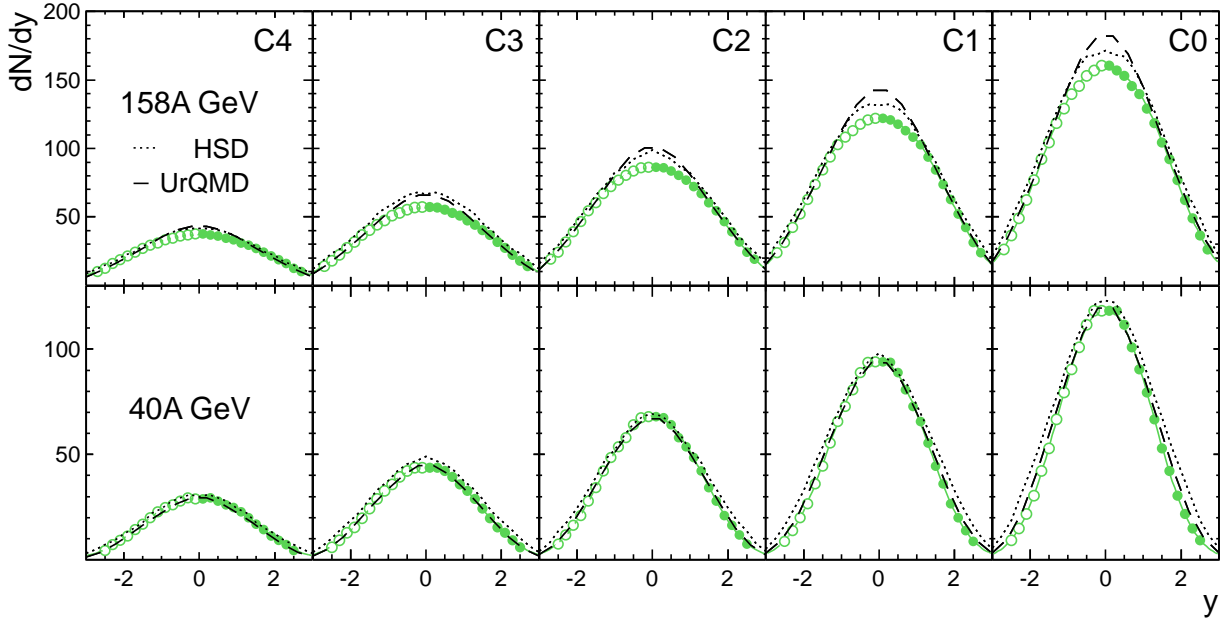
FIG. 5. (Color online) Rapidity spectra for \pi^- in Pb+Pb collisions at 40A GeV and 158A GeV beam energy for different centrality bins labelled C0-C4. Open symbols are reflected at mid-rapidity. Solid lines represent the fits of Eq. 2 (often not visible due to symbol size). The dotted and dashed lines represent HSD [36] and UrQMD2.3 [37] simulations, respectively. The error bars (mostly not visible) indicate the statistical uncertainty.
