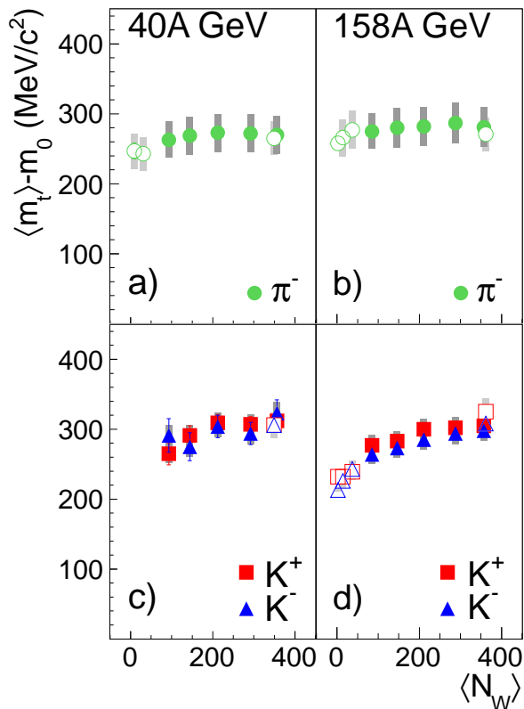
FIG. 4. (Color online) Mean transverse mass as extracted from the transverse mass spectra at mid-rapidity for \pi^- , K^+ and K^- versus number of participating nucleons. Open symbols show results from p+p, C+C, Si+Si and central Pb+Pb collisions. Except for the new results for C+C and Si+Si collisions at 40A GeV beam energy the data are taken from [2, 3, 8–10]. Filled symbols represent the centrality selected Pb+Pb data. The thin vertical bars indicate the statistical errors, which are mostly not visible. The thick shaded bars indicate the systematic errors.
