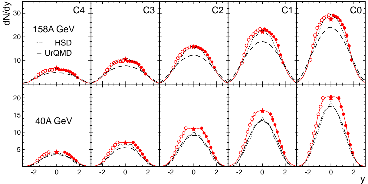
FIG. 6. (Color online) Rapidity spectra of K^+ in Pb+Pb collisions at 40A GeV and 158A GeV beam energy for different centrality bins labelled C0-C4. Circles are values from the dE/dx analysis, the stars give the result from the combined dE/dx and TOF analyses. Open symbols are reflected at mid-rapidity. Solid lines represent the fits of Eq. 2 (often not visible due to symbol size). The dotted and dashed lines represent HSD [36] and UrQMD2.3 [37] simulations, respectively. The error bars (mostly not visible) indicate the statistical uncertainty.
