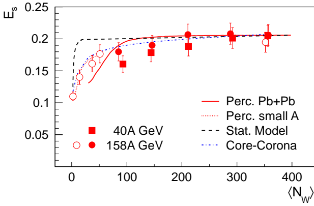
FIG. 14. (Color online) Total relative strangeness approximated by E_S for centrality selected minimum bias Pb+Pb collisions at 40A GeV (squares) and 158A GeV (circles) as function of \langle N_w \rangle . The open symbols are from p+p [9, 10], C+C, Si+Si [2], S+S [40] and central Pb+Pb [2] at 158A GeV. The filled symbols represent the data of centrality selected Pb+Pb collisions at 40A GeV and 158A GeV (this analysis and [6]). The lines indicate calculations within the statistical model assuming proportionality between ensemble volume and \langle N_w \rangle (dashed), with volumes as derived from percolation calculations for small systems (dotted line) and Pb+Pb collisions (solid line) [21], as well as calculations based on the core-corona ansatz at 158A GeV (dash-dotted line). Only statistical errors are shown.
