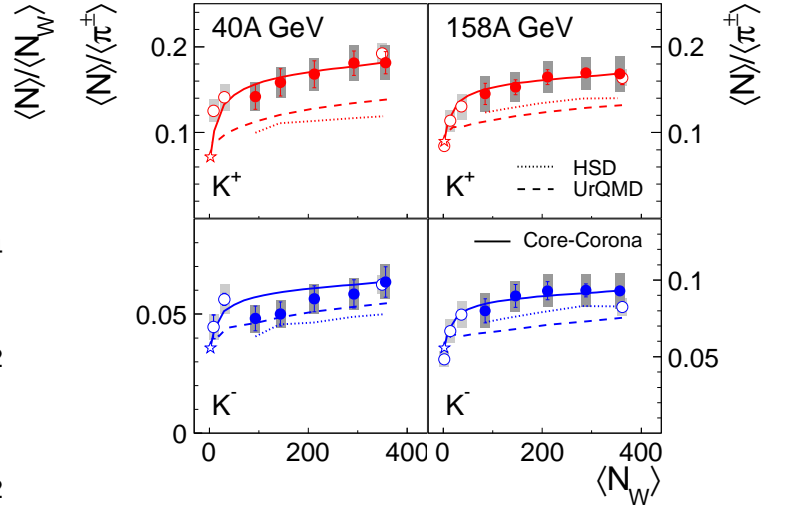
FIG. 11. (Color online) Kaon yields divided by mean number of pions \langle \pi^\pm \rangle = 0.5 \cdot (\langle \pi^- \rangle + \langle \pi^+ \rangle) as a function of centrality. Closed symbols show results from centrality selected Pb+Pb collisions, open symbols p+p data from NA49 [9, 10] as well as C+C, Si+Si (at 158A GeV [8]) and central Pb+Pb collisions from [2, 3]). The stars denote the values obtained from the parametrization "B" in reference [38]. Lines show results from HSD [36] and UrQMD2.3 [37] simulations and the core-corona model (the latter for the Pb+Pb collision system only, [39]). The thin vertical bars indicate the statistical errors, which are mostly not visible. The thick shaded bars indicate the systematic errors.
