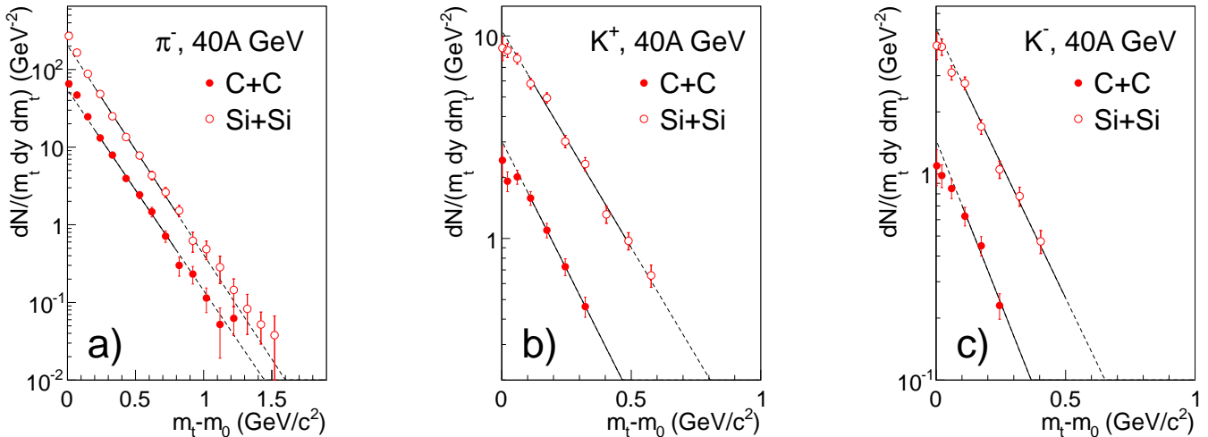
FIG. 3. (Color online) Transverse mass spectra of \pi^- ( 0 < y < 0.2 ) and kaons ( 0.8 < y < 1.0 ) at 40A GeV in C+C and Si+Si collisions. Lines show exponential fits for 0.2 \text{ GeV}/c^2 < m_T - m_0 < 0.8 \text{ GeV}/c^2 ( \pi^- ) and 0.1 \text{ GeV}/c^2 < m_T - m_0 < 0.5 \text{ GeV}/c^2 (kaons). The inverse slope parameters for K^+ ( K^- ) are 171 \pm 18 \text{ MeV} for C+C and 203 \pm 10 \text{ MeV} for Si+Si collisions ( 137 \pm 24 \text{ MeV} for C+C and 166 \pm 13 \text{ MeV} for Si+Si collisions). The inverse slopes of pions are given in Table IV. The error bars indicate the statistical uncertainty.
