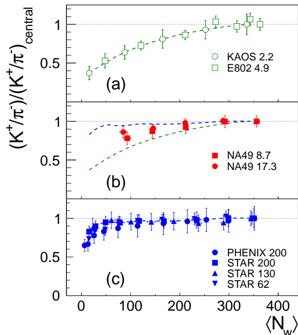
FIG. 13. (Color online) Centrality dependence of the double ratio of the K^+ to \pi^- multiplicities scaled to the ratios from the corresponding most central measurement minimum bias Pb+Pb (Au+Au) collisions at SIS [11] and AGS [12, 13] energies (a), at SPS energies (b) and at RHIC energies [14, 15] (c). The dashed lines in panels (a) and (c) are meant to guide the eye and are also drawn as a reference in panel (b). Only statistical errors are shown.
