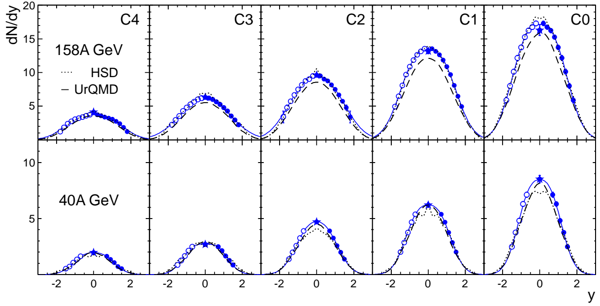
FIG. 7. (Color online) Rapidity spectra of K^- in Pb+Pb collisions at 40A GeV and 158A GeV beam energy for different centrality selections labelled C0-C4. Circles are values from the dE/dx analysis, the star gives the result from the combined dE/dx and TOF analysis. Open symbols are reflected at mid-rapidity. Solid lines represent the fits of Eq. 2. The dotted and dashed lines represent HSD [36] and UrQMD2.3 [37] simulations, respectively. The error bars (mostly not visible) indicate the statistical uncertainty..
