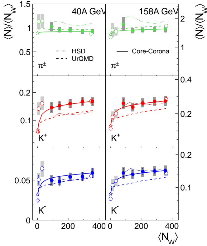
FIG. 10. (Color online) Particle yields divided by the mean number of wounded nucleons as a function of centrality. Closed symbols show results from centrality selected Pb+Pb collisions, open circles p+p data from NA49 [9, 10] as well as C+C, Si+Si (at 158A GeV [8]) and central Pb+Pb collisions from [2, 3]). The stars denote the values obtained from the parametrization "B" in reference [38]. At 40 GeV/c the yields of K^\pm in p+p are compared to values extracted from Fig. 132 reported in [10] (open crosses). Lines show results from HSD [36] and UrQMD2.3 [37] calculations as well as from the core-corona model (the latter for the Pb+Pb collision system only [39]). The thin vertical bars indicate the statistical errors, which are mostly not visible. The thick shaded bars indicate the systematic errors.
