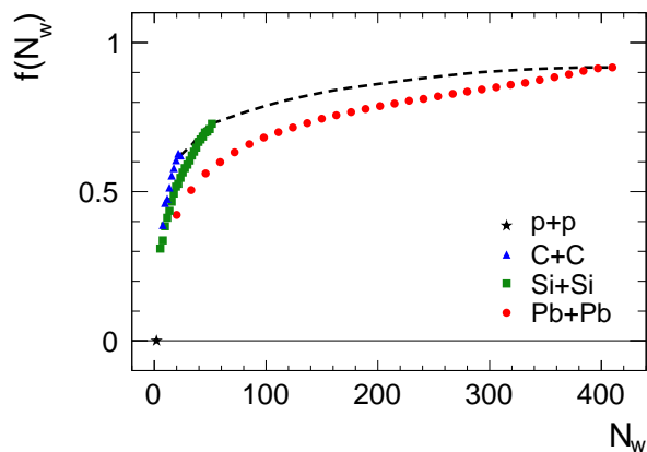
FIG. 12. (Color online) Core fraction obtained in the core-corona model for different collision systems as function of the number of participating nucleons [39]. The dashed line connects the endpoints of the curves for the different collision systems. f(\langle N_w \rangle) denotes the fraction of those nucleons, which undergo more than one collision.
