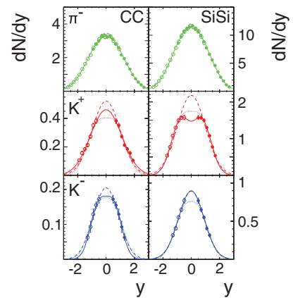
FIG. 8. (Color online) Rapidity spectra for \pi^- and K^\pm for semicentral C + C and Si + Si collisions at 40A GeV beam energy. Solid lines show free fits of double Gaussians. Open symbols are reflected at mid-rapidity. For K^\pm also double Gaussians with width \sigma and shift y_0 as for central Pb + Pb collisions at 40A GeV beam energy were fitted (short dashed line) as well as a single Gaussian with the same RM_{S_y} (dashed line). The error bars indicate the statistical uncertainty.
