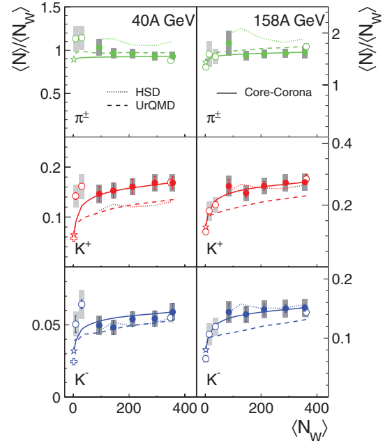
FIG. 10. (Color online) Particle yields divided by the mean number of wounded nucleons as a function of centrality. Closed symbols show results from centrality selected Pb + Pb collisions; open circles show p + p data from NA49 [9,10] as well as C + C , Si + Si (at 158A GeV [8]), and central Pb + Pb collisions from [2,3]. The stars denote the values obtained for p + p interactions from parametrization “B” in Ref. [38]. At 40 GeV/c the yields of K^\pm in p + p are compared to values extracted from Fig. 132 reported in [10] (open crosses). Lines show results from HSD [36] and UrQMD2.3 [37] calculations as well as from the core-corona model (the latter for the Pb + Pb collision system only [39]). The thin vertical bars indicate the statistical errors, which are mostly not visible. The thick shaded bars indicate the systematic errors.
