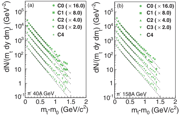
FIG. 2. (Color online) Transverse mass spectra at mid-rapidity ( 0 < y < 0.2 ) for \pi^- in Pb + Pb collisions at 40A GeV and 158A GeV beam energy. Lines show exponential fits for 0.2 < m_T - m_0 < 0.7 GeV/ c^2 . Different centralities are scaled for clarity. The error bars indicate the statistical uncertainty.
