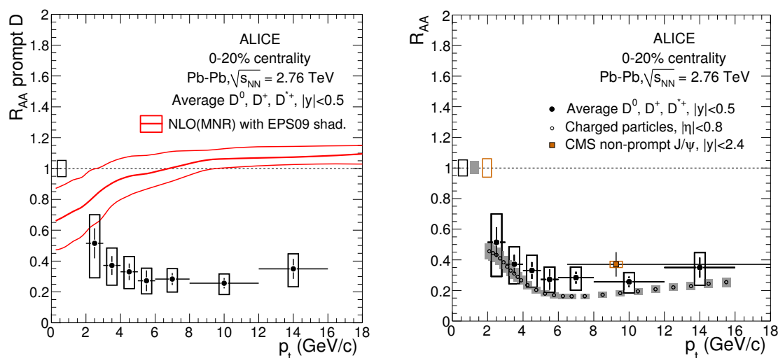
Figure 8. Average R_{AA} of D mesons in the 0–20% centrality class compared to: left, the expectation from NLO pQCD [59] with nuclear shadowing [61]; right, the nuclear modification factors of charged particles [26] and non-prompt J/\psi from B decays [33] in the same centrality class. The charged particle R_{AA} is shown only for 2 < p_t < 16 GeV/c. The three normalization uncertainties shown in the right-hand panel are almost fully correlated.
