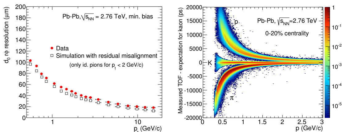
Figure 1. Left: track impact parameter resolution in the transverse plane as a function of p_t in Pb-Pb collisions. For p_t < 2 \text{GeV}/c , pion identification by the TPC or TOF detectors is required; the results for data and simulation are shown. The simulation includes the effect of the residual geometrical misalignment of the sensor modules of the Inner Tracking System (see text for details). Right (colour online): difference between the measured time-of-flight and that expected under the kaon hypothesis as a function of track momentum for the 20% most central Pb-Pb collisions.
