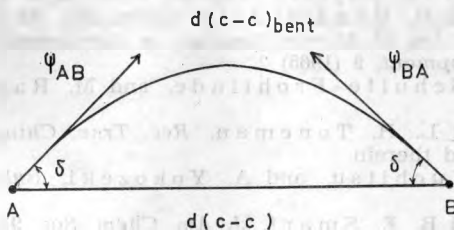
Fig. 1. Schematic Presentation of the Bent Bond.
