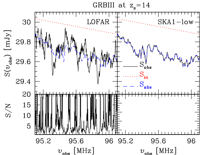
Figure 3. As Figure 1, but the GRBIII is positioned at z_s = 14 (i.e. \nu \sim 95 MHz) and \Delta\nu = 20 kHz. Note that the S/N in the lower right panel is always higher than the range covered by the axis.
