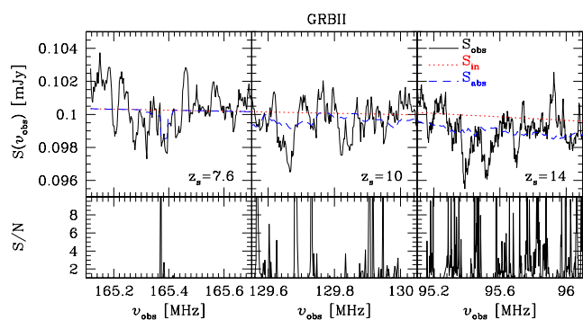
Figure 4. Upper panels: Spectrum of a GRBII with a flux density S_{in}(z_s) = 0.1 mJy. The red dotted lines refer to the intrinsic spectrum of the source, S_{in} ; the blue dashed lines to the simulated spectrum for 21 cm absorption, S_{abs} ; and the black solid lines to the spectrum for 21 cm absorption as it would be seen after an integration time t_{int} = 1000 h with a noise 0.01 \sigma_n (i.e. 1/10th of the SKA1-low noise). The panels refer to a case with z_s = 7.6 and \Delta\nu = 5 kHz (left), z_s = 10 and \Delta\nu = 10 kHz (middle), z_s = 14 and \Delta\nu = 20 kHz (right). Lower panels: S/N corresponding to the upper panels. See text for further details.
