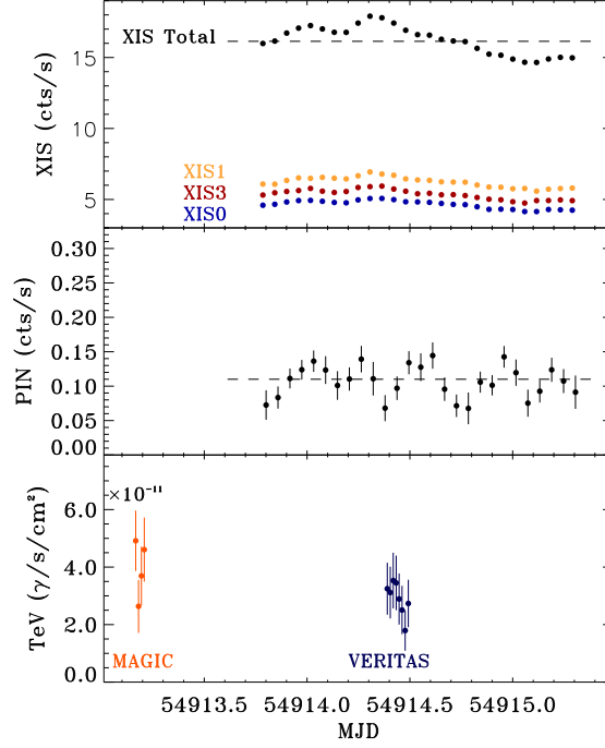
Fig. 2.— Light curves of Mrk 501 in the energy ranges used for Suzaku/XIS ( 0.6 \text{ keV} < E < 10.0 \text{ keV} ), Suzaku/HXD ( 10 \text{ keV} < E < 70 \text{ keV} ), MAGIC and VERITAS ( E > 300 \text{ GeV} ). Error bars show 1\sigma statistical errors. The constant fits to the Suzaku data are shown. See discussion in Sec. 3.1. A color version of this figure is available online.
