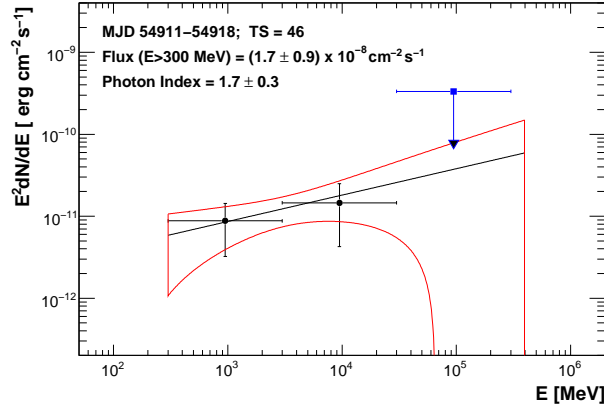
Fig. 4.— Plot of the Fermi spectral results for the 7 days centered on the Suzaku observing time window (MJD 54911 – MJD 54918). The solid line depicts the result of the unbinned likelihood power-law fit, and the contour shows the 68% uncertainty of the fit. The data points show the energy fluxes computed in differential energy ranges, with a 95% confidence level upper limit for the highest energy range. The Fermi analysis was performed in the energy range 0.3-400 GeV. The vertical bars show 1\sigma statistical errors, and the horizontal bars show the energy range for each point. A color version of this figure is available online.
