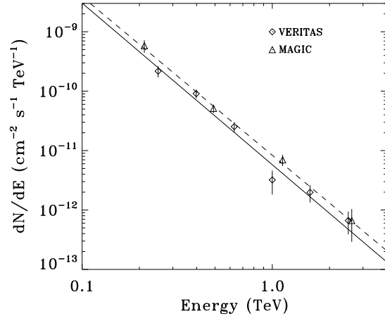
Fig. 5.— VHE spectrum from VERITAS (diamonds) and MAGIC (triangles), including the best-fit power-law models. The VERITAS fit is shown with a solid line, and the MAGIC fit is shown with a dashed line. The slopes of the power-law models agree well ( \Gamma_{VERITAS} = 2.72 \pm 0.15_{stat} \pm 0.10_{sys} and \Gamma_{MAGIC} = 2.67 \pm 0.21_{stat} \pm 0.20_{sys} ). The slight normalization offset corresponds to the moderately higher VHE flux levels during the MAGIC observation. The vertical bars show 1\sigma statistical errors.
