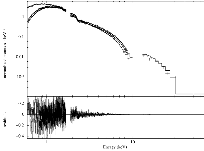
Fig. 3.— Observed X-ray spectra of Mrk 501 made from Suzaku XIS and HXD/PIN data separately. A joint fit to a broken power-law model was performed for the three XIS CCDs and the HXD/PIN. The solid histogram shows the best fits to the data (see Sec. 3.2). The error bars represent 1\sigma statistical errors. The bottom panel shows the residuals of the fit.
