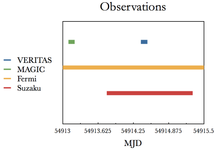
Fig. 1.— Overall time coverage of Mrk 501 by the instruments involved in the multiwavelength campaign. Gaps due to orbital constraints are not indicated in the Fermi and Suzaku plots. A color version of this figure is available online.
