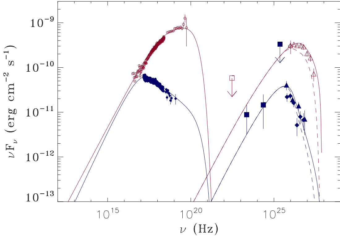
Fig. 6.— Spectral energy distributions of Mrk 501 in the quiescent state (in filled points) and during the 1997 extreme outburst (in open points). The former is made from data obtained in the present campaign with Suzaku (filled circles), Fermi (filled squares), VERITAS (filled diamonds), and MAGIC (filled triangles). The latter was taken from Pian et al. (1998) and Djannati-Ataï et al. (1999), with X-ray data from BeppoSAX (open circles), GeV \gamma -ray upper limit from EGRET (open square), and VHE \gamma -ray data from the Whipple 10m (open diamond) and the CAT Cerenkov telescope (open triangles). Note that the Whipple 10m spectral point overlaps with the lowest-energy CAT spectral point. The vertical bars for all data show 1\sigma statistical errors and the upper limits are at the 95% confidence level. Corresponding SED models matched to the data for each year are shown. The solid lines show the SSC match; dashed lines take EBL absorption into account. The VHE data points are not EBL-corrected. A color version of this figure is available online.
