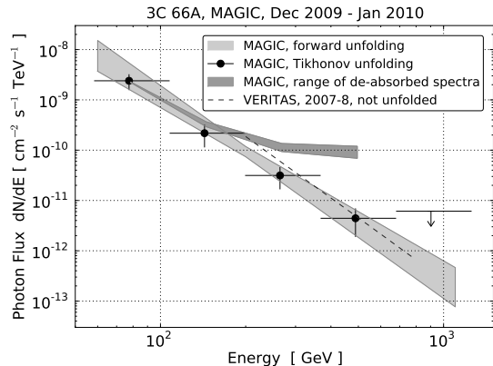
FIG. 3.— Observed and EBL-corrected (de-absorbed) differential energy spectra of 3C 66A in the period of 2009 December and 2010 January. The light-shaded area indicates the 1\sigma range of the observed power law spectrum gained by forward unfolding (see the text), the crosses are from the unfolding after Tikhonov & Arsenin (1979) for comparison. The dark-shaded area is the spread of the de-absorbed, mean flux values obtained by the four applied EBL models, assuming the redshift of z=0.444 . The VERITAS (observed) spectrum after Acciari et al. (2009) is shown for comparison.
