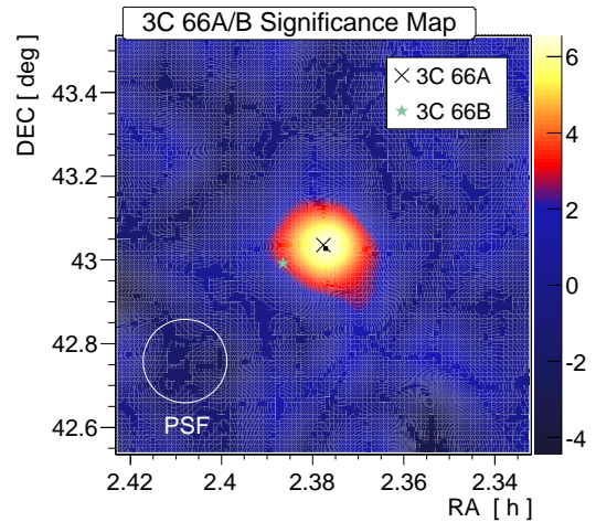
FIG. 1.— MAGIC significance skymap of the region around 3C 66A/B for events with energies above 100 GeV.
