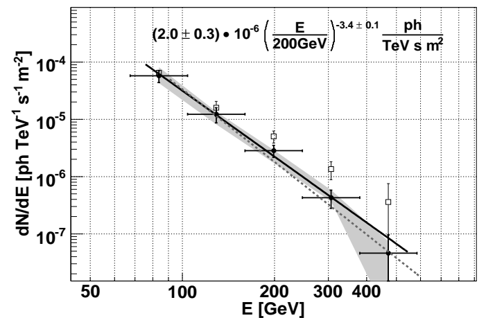
Fig. 1. MAGIC measured spectrum of PG 1553+113 (filled circles). The statistical significance of the points from left to right are 2.7, 4.2, 3.4, 4.3, and 3.0\sigma respectively. The EBL-corrected points are shown as empty squares. The spectrum obtained during our first observation is shown as a dashed line.
