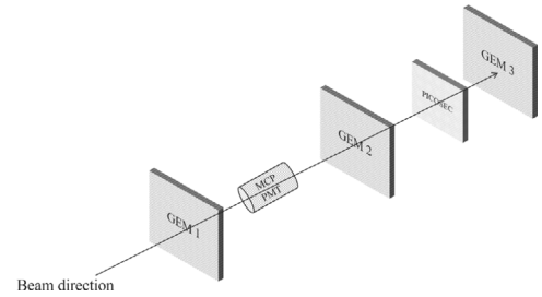
Fig. 2. Schematic of the experimental setup for time response test of the multipad detector to 150 GeV/c muons.
