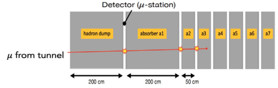
Fig. 1. Schematic of the muon stations and absorbers configuration to be installed at the hadron dump. The gray slabs represent the absorbers (made out of iron or rock) while the white slices, 8 in total, are the muon detector planes, where the PICOSEC-MM detector can be placed [5].
