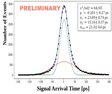
Fig. 3. Signal Arrival Time distribution of the central Pad-0 of the multipad detector, operating in the highest gain of 550 V on the cathode and 275 V on the anode after time walk corrections, resulting in a timing resolution of 21.3 \pm 0.6 ps. This number refers to approximately 11 photoelectrons per muon track.
