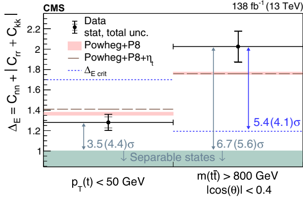
FIG. 29. The observed levels of entanglement characterized by \Delta_E are shown in the threshold region using the D measurement (first bin), and in the high- m(t\bar{t}) region using the full matrix measurement (second bin). The measurements (points) are shown with the statistical uncertainty (inner error bars) and total uncertainty (outer error bars) and compared to the predictions of POWHEG+PYTHIA, POWHEG+PYTHIA+ \eta_t . The POWHEG+PYTHIA prediction is displayed with the ME scale and PDF uncertainties. The horizontal blue lines correspond to the maximum level of entanglement \Delta_{E,\text{crit}} that can be explained by the exchange of information between t and \bar{t} at the speed of light. The significance in standard deviations ( \sigma ) by which the measurement exceeds \Delta_{E,\text{crit}} and unity is quoted in blue and light green, respectively, and indicated by the corresponding arrows.
