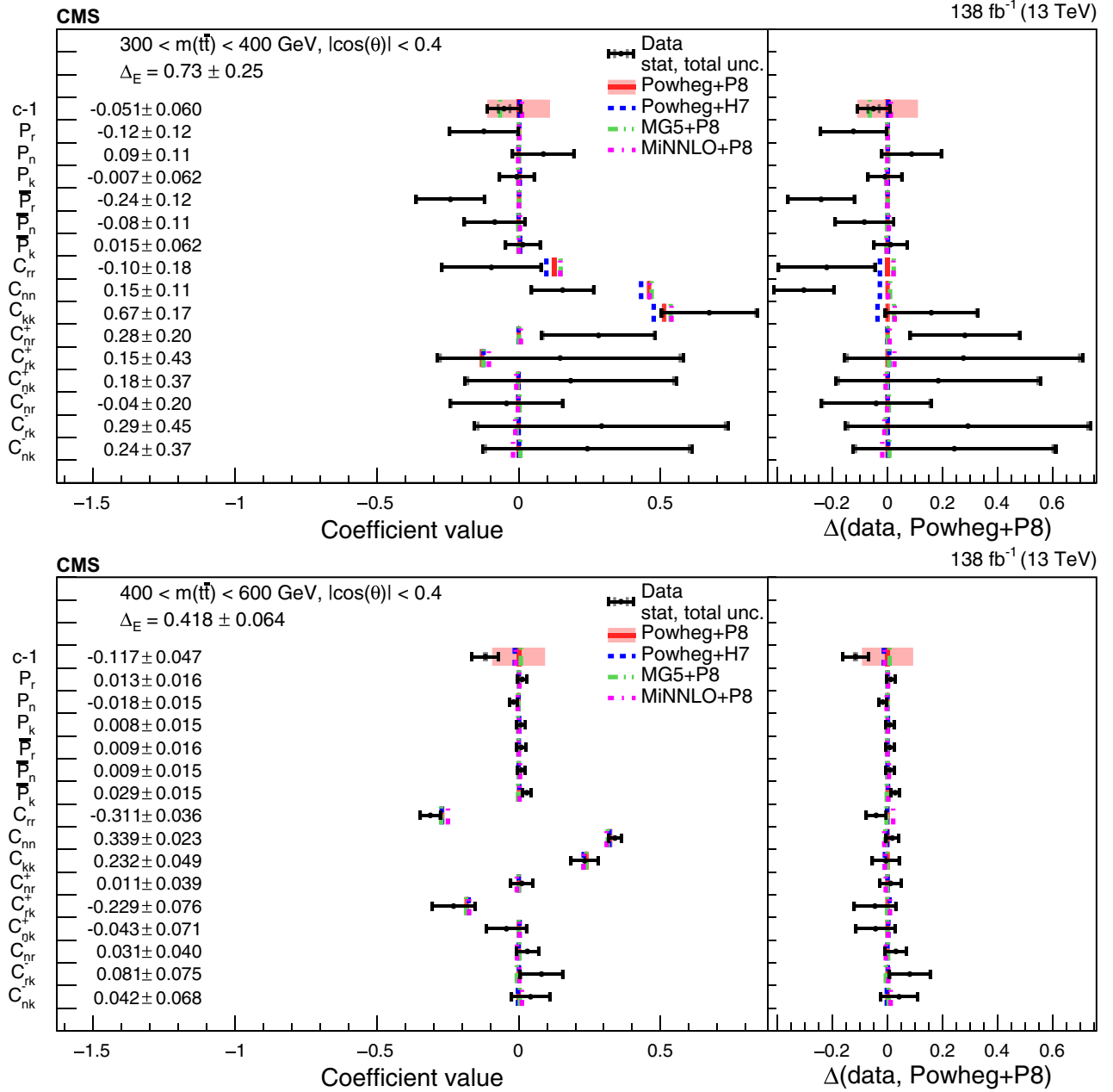
FIG. 25. Results of the full matrix measurement in bins of m(\bar{t}\bar{t}) for |\cos(\theta)| < 0.4 . The measurements (markers) are shown with the statistical uncertainty (inner error bars) and total uncertainty (outer error bars) and compared to the predictions of POWHEG+PYTHIA, POWHEG+Herwig, MadGraph5_aMC@NLO+PYTHIA and MiNNLO+PYTHIA. In the right panels, results are presented with the POWHEG+PYTHIA predictions subtracted. The POWHEG+PYTHIA prediction is displayed with ME scale and PDF uncertainties. The values of \Delta_E are displayed for each measurement.
