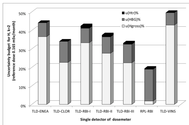
Fig. 3. Uncertainty of H for seven detectors of five passive dosimetry systems* with k = 2 obtained from a simulation of a hypothetical dose of 0.165 mSv/month. For each dosimeter the different colours represent the factors taken into account with their relative contribution in the uncertainty budget analysis. * The three data of TLD-RBI refer to three detectors of a single dosimeter).
