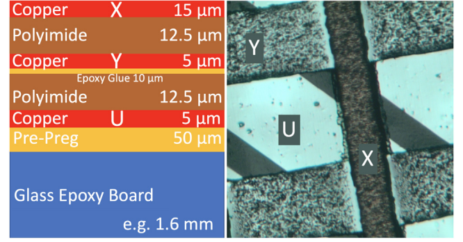
Fig. 4. Schematic cross section and close view of the three overlapping strips.
