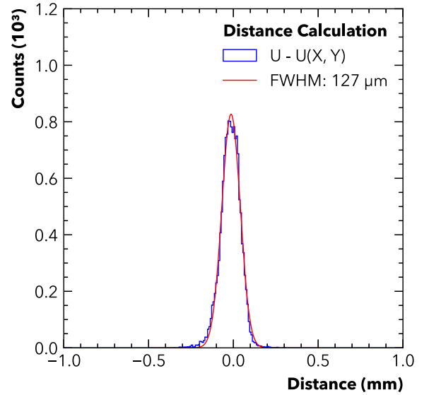
Fig. 8. Computed distance of the U projection from the hits position obtained from the X and Y coordinates, using U(X,Y) = 511 - X - Y , where 511 is the total number of U strips.
