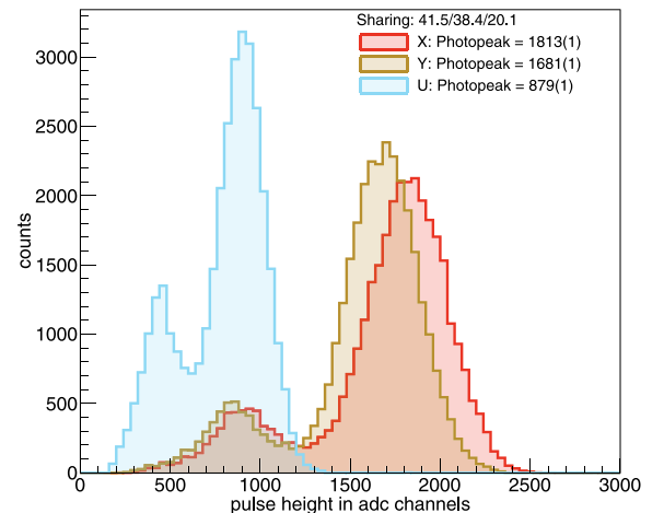
Fig. 5. Pulse height spectra recorded for 5.9 keV X-rays on the X, Y and U projections.
