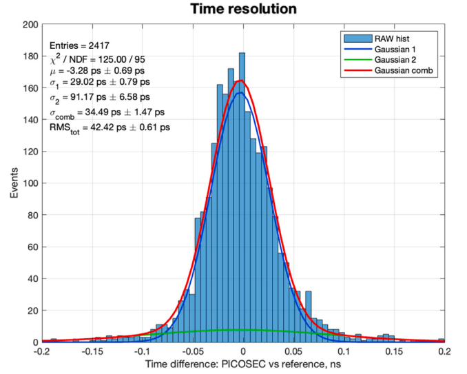
Fig. 11. SAT distribution of a prototype equipped with a 9 nm \text{B}_4\text{C} photocathode. The voltages were at V_C = -490 V on the cathode and V_A = 275 V on the anode. The results show a time resolution of \sigma = 34.5 \pm 1.5 ps.
