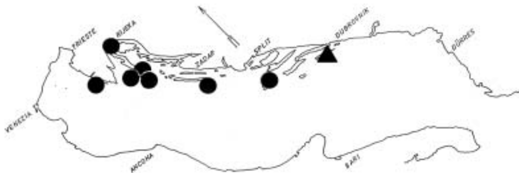
Fig. 20. Records of Ophioconis forbesi in the Adriatic Sea. ● from the literature, ▲ present study
