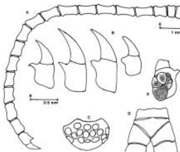
Fig. 2. Antedon mediterranea . A = cirrus; B = terminal claws; C = centro-dorsal plate; D = Ibr2; E = an epizoic foraminiferan settled on a terminal cirrus claw
