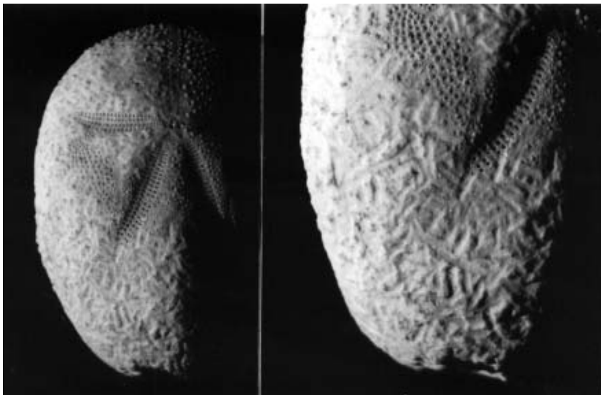
Fig. 27. Brissus unicolor . A scratched test (CMRR 2287, TL 44 mm). Left: Aboral view; Right: A detail
