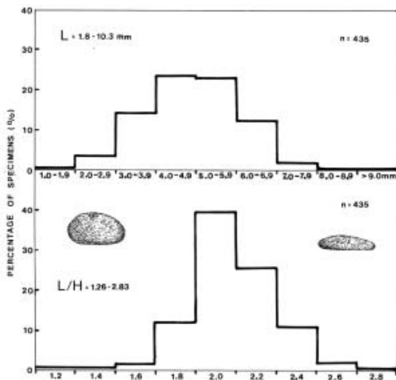
Figure 22. Morphometry of the Echinocyamus pusillus tests
