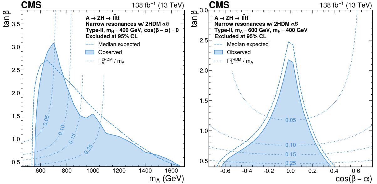
Figure 7: Median expected (dashed lines) and observed (filled contours) 95% CL exclusion regions in the type-II 2HDM (\tan \beta, m_A) parameter space at m_H = 400 GeV (left) and in the (\tan \beta, \cos(\beta - \alpha)) parameter space at m_A = 600 GeV and m_H = 400 GeV (right), derived assuming narrow resonances. The enclosed regions are excluded. The dotted lines indicate points of constant total decay width \Gamma_A of the A boson relative to its mass in the 2HDM.
