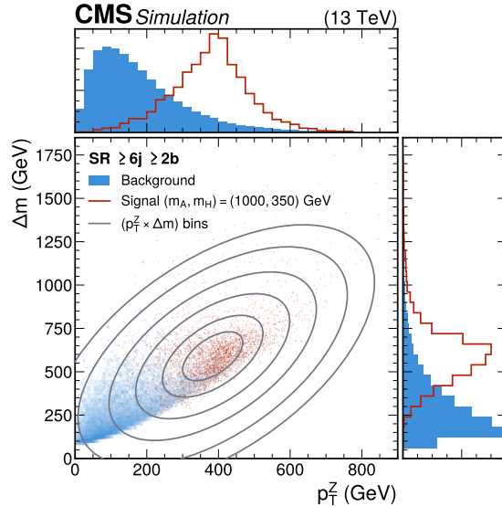
Figure 2: Expected (\Delta m, p_T^Z) distribution for signal events with m_A = 1000 GeV and m_H = 350 GeV (red) and sum of backgrounds (blue) in the \text{SR} \geq 6j \geq 2b category, and boundaries of the elliptical bins (solid lines) used to construct the final observable.
