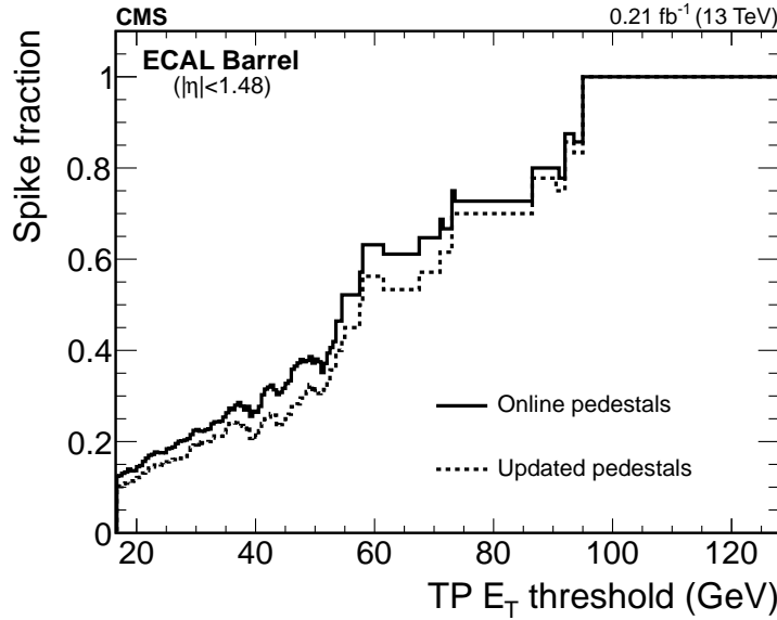
Figure 15. Fraction of ECAL TPs in the barrel region that are matched to an offline spike, as a function of the trigger primitive E_T threshold, before and after updated pedestal values are applied.
