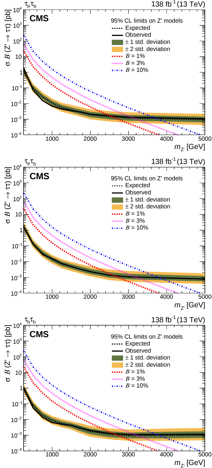
Figure 3: Upper limits at 95% CL on \sigma B(Z' \rightarrow \tau^+\tau^-) for the (upper) \tau_\mu \tau_h , (middle) \tau_e \tau_h , and (lower) \tau_h \tau_h channel. In each plot, the solid black line represents the observed limit, and the black dashed line with green and yellow bands depicts the expected limit with its one- and two-standard deviation uncertainties, respectively. The red dashed, magenta dotted, and blue dash-dotted lines represent the theoretical predictions for B(Z' \rightarrow \tau^+\tau^-) = 1, 3, \text{ and } 10\% , respectively; 3% is the value of B(Z' \rightarrow \tau^+\tau^-) in the SSM. These assume that the B(Z' \rightarrow \tau^+\tau^-) values are fixed for all m_{Z'} .
