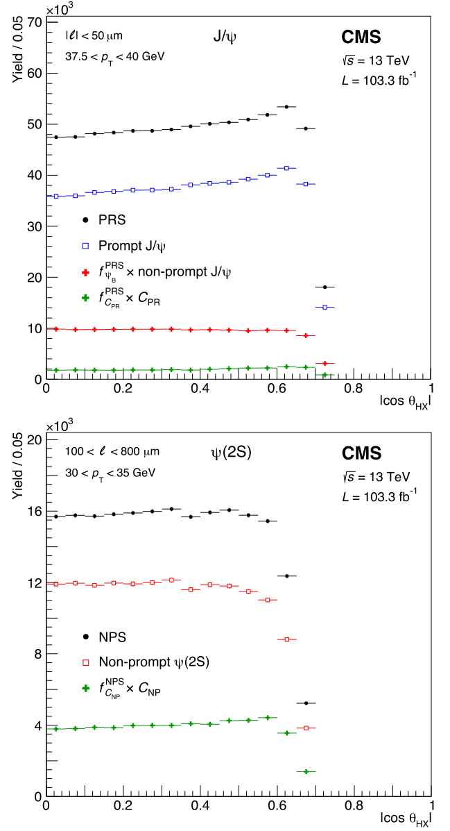
Fig. 10. |\cos \theta_{HX}| distributions measured in the PRS J/\psi (top) and NPS \psi(2S) (bottom) samples, of the terms of Eqs. (4) and (3), respectively, in the mentioned p_T bins.
