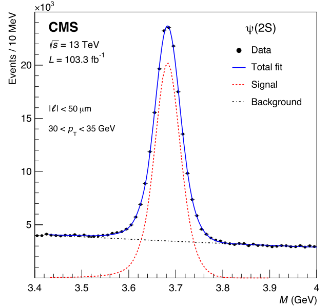
Fig. 4. Dimuon mass distributions measured for the prompt J/\psi (top) and \psi(2S) (bottom) event samples, in the mentioned p_T bins. The total fit function (blue), the sum of the two CB functions and (only in the J/\psi case) the Gaussian function (red), and the background continuum (black) are also shown.
