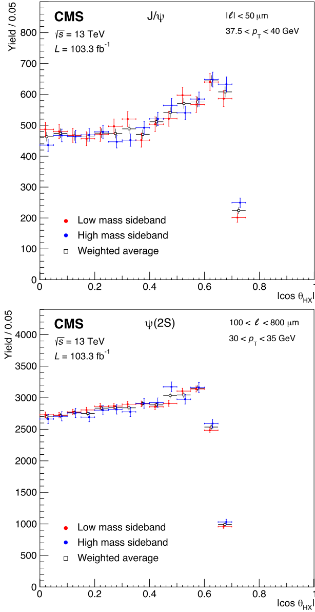
Fig. 9. |\cos \theta_{HX}| distributions measured in the mass sidebands (shifted horizontally for better visibility), and their weighted average, for the prompt J/\psi (top) and non-prompt \psi(2S) (bottom) samples, in the mentioned p_T bins.
