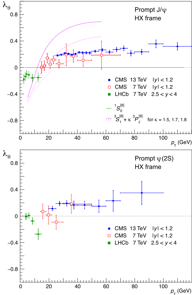
Fig. 13. The \lambda_\theta parameter measured, as a function of p_T , for prompt J/ \psi (top) and \psi(2S) (bottom) mesons, in pp collisions at \sqrt{s} = 13 TeV, compared to measurements made at 7 TeV by CMS [10] and LHCb [11,12]. The vertical bars represent the total uncertainties. The curves on the top panel are described in the text.
