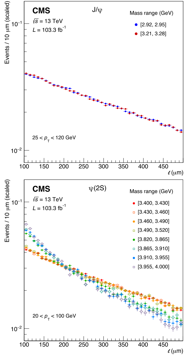
Fig. 6. Dimuon decay length distributions, integrated in p_T , measured for the sideband mass ranges mentioned in the legends, in the J/\psi (top) and \psi(2S) (bottom) cases.
