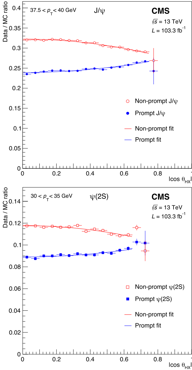
Fig. 11. Ratios between the measured and simulated |\cos \theta_{\text{HX}}| distributions for the prompt and non-prompt J/\psi (top) and \psi(2S) (bottom) events, in the p_T bins mentioned in the legends. The curves represent fits using Eq. (2) and excluding the largest |\cos \theta_{\text{HX}}| bins.
