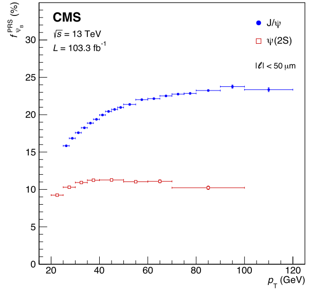
Fig. 8. Variation with p_T of the fraction of events in the PRS region from non-prompt J/\psi and \psi(2S) mesons.
