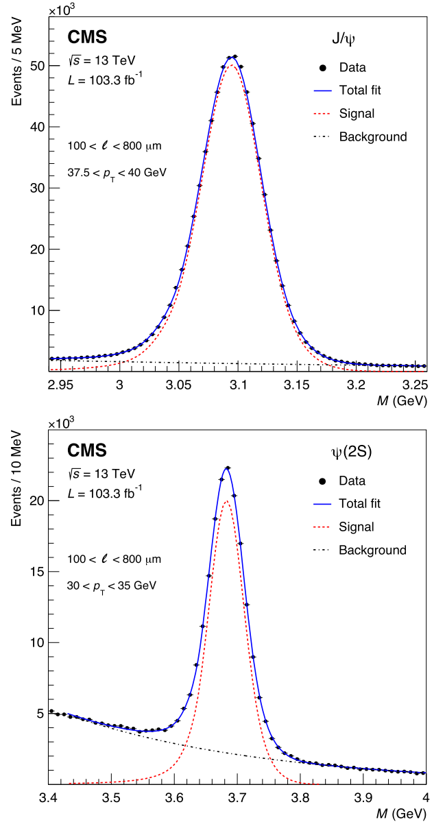
Fig. 2. Dimuon mass distributions measured for the non-prompt J/\psi (top) and \psi(2S) (bottom) event samples, in the mentioned p_T bins. The total fit function (blue), the sum of the two CB functions and, only in the J/\psi case, the Gaussian function (red), and the background continuum (black) are also shown.
