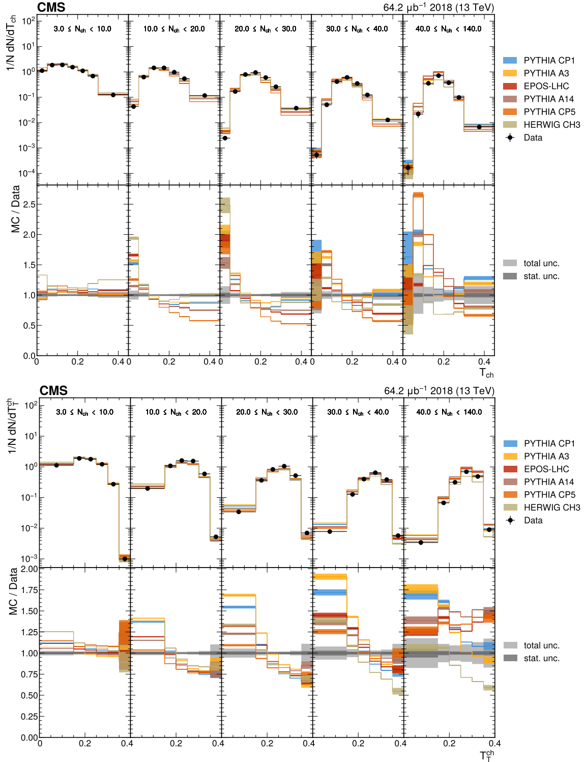
Figure B.2: The unfolded distributions of thrust (upper) and transverse thrust (lower) in slices of charged-particle multiplicity compared with the nominal MC from the PYTHIA CP1 tune and MC predictions from the PYTHIA A14, CP5, A3 tunes, the EPOS-LHC generator, and the HERWIG CH3 tune. The statistical uncertainty on each of the predictions is shown by its shaded band.
