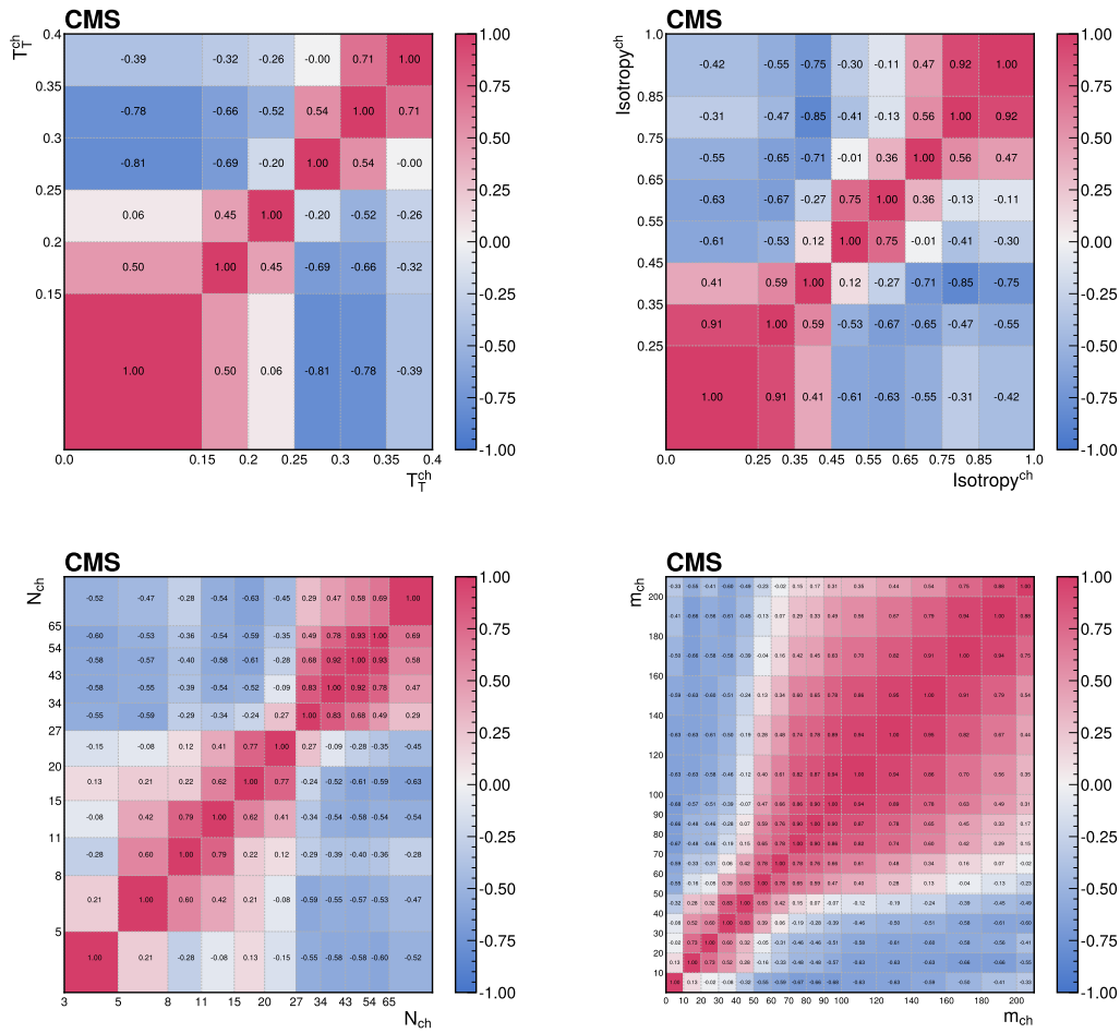
Figure C.2: The correlations of the unfolding systematic uncertainty between bins of the event-shape observables shown for (upper left) transverse thrust, (upper right) isotropy, (lower left) particle multiplicity, and (lower right) invariant mass.
