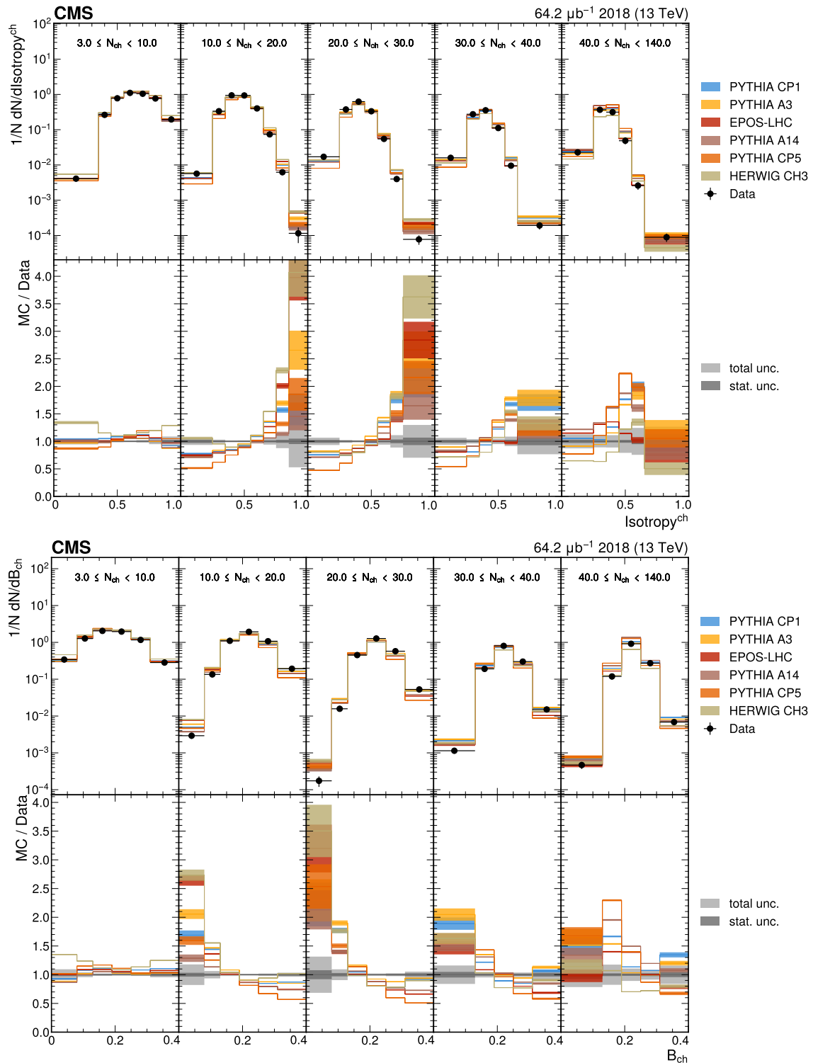
Figure B.1: The unfolded distributions of event isotropy (upper) and broadening (lower) in slices of charged-particle multiplicity compared with the nominal MC from the PYTHIA CP1 tune and MC predictions from the PYTHIA A14, CP5, A3 tunes, the EPOS-LHC generator, and the HERWIG CH3 tune. The statistical uncertainty on each of the predictions is shown by its shaded band.
