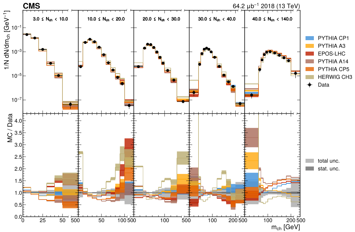
Figure B.3: The unfolded invariant mass of charged particles in slices of charged-particle multiplicity compared with the nominal MC from the PYTHIA CP1 tune and MC predictions from the PYTHIA A14, CP5, A3 tunes, the EPOS-LHC generator, and the HERWIG CH3 tune. The statistical uncertainty on each of the predictions is shown by its shaded band.
