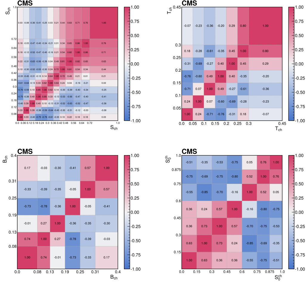
Figure C.1: The correlations of the unfolding systematic uncertainty between bins of the event-shape observables shown for (upper left) sphericity, (upper right) thrust, (lower left) broadening, and (lower right) transverse sphericity.
