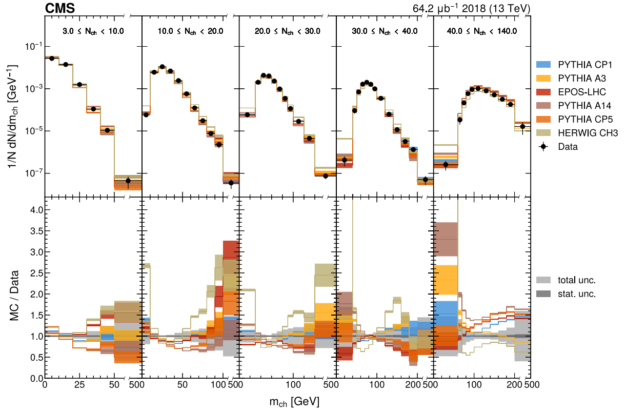
FIG. 7. The unfolded invariant mass of charged particles in slices of charged-particle multiplicity compared with the nominal MC from the PYTHIA CP1 tune and MC predictions from the PYTHIA A14, CP5, A3 tunes, the EPOS-LHC generator, and the HERWIG CH3 tune. The statistical uncertainty on each of the predictions is shown by its shaded band.
