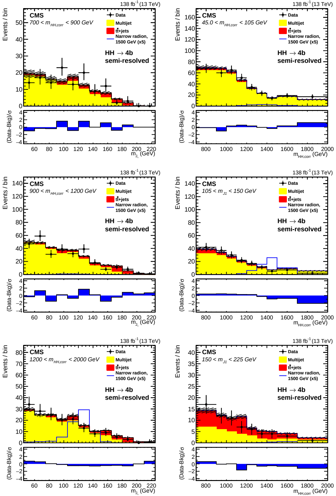
Figure 4: Slices of 2D distributions of observed events and the post-fit templates in the semi-resolved signal region, projected onto the m_{J1} (left) and m_{HH,corr} together with the signal expected for a radion of mass 1.5 TeV. The signal is scaled by the same factor as in Figs. 2 and 3.
