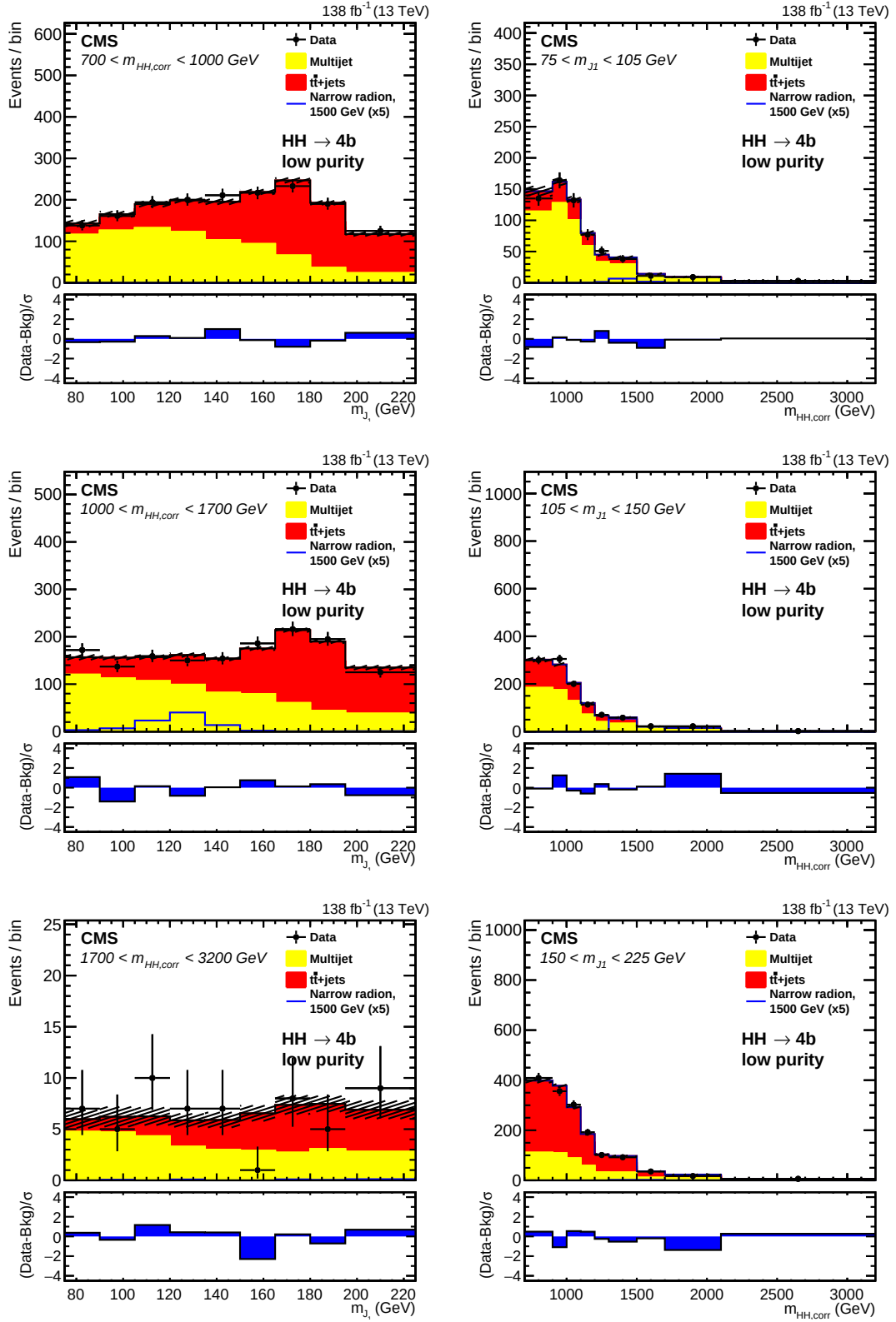
Figure 3: Slices of 2D distributions of observed events and the post-fit templates in the LP signal region, projected onto the m_{j_1} (left) and m_{HH,corr} (right) axes, together with the signal expected for a radion of mass 1.5 TeV. The signal is scaled by the same factor as in Fig. 2.
