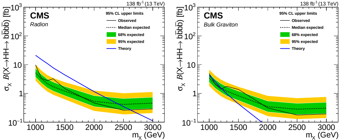
Figure 5: The observed (solid black line) and expected (dashed black line) upper limits at 95% CL on \sigma(\text{pp} \rightarrow X)\mathcal{B}(X \rightarrow \text{HH} \rightarrow b\bar{b}b\bar{b}) for a narrow spin-0 radion (left, corresponding to \Lambda_R = 3 TeV) and a narrow width spin-2 bulk graviton (right, corresponding to k/\bar{M}_{\text{Pl}} = 0.5 ) models. The green (yellow) bands represent one (two) standard deviations from the expected limit. The predicted theoretical cross sections for the narrow radion and bulk graviton are also shown.
