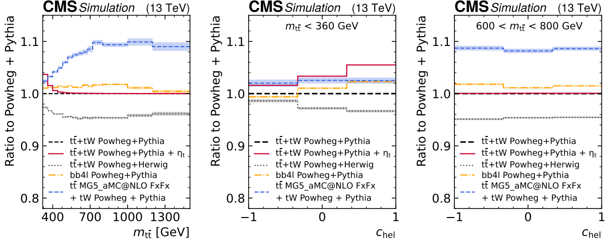
Figure 6: Ratios of the predictions for POWHEG v2 h\nu q +HERWIG (gray), POWHEG vRES bb4l+PYTHIA (orange), and MADGRAPH5_aMC@NLO FxFx+PYTHIA (blue) to POWHEG v2 h\nu q +PYTHIA (black) for m_{t\bar{t}} (left), c_{hel} at the t\bar{t} threshold ( m_{t\bar{t}} < 360 GeV, center), and c_{hel} in the t\bar{t} continuum ( 600 < m_{t\bar{t}} < 800 GeV, right), both integrated over c_{han} . The effect of adding \eta_t to POWHEG v2 h\nu q +PYTHIA is shown in red for comparison. The shaded bands denote the statistical uncertainties from the MC simulation.
