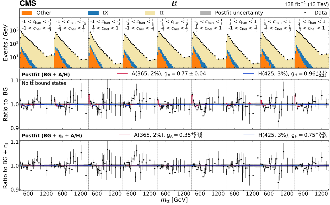
Figure 8: Observed and expected m_{t\bar{t}} distribution in c_{\text{hel}} and c_{\text{han}} bins, shown for the \ell\ell channel summed over lepton flavors and eras. Notations as in Fig. 6.
