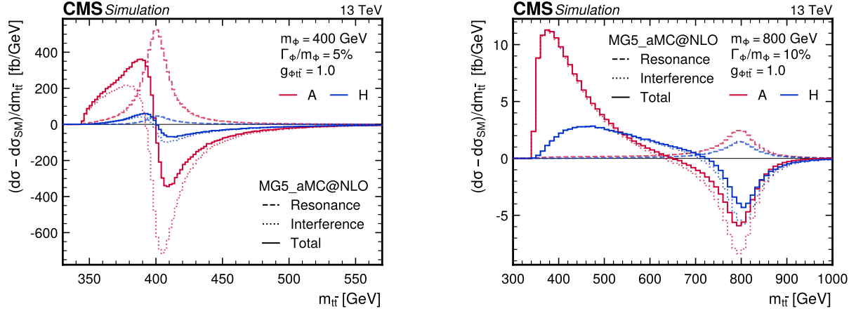
Figure 2: Differential cross section of t\bar{t} production at parton level as a function of m_{t\bar{t}} , shown as difference between various BSM scenarios and the SM prediction. Shown are the cases of a single A (red) or H (blue) boson for two example configurations: m_\Phi = 400 GeV and \Gamma_\Phi/m_\Phi = 5\% (left), or m_\Phi = 800 GeV and \Gamma_\Phi/m_\Phi = 10\% (right), with g_{\Phi t\bar{t}} = 1 in both cases. Separately shown are the cases where only the resonant \Phi \rightarrow t\bar{t} contribution is added to the SM prediction (dashed), where only the interference between SM and \Phi boson contributions is added (dotted), and where both contributions are added (solid). The distributions have been calculated using MADGRAPH5_aMC@NLO as described in Section 3.
