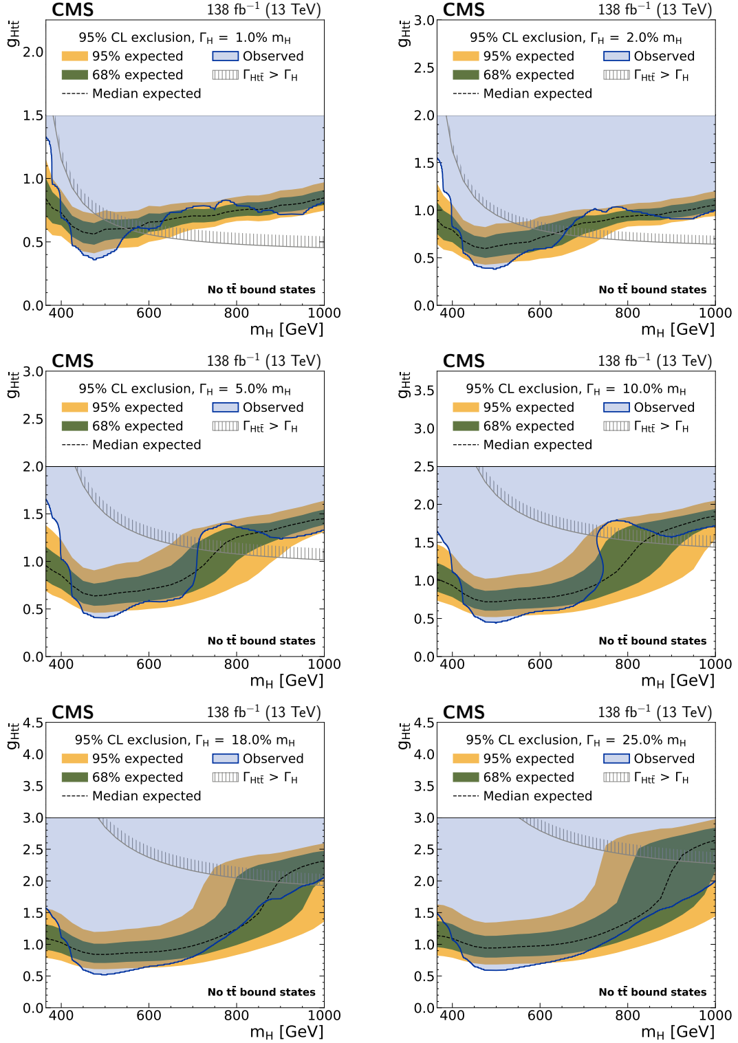
Figure 11: Model-independent constraints on g_{Ht\bar{t}} as functions of the H boson mass in the background scenario without \eta_t contribution, shown in the same fashion as in Fig. 10.
