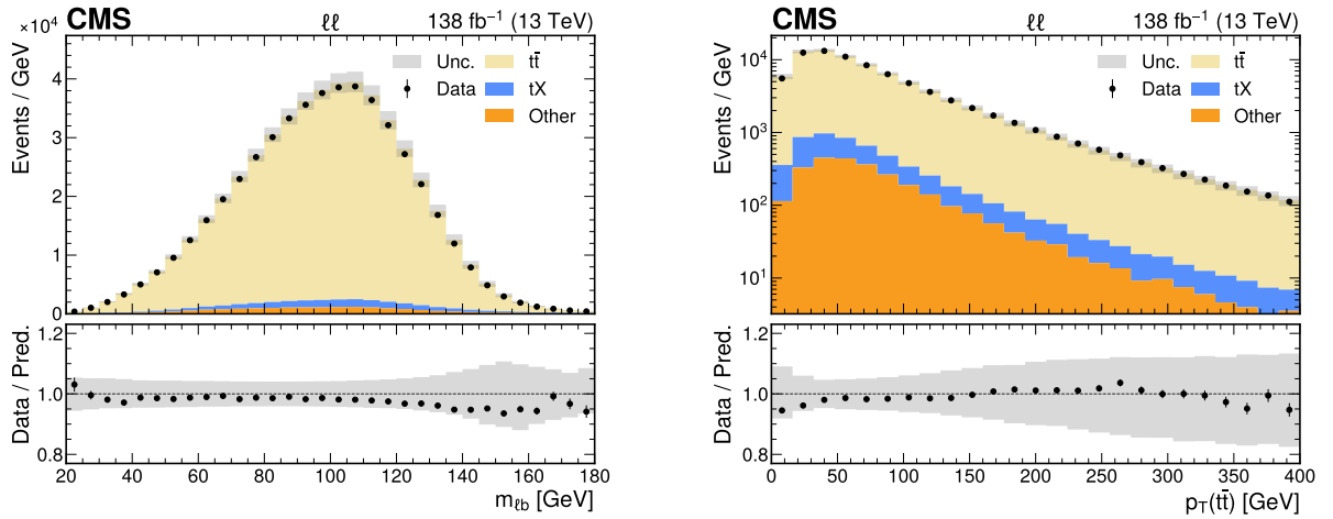
Figure 5: Comparison of the number of observed (points) and expected (colored histograms) events in the \ell\ell channel after the kinematic reconstruction and background estimation for the distributions of the invariant lepton-b jet mass m_{\ell b} (left) and the p_T of the t\bar{t} system (right). The ratio to the total prediction is shown in the lower panel, and the total systematic uncertainty is shown as the gray band.
