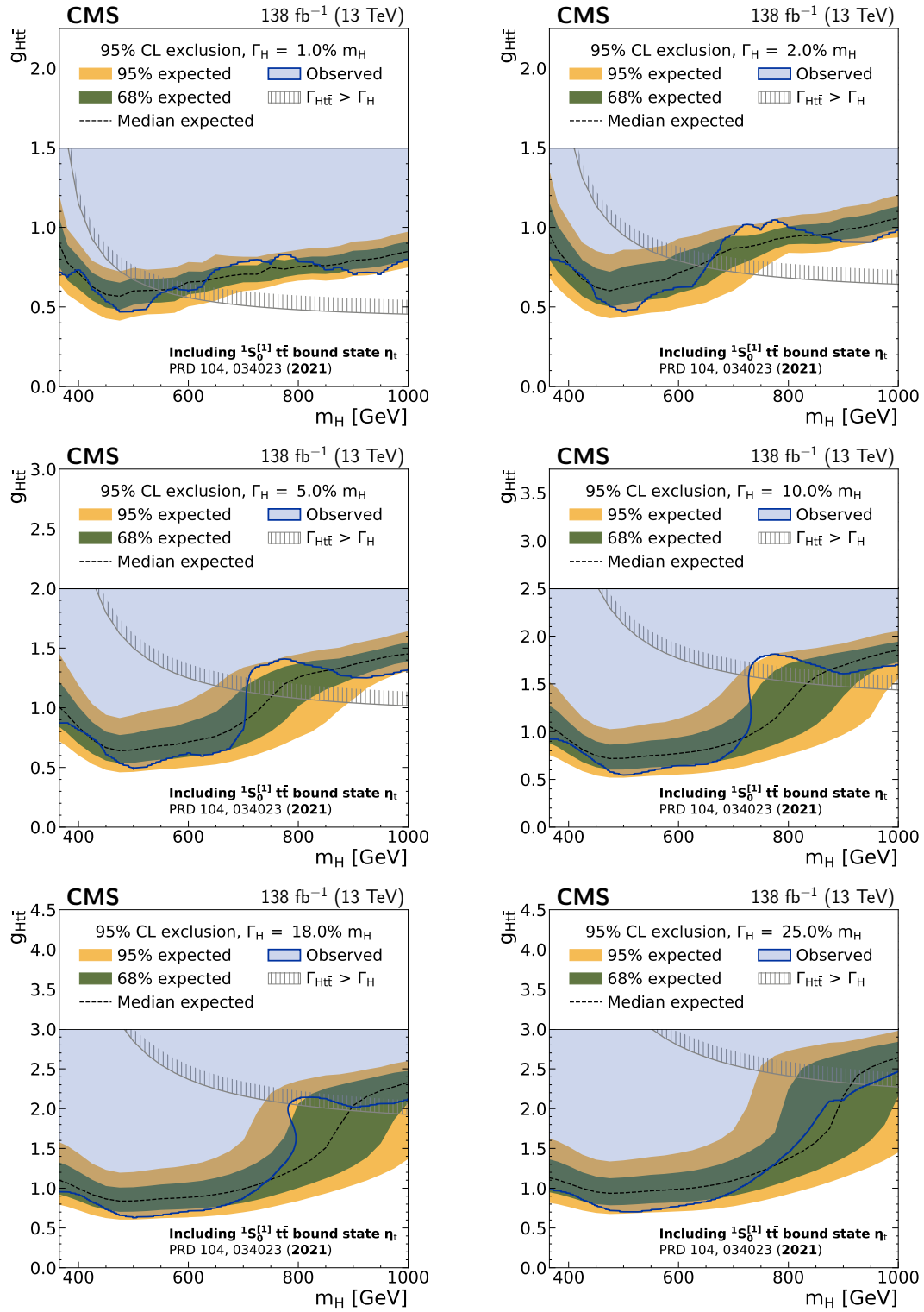
Figure 13: Model-independent constraints on g_{Ht\bar{t}} as functions of the H boson mass in the background scenario with \eta_t contribution, shown in the same fashion as in Fig. 10.
