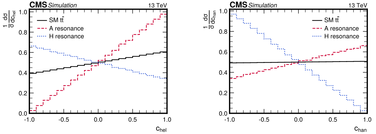
Figure 4: Normalized differential cross sections in the spin correlation observables c_{\text{hel}} (left) and c_{\text{han}} (right) at the parton level in the \ell\ell channel, with no requirements on acceptance, for SM t\bar{t} production (black solid), resonant A boson production (red dashed), and resonant H boson production (blue dotted). The corresponding distributions for \eta_t are identical to those of a A boson.
