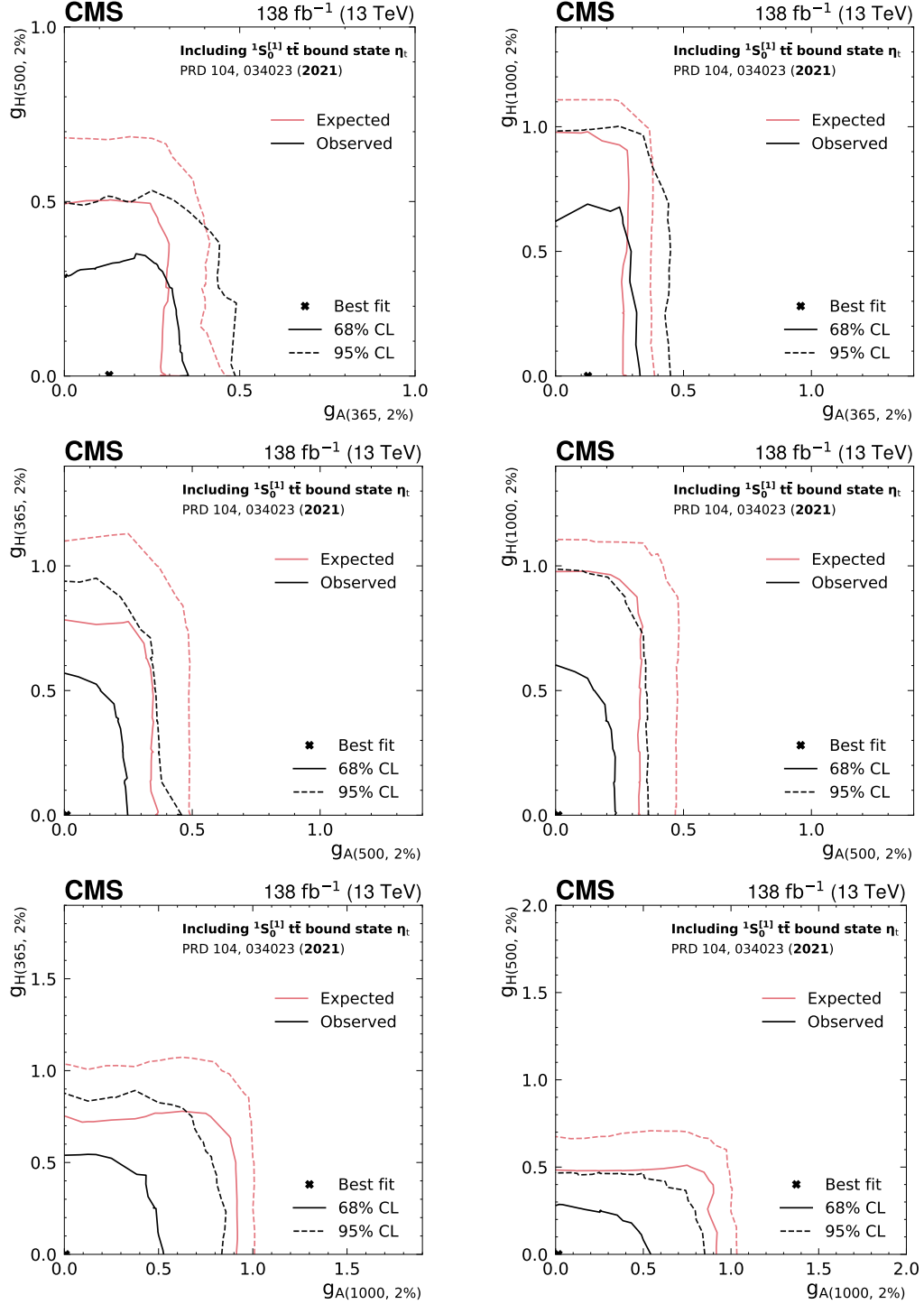
Figure 15: Frequentist 2D exclusion contours for g_{A t \bar{t}} and g_{H t \bar{t}} in the A+H boson interpretation for six different signal hypotheses with unequal A and H boson masses, corresponding to combinations of 365, 500, and 1000 GeV, all assuming a relative width of 2%. The expected and observed contours, evaluated with the Feldman–Cousins prescription [128, 129], are shown in pink and black, respectively, with the solid and dashed lines corresponding to exclusions at 68 and 95% CL. The regions outside of the contours are considered excluded. In all cases, \eta_t production is included in the background model.
