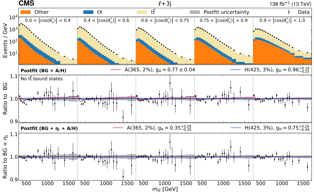
Figure 6: Observed and expected m_{t\bar{t}} distribution in bins of |\cos\theta_{t_\ell}^*| , shown for the \ell + 3j channel summed over lepton flavors and eras. In the upper panel, the data (points with statistical error bars) are compared to t\bar{t} production in FO pQCD and other sources of background (colored histograms) after the fit to the data in the A+H interpretation. The ratio of data to the prediction is shown in the middle panel, where the two signals A(365, 2%) and H(425, 3%), corresponding to the best fit point, are overlaid. The lower panel shows the equivalent ratio for the fit where \eta_t is considered as an additional background, for the same signal points. In both cases, the gray band shows the postfit uncertainty, and the respective signals are overlaid with their best fit model parameters.
