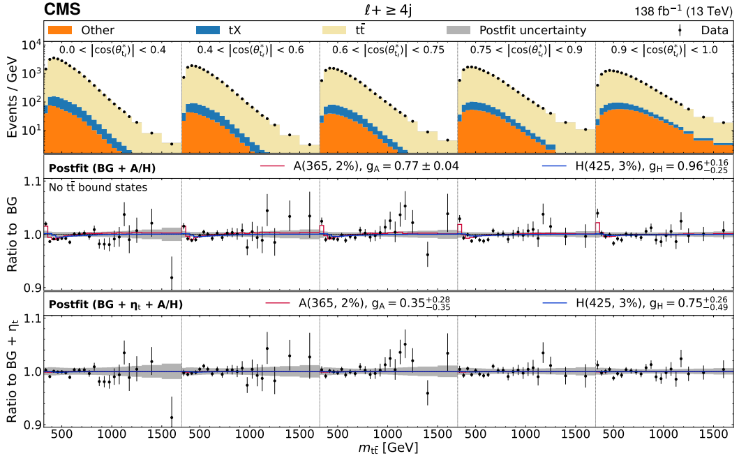
Figure 7: Observed and expected m_{t\bar{t}} distribution in |\cos\theta_{t_\ell}^*| bins, shown for the \ell + \geq 4j channel summed over lepton flavors and eras. Notations as in Fig. 6.
