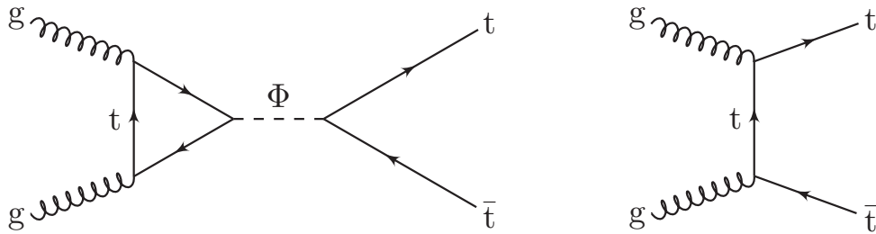
Figure 1: Example Feynman diagrams for the signal process (left) and for SM t\bar{t} production (right).
