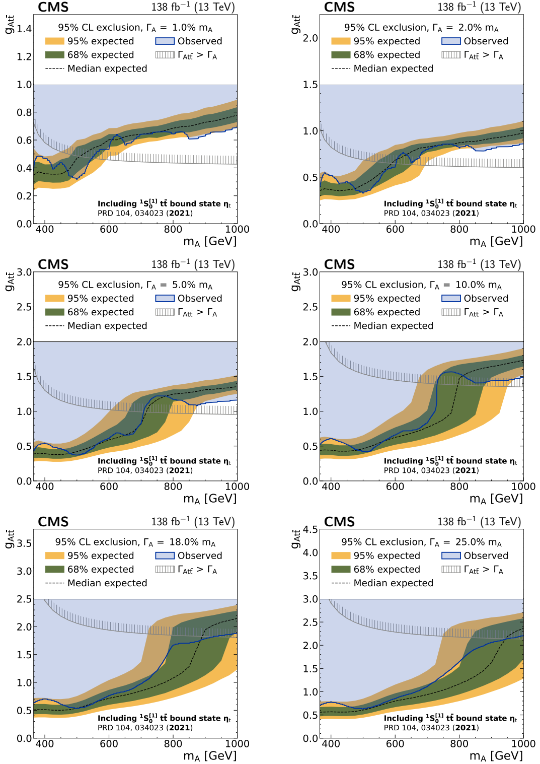
Figure 12: Model-independent constraints on g_{A\bar{t}t} as functions of the A boson mass in the background scenario with \eta_t contribution, shown in the same fashion as in Fig. 10.
