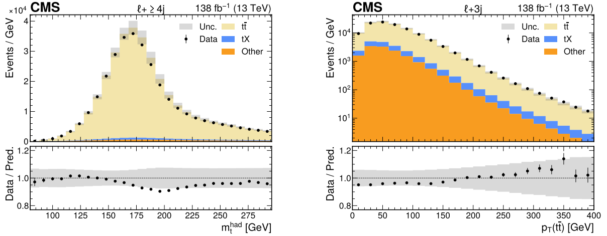
Figure 3: Comparison of the number of observed (points) and expected (colored histograms) events in the \ell j channel after the kinematic reconstruction and background estimation for the distributions of the reconstructed hadronic top quark mass m_t^{\text{had}} in the region with four or more jets (left) and the p_T of the t\bar{t} system in the region with exactly three jets (right). The ratio to the total prediction is shown in the lower panel, and the total systematic uncertainty is shown as the gray band.
