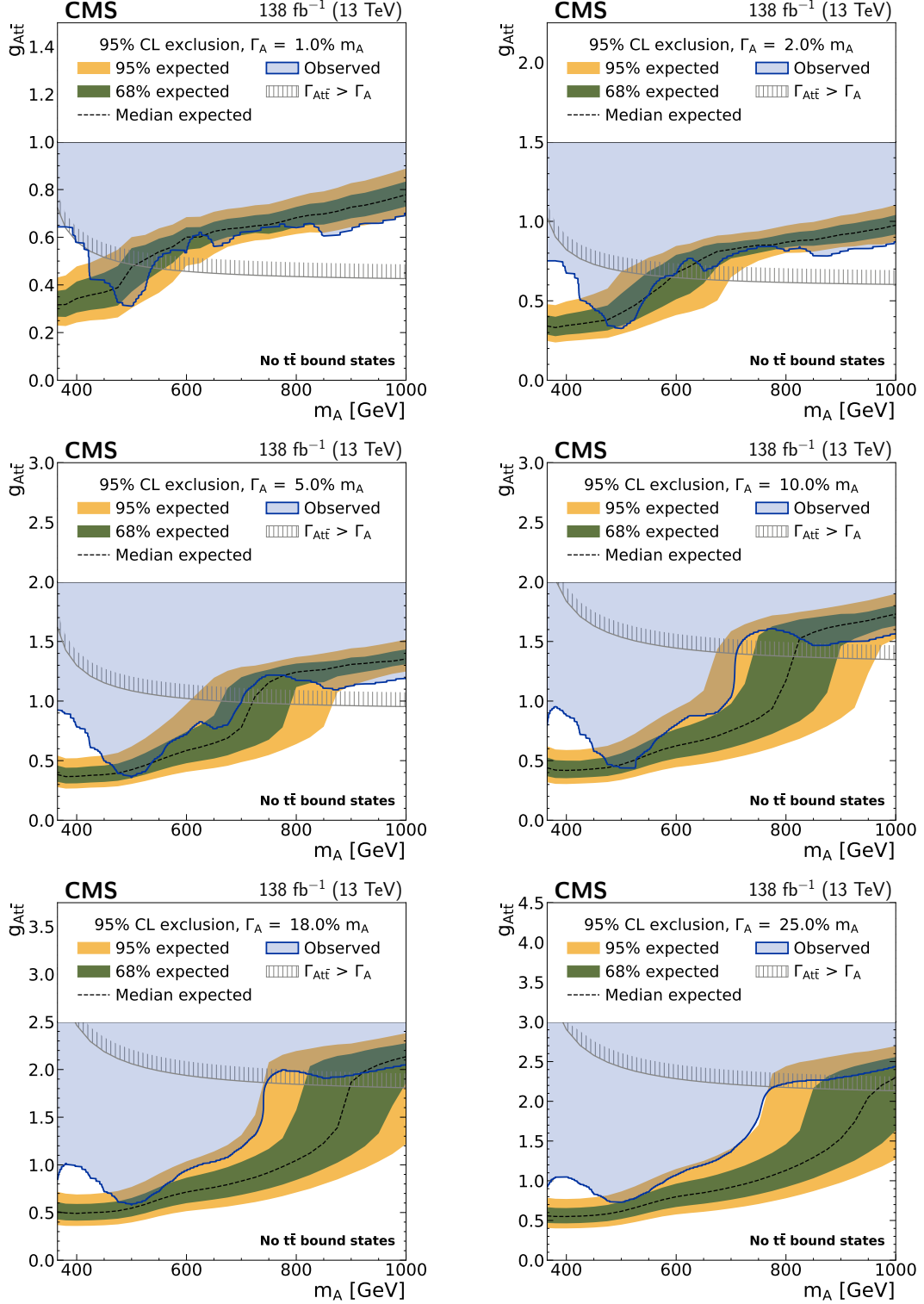
Figure 10: Model-independent constraints on g_{A t \bar{t}} as functions of the A boson mass in the background scenario without \eta_t contribution, for \Gamma_\Phi / m_\Phi of 1, 2, 5, 10, 18, and 25% (from upper left to lower right). The observed constraints are indicated by the shaded blue area, bounded by the solid blue curve. The inner green and outer yellow bands indicate the regions containing 68 and 95%, respectively, of the distribution of constraints expected under the background-only hypothesis. The unphysical region of phase space in which the partial width \Gamma_{A \rightarrow t \bar{t}} becomes larger than the total width of the A boson is indicated by the hatched line.
