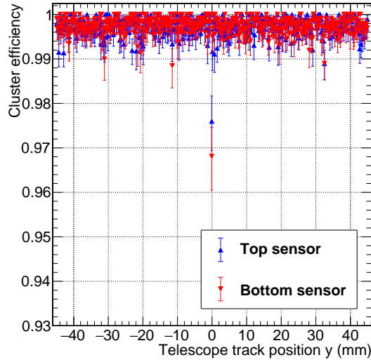
Figure 17. Cluster efficiency of module 1 as a function of the y -position for the top (blue) and bottom (red) sensor. The bin width in y is 200\ \mu\text{m} . The shown uncertainties are statistical only. The measurements are done with a hit detection threshold of approximately 6000\ e^- .
