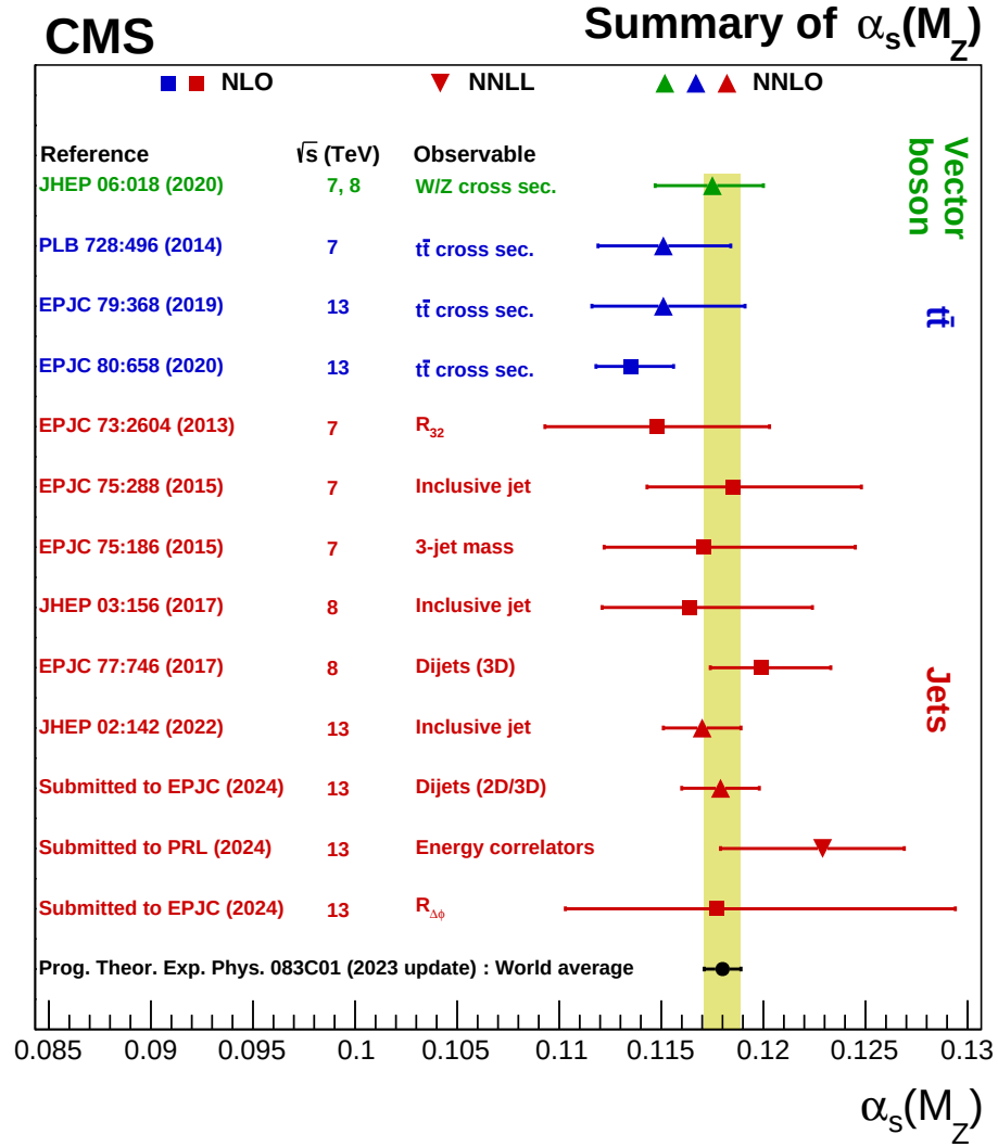
Figure 7: A summary of \alpha_s(m_Z) extractions from the CMS experiment compared with the 2023 PDG world-average. For each measurement, pp collision energy and the QCD perturbative order of the \alpha_s(m_Z) extraction are listed. Results are grouped by the type of the final state used: vector boson, t\bar{t} , and jets.
