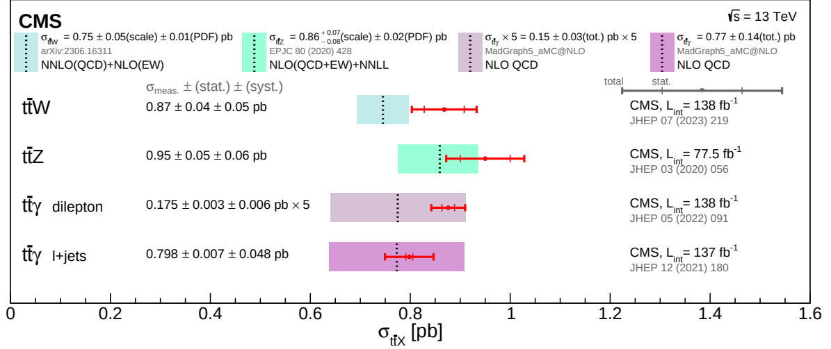
Figure 45: Summary of CMS t\bar{t}W and t\bar{t}V^0 cross section measurements with respect to the SM prediction. The horizontal bars display separately the statistical and the total uncertainties of the experimental measurements. The uncertainty associated to the theory predictions is represented by shaded bands and includes the variations of the renormalization and factorization scales and parton density functions.
