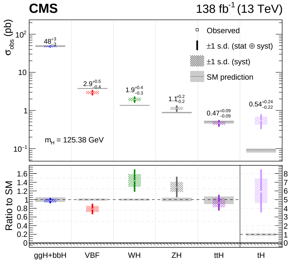
Figure 56: Measured cross sections for the main Higgs boson production modes. The best fit cross sections are plotted together with the respective 68% confidence level intervals. The systematic components of the uncertainty in each parameter are shown by the coloured boxes. The grey boxes indicate the theoretical uncertainties in the SM predictions. The lower panel shows the ratio of the fitted values to the SM predictions.
