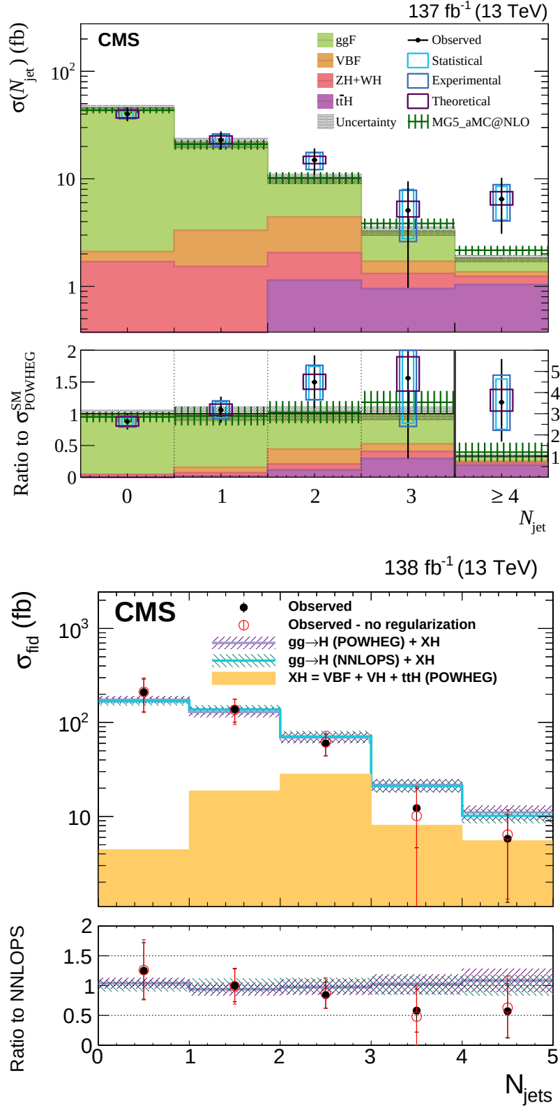
Figure 59: Differential fiducial cross sections for Higgs boson production as functions of the number of jets in the event, for the H \rightarrow WW [546] (upper) and H \rightarrow \tau\tau [545] (lower) decay modes. Figure compiled from Refs. [543, 554].
