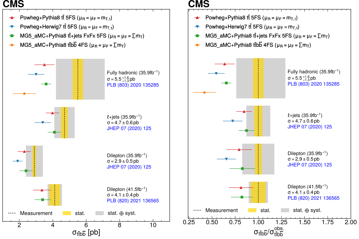
Figure 48: Summary of t\bar{t}b\bar{b} cross section measurements. The left plot depicts the measurements performed in the full phase space using different final states and data sets, compared with different MC predictions. The right plot shows the ratio between the theoretical and measured cross. The statistical and total uncertainties on the measurements are represented by different shaded bands, while the uncertainty on the predictions are represented by error bars.
