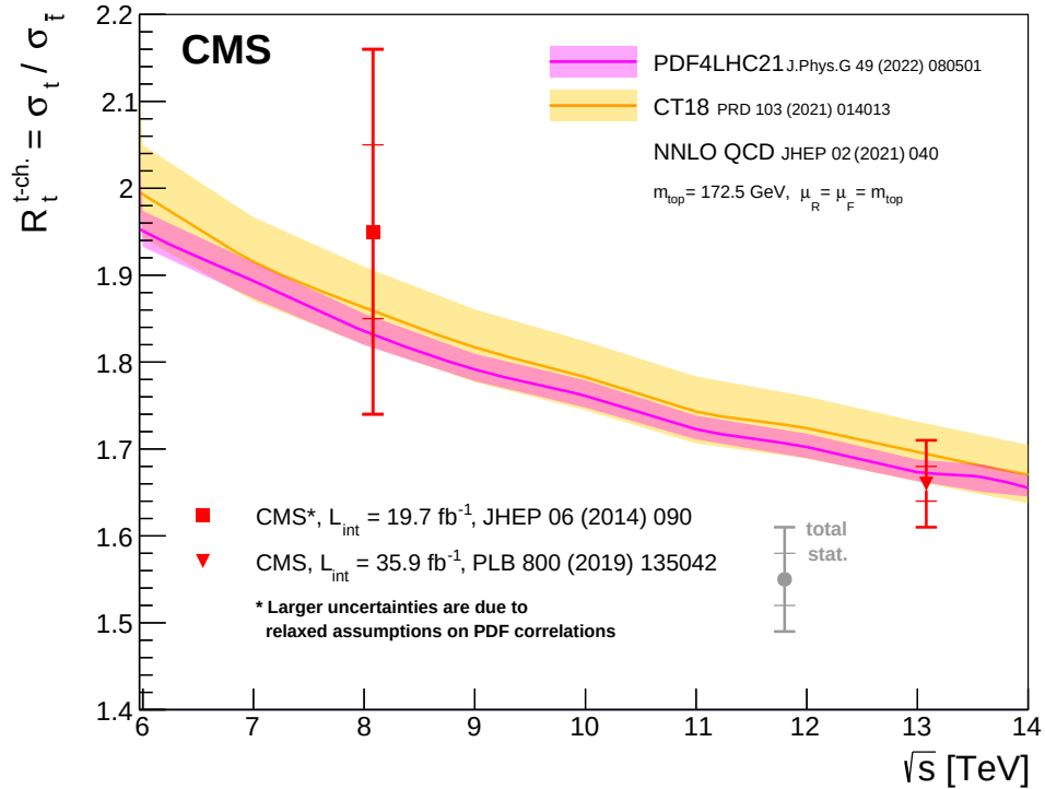
Figure 36: Summary of the CMS measurements of R_t = \sigma_t/\sigma_{\bar{t}} , the cross section ratio between t -channel top quark and t -channel top antiquark production. The measurements are compared with NNLO QCD calculations using the PDF sets CT18 and PDF4LHC21. The coloured bands represent the uncertainties in the theoretical predictions (scale and PDF uncertainties). The PDF uncertainties are estimated using the PDF4LHC21 prescription [399].
