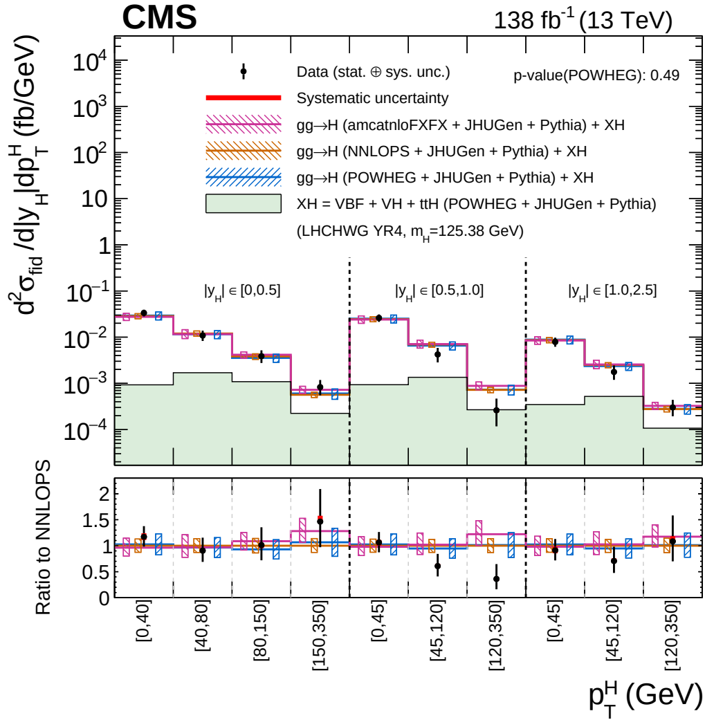
Figure 60: Double-differential cross sections for Higgs boson production in the H \rightarrow ZZ \rightarrow 4\ell decay channel. The cross section is measured in bins of the rapidity of the Higgs boson |y_H| , as a function of the Higgs boson transverse momentum p_T^H . Figure taken from Ref. [544].
