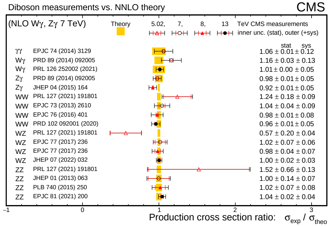
Figure 22: Summary of cross section measurements for diboson production shown as a ratio over the NNLO or NLO QCD predictions. The yellow bands indicate the uncertainties in the theoretical predictions and the error bars on the points are the statistical uncertainties, whereas the outer bars are the combined statistical and systematic uncertainties.
