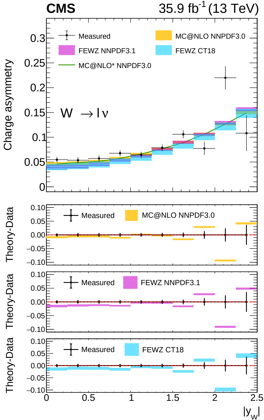
Figure 15: Measured W boson charge asymmetry as a function of |y_W| from the combination of the electron and muon channels (black dots), compared with different theoretical predictions. The vertical errors bars around the experimental data points show the total uncertainty of the measurements. The yellow band represents the default generator used in this analysis, MG5_aMC with the NNP3.0 PDF set, the pink band represents the FEWZ generator with the NNP3.1 PDF set, and the cyan band represents the FEWZ generator with the CT18 PDF set. The uncertainty bands of the prediction include the PDF uncertainties only, which are dominant with respect to \alpha_s , or renormalization and factorization scale variations for this quantity. Figure taken from Ref. [244].
