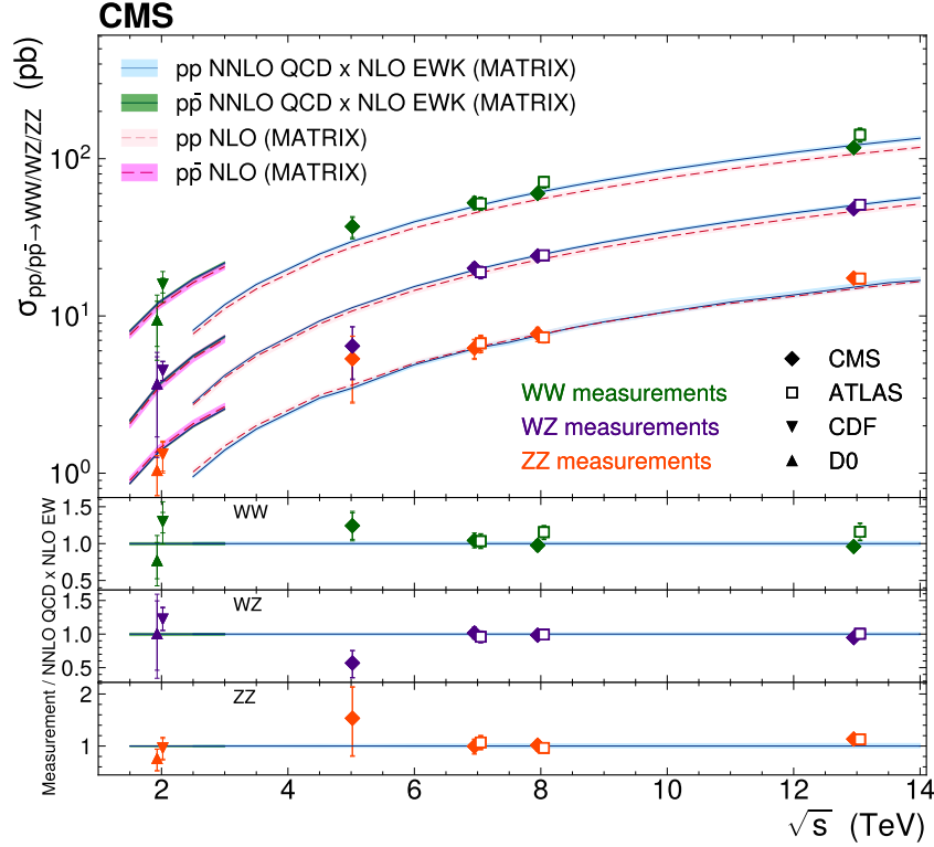
Figure 23: The total W^\pm W^\mp , WZ and ZZ cross sections as functions of the pp centre-of-mass energy. Results from the CMS and ATLAS experiments for pp collisions are compared with the predictions from MATRIX at NNLO in QCD and NLO in EW, and at NLO in QCD. Also shown are results from p\bar{p} collisions at the CDF and D0 experiments compared with MATRIX predictions as above. The inner vertical error bars around the experimental data points show the statistical uncertainties of the measurements, whereas the outer bars show the total uncertainties. Measurements at the same centre-of-mass energy are shifted slightly along the horizontal axis for clarity. Figure taken from Ref. [303].
