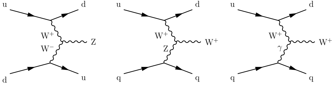
Figure 31: Feynman diagrams for vector boson fusion production of Z (left) and W bosons (middle) via the WWZ TGC vertex and W via the WW \gamma TGC vertex (right).
