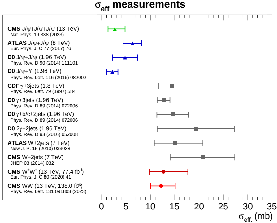
Figure 9: Selected measurements of the effective DPS cross section in pp collisions at the LHC by the CMS and ATLAS experiments, and in p\bar{p} collisions at the Tevatron by the CDF and D0 experiments. The horizontal bars indicate the combined statistical and systematic uncertainty for each measurement. Figure taken from Ref. [212].
