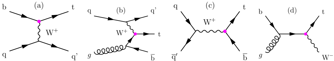
Figure 34: Feynman diagrams illustrating the pure EW contributions to single top quark production at the LHC at Born level. Charge conjugate states are implied. From left to right: the t -channel production, (a) with and (b) without a b quark in the initial state; (c) the s -channel; and (d) the tW -production. In all diagrams the tWq vertex is marked with a purple dot.
