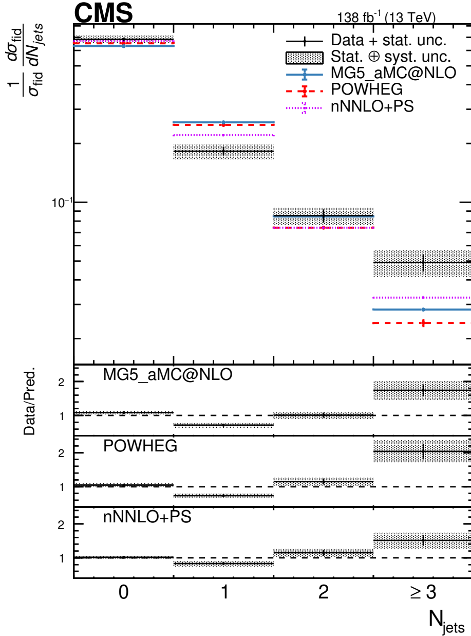
Figure 27: The differential cross section normalized to the fiducial cross section as a function of the number of jets. The on-shell Z requirement 60 < m_Z < 120 \text{ GeV} is applied for both Z boson candidates. Points represent the unfolded data, the solid lines the (MADGRAPH5_aMC@NLO q\bar{q} \rightarrow ZZ ) + (MCFM g g \rightarrow ZZ ) + (POWHEG H \rightarrow ZZ ) predictions, and red dashed lines the (POWHEG q\bar{q} \rightarrow ZZ ) + (MCFM g g \rightarrow ZZ ) + (POWHEG H \rightarrow ZZ ) predictions. The MADGRAPH5_aMC@NLO EW ZZ predictions are included. The purple dashed lines represent the nNNLO+PS predictions. Vertical bars on the MC predictions represent the statistical uncertainties. The lower panels show the ratio of the measured to the predicted cross sections. The shaded areas represent the full uncertainties calculated as the sum in quadrature of the statistical and systematic uncertainties and the vertical bars around the data points represent the statistical uncertainties only. The overflow events are included in the last bin of the distributions. Figure and caption taken from Ref. [324].
