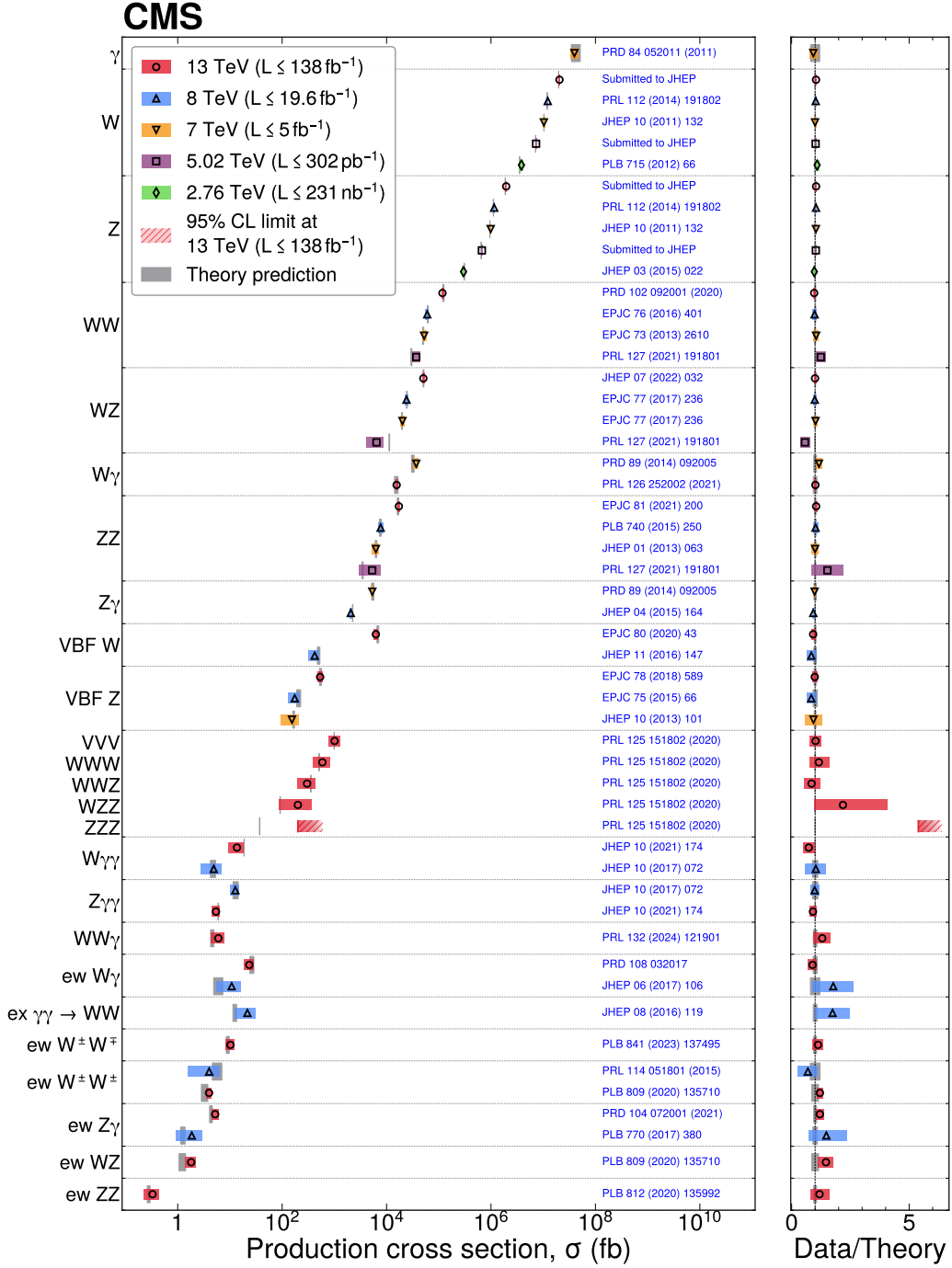
Figure 63: Summary of electroweak cross section measurements. Measurements performed at different LHC pp collision energies are marked by unique symbols and the coloured bands indicate the combined statistical and systematic uncertainty of the measurement. Grey bands indicate the uncertainty of the corresponding SM theory predictions. Shaded hashed bars indicate the excluded cross section region for a production process with the measured 95% C.L. upper limit on the process indicated by the solid line of the same colour.
