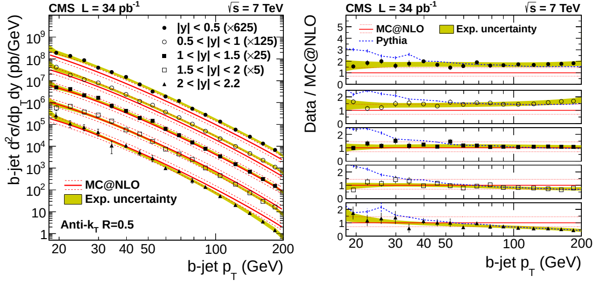
Figure 5: Measured b jet cross section from the jet analysis, multiplied by the arbitrary factors shown in the figure for easier viewing, compared to the MC@NLO calculation (left) and as a ratio to the MC@NLO calculation (right). The experimental systematic uncertainties are shown as a shaded band and the statistical uncertainties as error bars. The MC@NLO uncertainty is shown as dotted lines. The PYTHIA prediction is also shown in the right panel. Figure and caption taken from Ref. [155].
