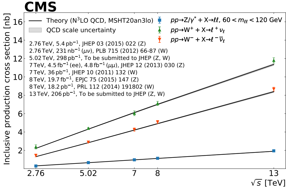
Figure 12: Summary of the production cross section of weak gauge bosons, measured by CMS, plotted against the pp centre-of-mass energy ranging from 2.76 to 13 TeV. The error bars around the experimental data points represent the total uncertainty of the measurement. The measurements are compared with theoretical predictions (black lines) obtained at N 3 LO in QCD using the MSHT20aN 3 LO PDF set. The grey band shows the envelope from renormalization and factorization scale variations.
