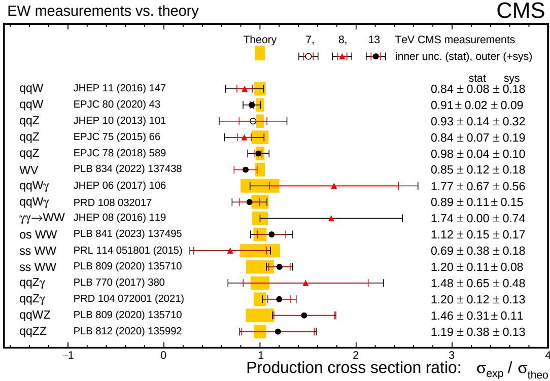
Figure 33: Summary of cross section measurements of EW single or diboson production processes including vector boson fusion, vector boson scattering, and scattering via exclusive processes. Production of pairs of W bosons can occur in same-sign (ss) W^{\pm}W^{\pm} , opposite-sign (os), W^{\pm}W^{\mp} , or exclusive production where photons are radiated from the incoming protons and form W^{\pm}W^{\mp} pairs via EW scattering. Results are displayed as a ratio of the experimental measurement over the SM prediction. The yellow bands indicate the uncertainties in the theoretical predictions and the error bars on the points are the experimental uncertainties, with the outer bar being the combined statistical and systematic uncertainty.
