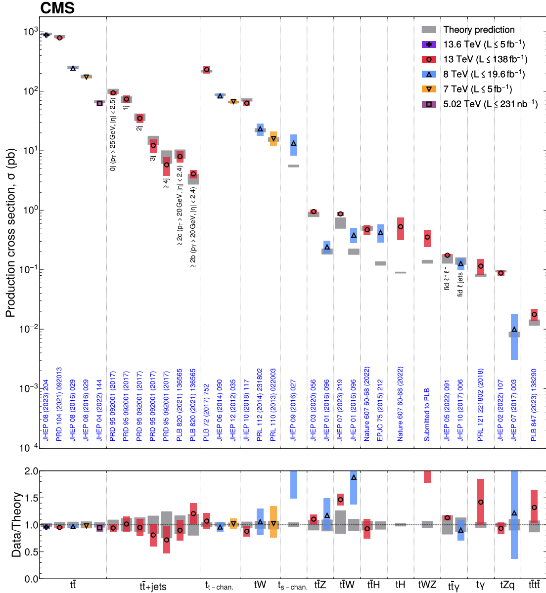
Figure 53: Summary of production cross section measurements involving top quarks. Measurements performed at different LHC pp collision energies are marked by unique symbols and the coloured bands indicate the combined statistical and systematic uncertainty of the measurement. Grey bands indicate the uncertainty of the corresponding SM theory predictions. Shaded hashed bars indicate the excluded cross section region for a production process with the measured 95% C.L. upper limit on the process indicated by the solid line of the same colour.
