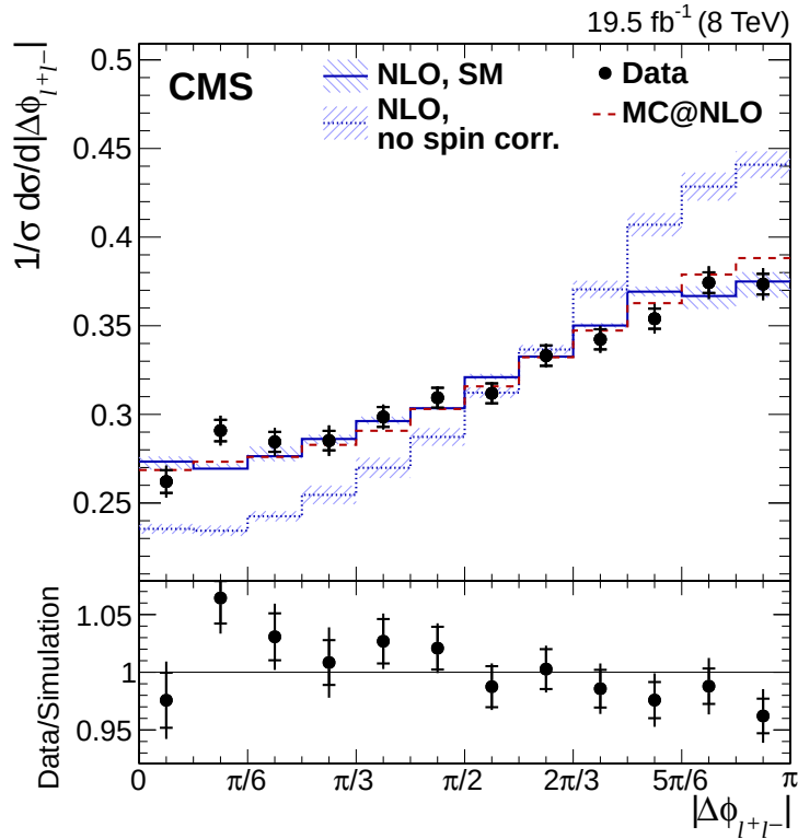
Figure 42: Normalized differential cross section as a function of the azimuthal opening angle between the two charged leptons in a t\bar{t} dilepton final state ( |\Delta\phi_{\ell^+\ell^-}| ) from data (points); parton-level predictions from MC@NLO (dashed histograms); and theoretical predictions at NLO with (SM) and without (no spin corr.) spin correlations (solid and dotted histograms, respectively). The ratio of the data to the MC@NLO prediction is shown in the lower panel. The inner and outer vertical bars on the data points represent the statistical and total uncertainties, respectively. The hatched bands represent variations of \mu_R and \mu_F simultaneously up and down by a factor of 2. Figure from Ref. [440].
