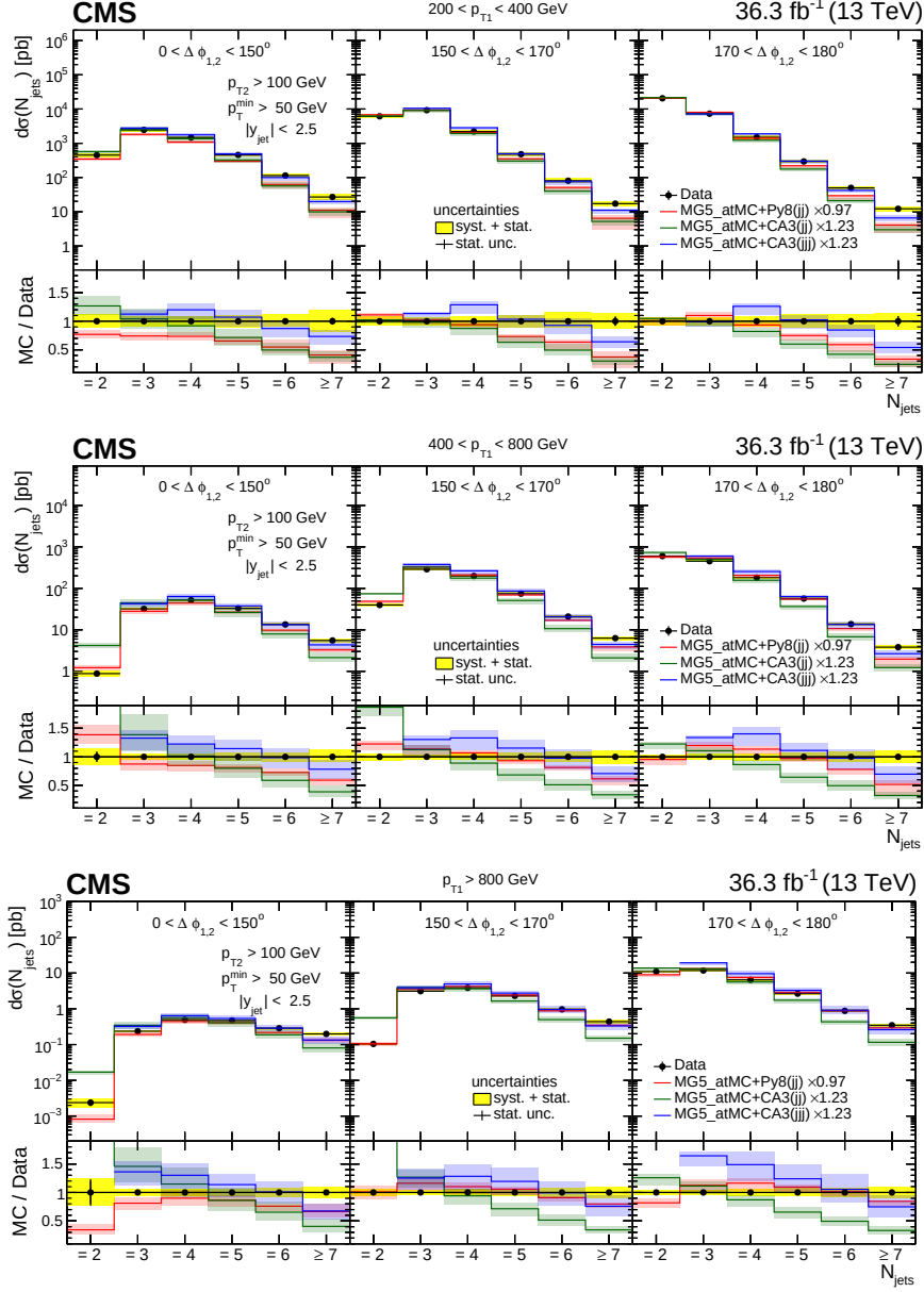
Figure 4: Differential cross section of jet production as a function of the exclusive jet multiplicity (inclusive for 7 jets) in bins of p_T and \Delta\phi_{12} . The data are compared with the NLO dijet predictions from MADGRAPH5_aMC@NLO: MG5_aMC+Py8 (jj) and MG5_aMC+CA3 (jj), as well as the NLO three-jet prediction of MG5_aMC+CA3 (jjj), where parton showering is performed by PYTHIA 8 (Py8) and CASCADE3 [88] (CA3). The vertical error bars correspond to the statistical uncertainty, the yellow band shows the total experimental uncertainty. The shaded bands show the uncertainty from a variation of the renormalization and factorization scales. The predictions are normalized to the measured inclusive dijet cross section using the scaling factors shown in the legend. Figure taken from Ref. [154].
