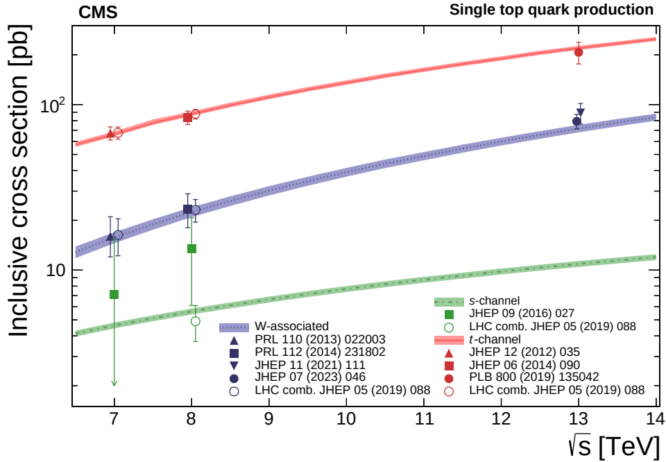
Figure 35: Single top quark cross section summary of CMS measurements as a function of the pp centre-of-mass energy. Where available the results from the full LHC combination are also overlaid for comparison. The theoretical calculations for t -channel, s -channel, and W-associated production are from Refs. [386–389].
