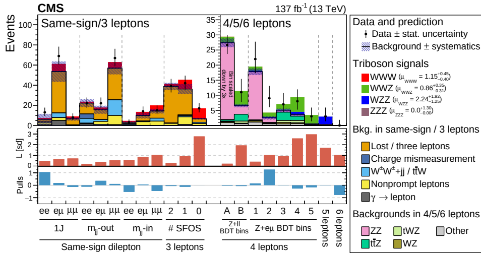
Figure 29: Comparison of the observed numbers of events to the predicted yields. For the WWW and WWZ channels, the results from boosted decision tree (BDT) based selections are used. For the other results different categorizations based on the number of jets, whether dijet masses are inside or outside a selection window used to identify the boson, and specific lepton combinations or the number of same-flavour, opposite-sign (SFOS) leptons are shown. The WWW signal is shown stacked on top of the total background. The points represent the data and the error bars show the statistical uncertainties. The expected significance L in the middle panel represents the number of standard deviations (sd) with which the null hypothesis (no signal) is rejected. The lower panel shows the pulls for the fit result. Figure taken from Ref. [332].
