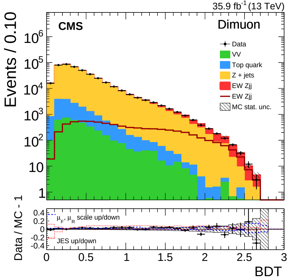
Figure 32: Distribution for a BDT discriminant used to select VBF Z events in dimuon events. The contributions from the different background sources and the signal are shown stacked, with data points superimposed. The vertical errors bars around the experimental data points show the total uncertainties. The expected signal-only contribution is also shown as an open histogram. The lower panel shows the relative difference between the data and expectations, as well as the uncertainty envelopes for the jet energy scale, and renormalization and factorization scale uncertainties. Figure taken from Ref. [344].
