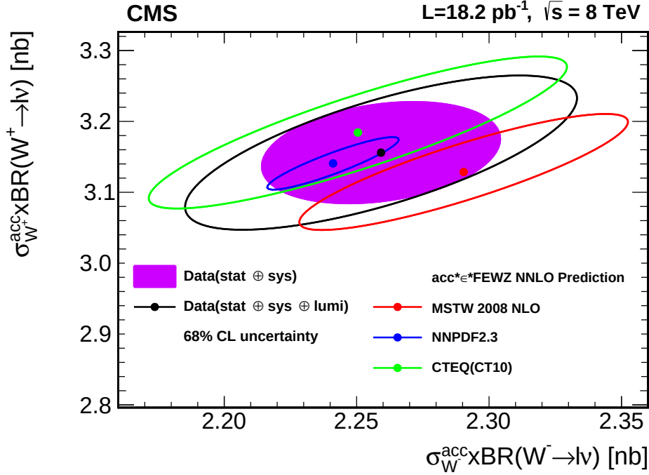
Figure 14: Measured and predicted W^+ versus W^- production fiducial cross sections times branching fractions. The ellipses illustrate the 68% CL coverage for total uncertainties (open) and excluding the integrated luminosity uncertainty (filled). The uncertainties in the theoretical predictions correspond to the PDF uncertainty components only and are evaluated for three PDF sets: NNPDF2.3, CTEQ CT10, and MSTW 2008 NLO. Figure taken from Ref. [231].
