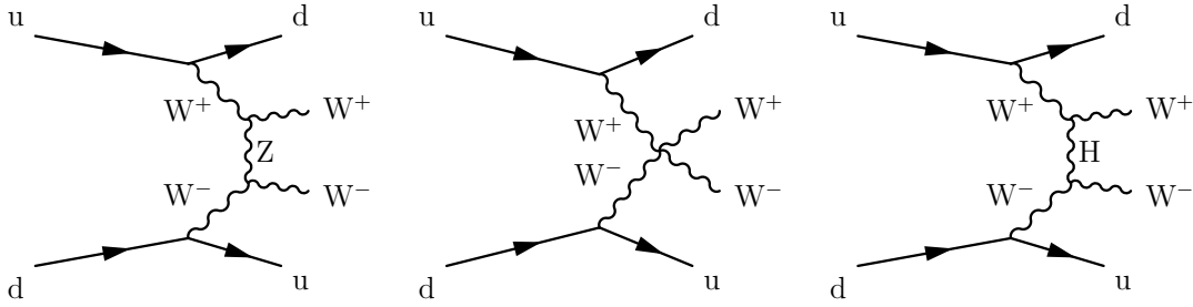
Figure 30: Production of oppositely charged W bosons via vector boson scattering. Example Feynman diagrams include: scattering via Z boson and two TGC vertices (left), a QGC vertex (middle), and scattering via a Higgs boson in t -channel (right).
