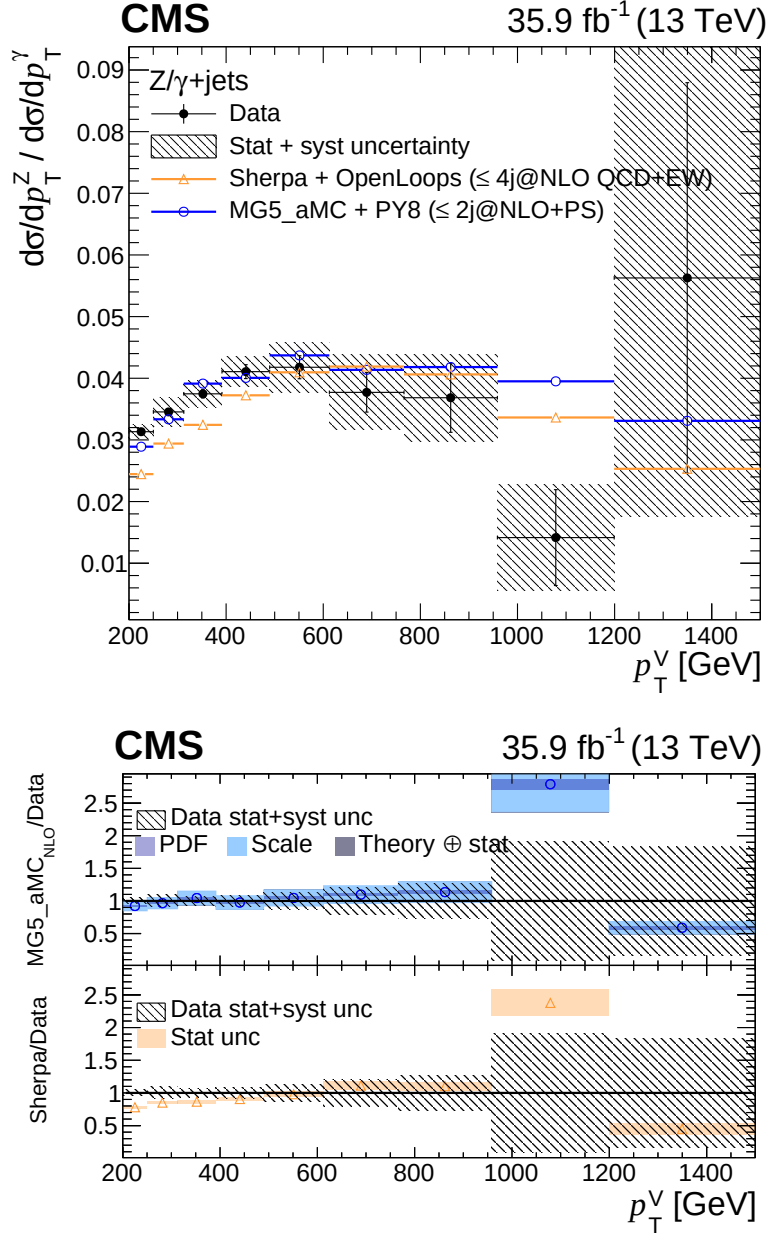
Figure 18: Differential cross section ratio of Z+jets (with Z \rightarrow \mu^+\mu^- ) to \gamma +jets as a function of the vector boson (V) transverse momentum compared with the theoretical prediction from MADGRAPH5_aMC@NLO and SHERPA + OPENLOOPS. Only bosons produced centrally, with |y| < 1.4 , in association with one or more jets are considered. The panel shows the ratio of the theoretical prediction to the unfolded data. The vertical errors bars around the experimental data points show the statistical uncertainties of the measurements. The hatched band is the sum in quadrature of the statistical and systematic uncertainty components in the measurement. The dark (light) shaded band on the NLO prediction from MADGRAPH5_aMC@NLO represents the PDF (scale) uncertainties, which are treated as uncorrelated between Z+jets and \gamma +jets, whereas the statistical uncertainties are barely visible. The shaded band on the SHERPA + OPENLOOPS calculation is the statistical uncertainty. Figure taken from Ref. [277].
