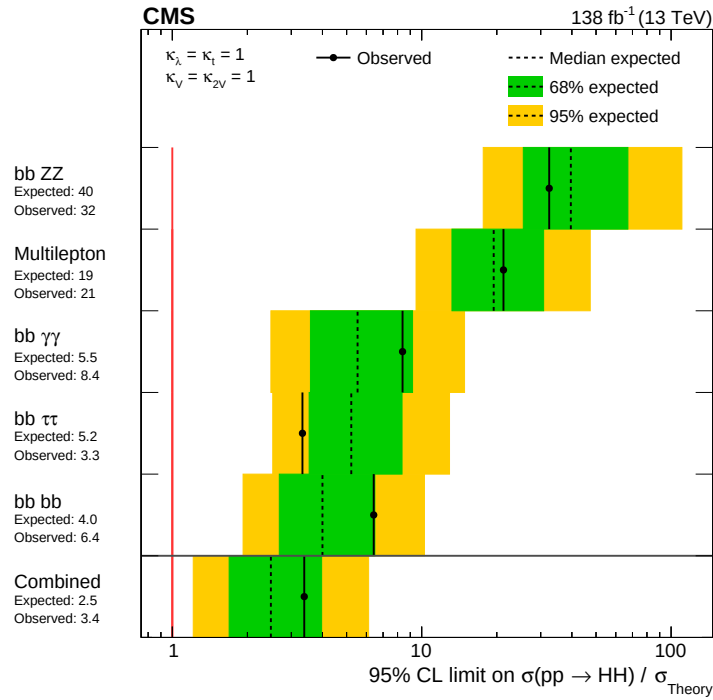
Figure 62: The expected and observed upper limits on the production of Higgs boson pairs. The results are expressed as a ratio to the SM prediction for the cross section ( \sigma(pp \rightarrow HH)/\sigma_{SM} ). A vertical red line at \sigma(pp \rightarrow HH)/\sigma_{SM} = 1 is drawn to guide the eye. The search modes are ordered, from upper to lower, by their expected sensitivities from the least to the most sensitive. The overall combination of all searches is shown by the lowest entry. Figure taken from Ref. [529].
