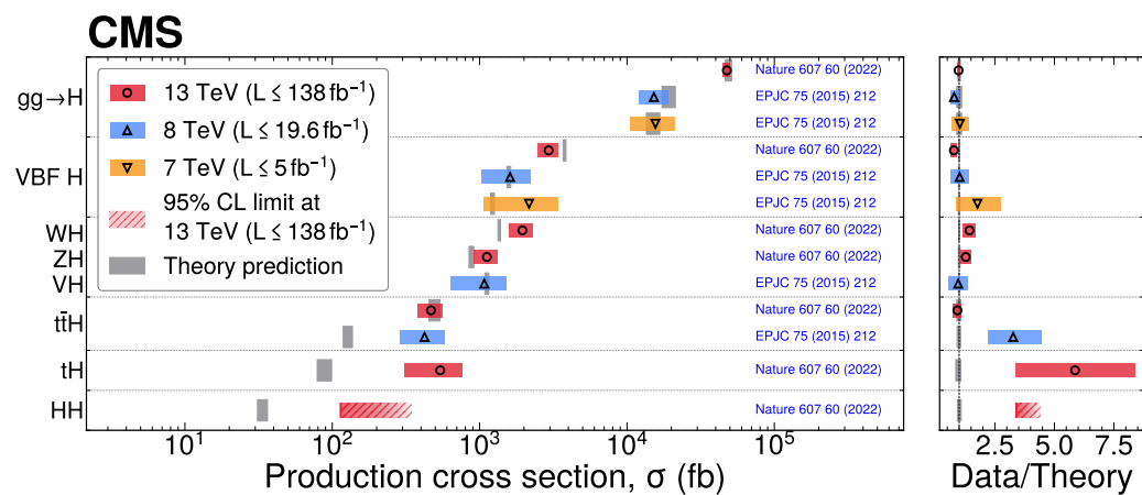
Figure 66: Summary of Higgs boson production cross section measurements.
