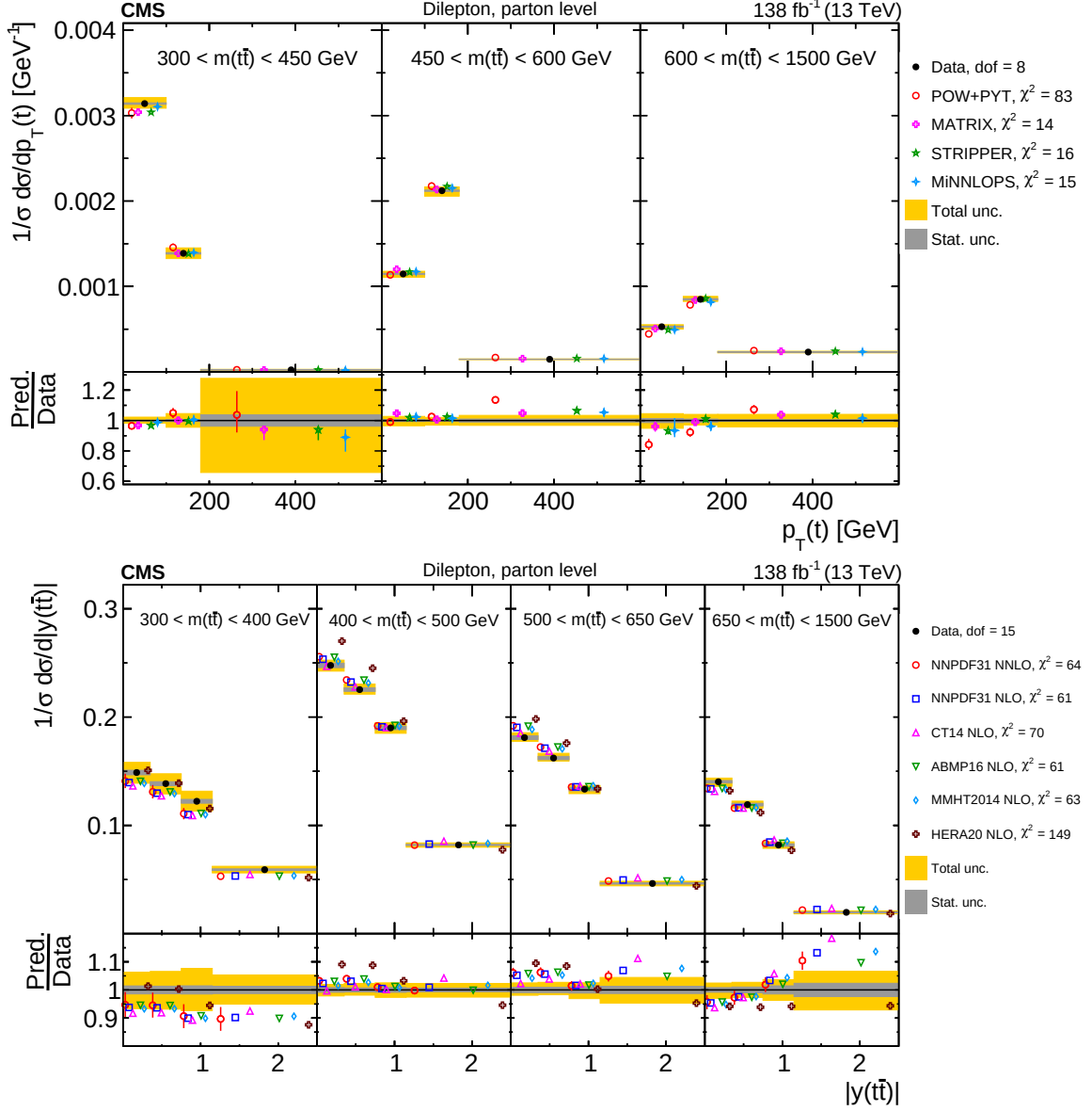
Figure 41: Normalized differential cross sections as a function of p_T(t) in bins of m(t\bar{t}) (upper), and as a function of y(t\bar{t}) in bins of m(t\bar{t}) (lower). The data, shown as bullets with grey and yellow bands indicating the statistical and total uncertainties, are compared with the prediction from POWHEG +PYTHIA 8 and various theoretical predictions (see text). The error bars represent the theory uncertainty in some of the predictions. The lower panel in each figure shows the ratios of the predictions to the data. Figure from Ref. [436].
