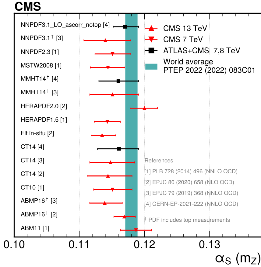
Figure 51: Summary of \alpha_S determinations from inclusive and differential top quark cross section measurements. The error bars represent the total uncertainty of the measurements. The results obtained with different PDF sets are compared with the world average [127] and the reference \alpha_S in the corresponding PDF set. The 68% confidence intervals are represented by the error bars and the coloured ranges. The PDFs marked with a † include LHC top quark data in their fits.
