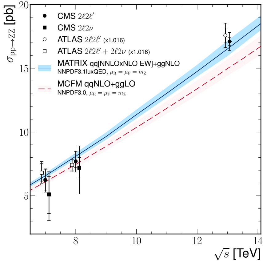
Figure 24: The total ZZ cross section as a function of the pp centre-of-mass energy. Results from the CMS and ATLAS [315–317] experiments are compared with the predictions from MATRIX and MCFM, as described in the text. The ATLAS measurements were performed with a Z boson mass window of 66–116 GeV, instead of 60–120 GeV used by CMS, and are corrected for the resulting 1.6% difference in acceptance. The inner vertical errors bars around the experimental data points show the statistical uncertainties of the measurements, whereas the outer bars show the total uncertainties. Measurements at the same centre-of-mass energy are shifted slightly along the horizontal axis for clarity. Figure taken from Ref. [308].
