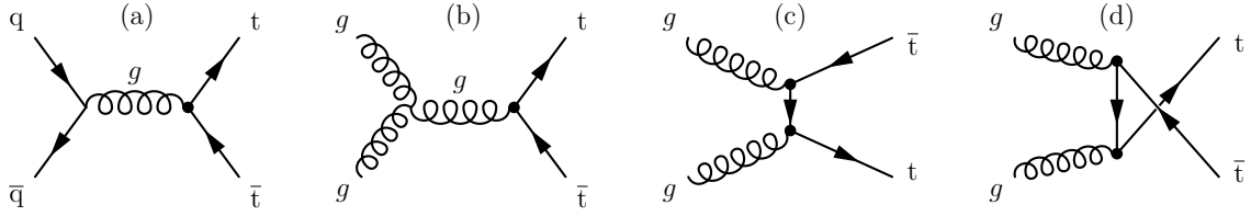
Figure 37: Leading order Feynman diagrams for t\bar{t} production.
