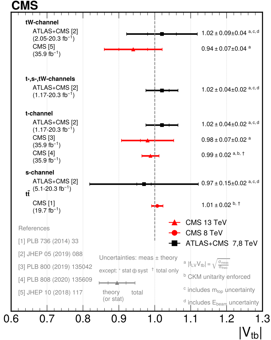
Figure 52: Summary of |V_{tb}| determinations from top quark events using different techniques. The values measured and the corresponding references are given in the figures. The error bars represent separately different uncertainties, as described in the legend. In the LHC combinations, the reference theory cross section used in the t - and s -channel measurements is computed at NLO QCD accuracy [387] with the PDF4LHC prescription for the PDF uncertainty using CT10nlo, MCSTW2008nlo, and NNPDF2.3nlo [500], whereas in the tW channel the theory reference is computed at NNLO+NNLL QCD accuracy [501] using the MSTW2008 NNLO PDF [112]. A line at |V_{tb}| = 1 is used as a common reference.
