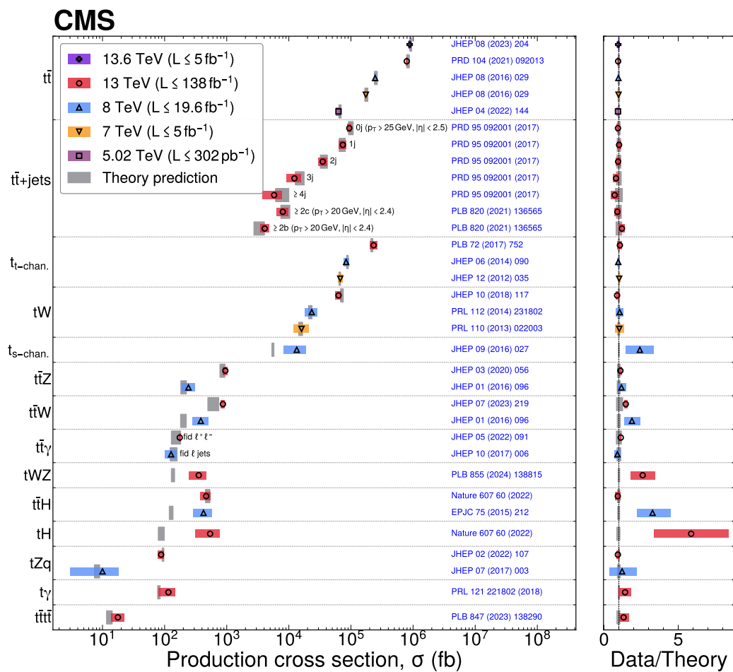
Figure 65: Summary of top quark production cross section measurements.
