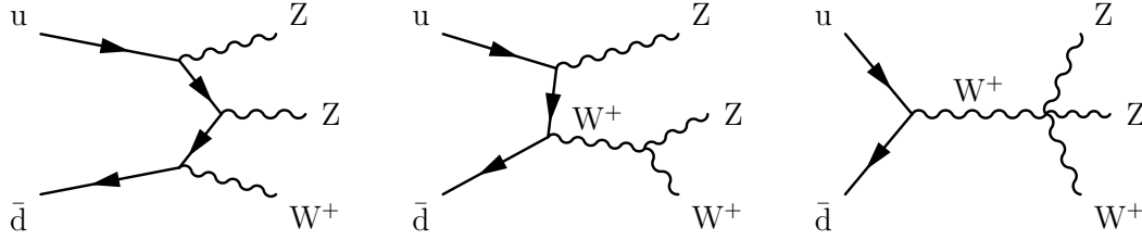
Figure 28: Triboson WZZ production via diagrams involving radiative production (left), TGCs (centre), and QGCs (right). This set of triboson Feynman diagrams is representative of most triboson signatures, with the caveat that neutral TGCs and some QGC combinations are not allowed in the SM.
