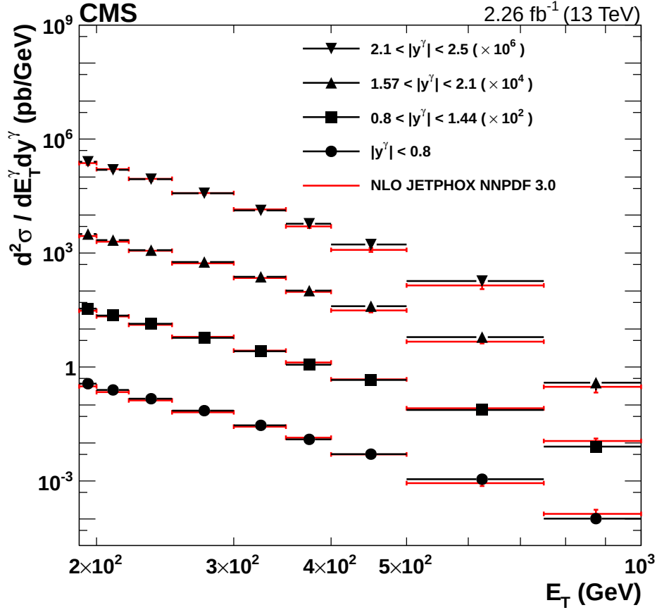
Figure 11: Differential cross sections for isolated-photon production in four photon rapidity intervals. The points show the measured values and their total uncertainties; the lines represent the NLO JETPHOX predictions with the NNPDF3.0 PDF set. Figure and caption taken from Ref. [223].
