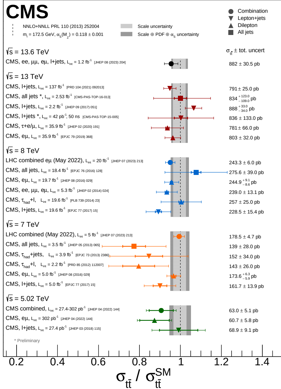
Figure 39: Summary of CMS top quark-antiquark pair cross section measurements at different \sqrt{s} , normalized to the theory calculation at NNLO+NNLL accuracy. The different final states and \sqrt{s} are respectively represented by various markers and colours. The total (statistical) uncertainty associated with the measurements is represented by the outer (inner) error bars.
