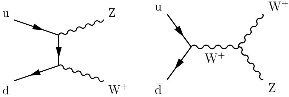
Figure 20: Feynman diagrams for WZ diboson production. Shown are radiative production (left), where the vector bosons are radiated off a quark, and a TGC production (right), where a W boson is created by q\bar{q} annihilation and splits into W and Z bosons. These diagrams are representative of all diboson production mechanisms that involve radiative or TGC processes. In the case of neutral final states TGCs are forbidden in the SM and only anomalous coupling due to new physics could lead to contributions from that type of diagram.
