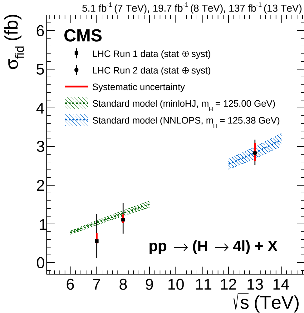
Figure 57: The measured inclusive fiducial cross section for H \rightarrow ZZ \rightarrow 4\ell as a function of \sqrt{s} . The acceptance is calculated using HRES [547, 548] at 7 and 8 TeV, and POWHEG at 13 TeV, and the total gluon fusion cross section and uncertainty are taken from Ref. [549]. The SM predictions and measurements are calculated at m_H = 125.0 GeV for \sqrt{s} = 6 –9 TeV, and at m_H = 125.38 GeV for 12–14 TeV. Figure taken from Ref. [509].
