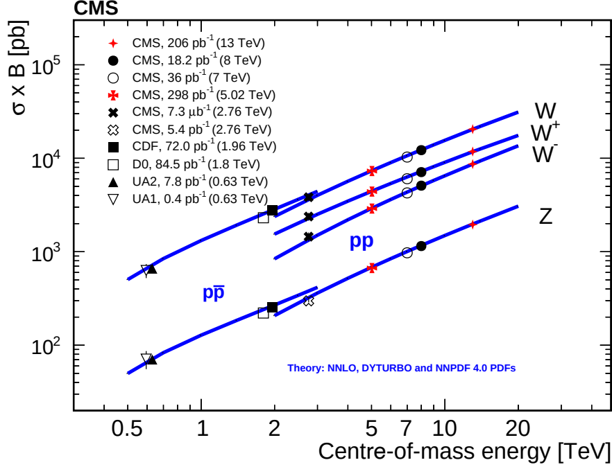
Figure 13: Summary of the production cross section of weak gauge bosons in pp collisions, measured by CMS, and in p\bar{p} collisions, by the UA1, UA2, CDF, and D0 experiments, plotted against the pp or p\bar{p} centre-of-mass energy ranging from 0.63 to 13 TeV. The measurements are compared with theoretical predictions (blue lines) obtained at NNLO in QCD by using DYTURBO and the NNPDF4.0 PDF set. Figure taken from Ref. [228].
