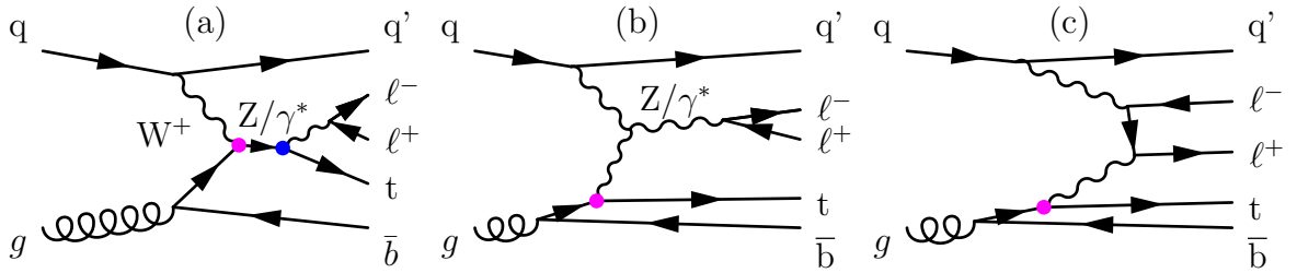
Figure 44: Example Feynman diagrams for the production of tZq .
