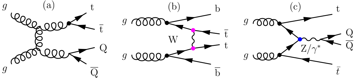
Figure 47: Feynman diagrams contributing to the associated production of top quarks with heavy-flavoured jets.
