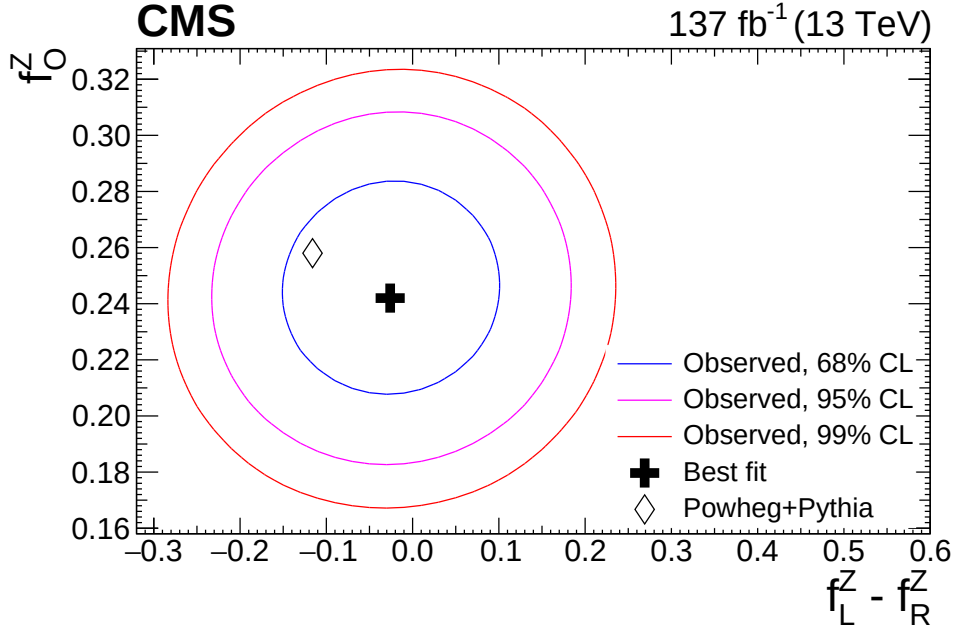
Figure 26: Confidence regions in the f_O^Z vs. f_L^Z - f_R^Z parameter plane for the Z boson polarization. The results are obtained with no additional requirement for the charge of the W boson. The blue, magenta, and red contours present the 68, 95, and 99% confidence levels, respectively. Figure from Ref. [306]. The cross indicates the best fit to the observed data and the diamond shows the result of the POWHEG + PYTHIA simulation.
