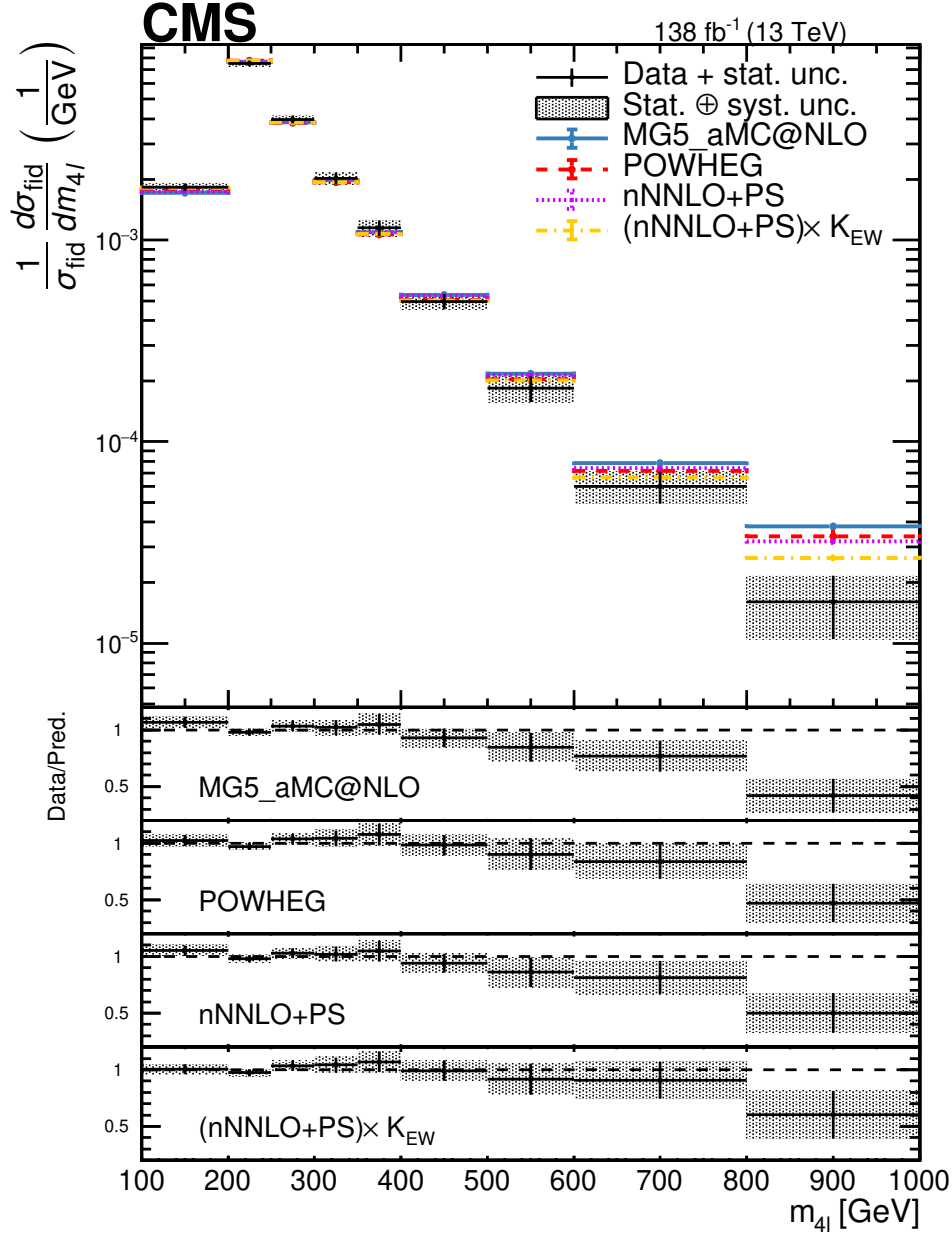
Figure 25: Differential cross section normalized to the fiducial cross section as a function of m_{4\ell} . The on-shell Z requirement 60 < m_Z < 120 GeV is applied for both Z boson candidates. Points represent the unfolded data, the solid lines the (MADGRAPH5_aMC@NLO q\bar{q} \rightarrow ZZ ) + (MCFM gg \rightarrow ZZ ) + (POWHEG H \rightarrow ZZ ) predictions, and red dashed lines the (POWHEG q\bar{q} \rightarrow ZZ ) + (MCFM gg \rightarrow ZZ ) + (POWHEG H \rightarrow ZZ ) predictions. The MADGRAPH5_aMC@NLO EW ZZ predictions are included. The purple dashed lines represent the nNNLO+PS predictions, and the yellow dashed lines represent the nNNLO+PS prediction with EW corrections applied. Vertical bars on the MC predictions represent the statistical uncertainties. The lower panels show the ratio of the measured to the predicted cross sections. The shaded areas represent the full uncertainties calculated as the sum in quadrature of the statistical and systematic uncertainties and the vertical bars around the data points represent the statistical uncertainties only. The overflow events are included in the last bin of the distributions. Figure and caption taken from Ref. [324].
