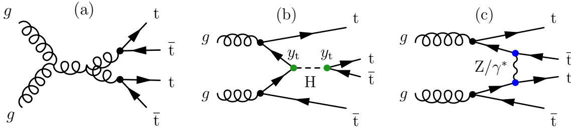
Figure 49: Representation of different Feynman diagrams contributing to t\bar{t}t\bar{t} production at the LHC. Diagrams that involve strong coupling vertices, shown in (a), are expected to dominate.
