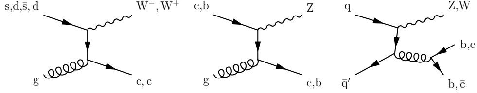
Figure 19: Production of W or Z bosons with heavy-flavour quarks. Examples of lowest order Feynman diagrams include W + charm (left), Z + charm or bottom (middle), W or Z production with two heavy-flavour quarks (right).
