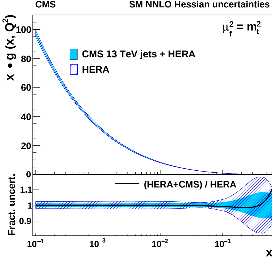
Figure 6: The gluon distribution, shown as a function of x for the factorization scale \mu_f = m_t . The filled (hatched) band represents the results of the NNLO fit using HERA DIS and the CMS inclusive jet cross section at \sqrt{s} = 13 TeV (using the HERA DIS data only). The PDFs are shown with their total uncertainty. In the lower panel, the comparison of the relative PDF uncertainties is shown for each distribution. The solid line corresponds to the ratio of the central PDF values of the two variants of the fit. Figure and caption taken from Ref. [151].
