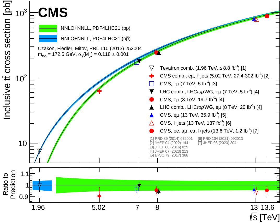
Figure 38: Summary of top quark-antiquark pair cross section measurements by the CMS Collaboration in comparison with the theory calculation at NNLO+NNLL accuracy. The Tevatron measurements are also shown. The lower panel displays the ratio between the different measurements and the theory prediction. The coloured bands represent the theory uncertainty, while the error bars represent the uncertainty on the measurements.
