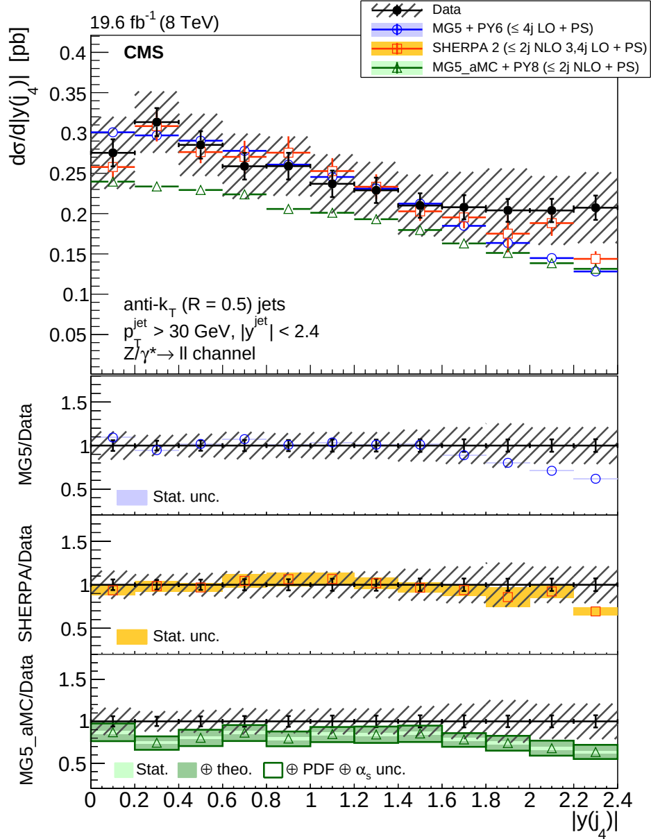
Figure 17: The differential cross section for Z \rightarrow \ell^+ \ell^- + \text{jets} production as a function of the absolute value of the 4th jet's rapidity compared with the predictions calculated with MADGRAPH 5+PYTHIA 6, SHERPA 2, and MG5_aMC +PYTHIA 8. The lower panels show the ratios of the theoretical predictions to the measurements. Error bars around the experimental points show the statistical uncertainty and the cross-hatched bands indicate the statistical and systematic uncertainties added in quadrature. The boxes around the MG5_aMC + PYTHIA 8 to measurement ratio represent the uncertainty in the prediction, including statistical, theoretical (from scale variations), and PDF uncertainties. The dark green area represents the statistical and theoretical uncertainties only and the light green area represents the statistical uncertainty alone. Figure taken from Ref. [264].
