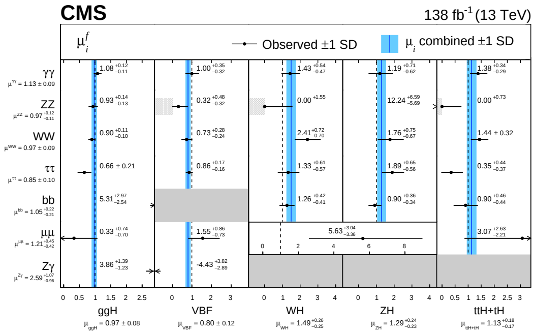
Figure 55: Signal strength parameters per individual production mode and decay channel \mu_i^f , and combined per production mode \mu_i and decay channel \mu^f . The SM expectation at 1 (dashed vertical lines) is shown as a reference. Light-grey shading indicates that \mu is constrained to be positive. Dark-grey shading indicates the absence of a measurement. The measured value for each production cross section modifier obtained from the combination across the decay channels, \mu_i , is indicated by the blue vertical line. The corresponding 68% CL interval is indicated by the blue bands. The arrows indicate cases where the confidence intervals exceed the scale of the horizontal axis. Figure taken from Ref. [529].
