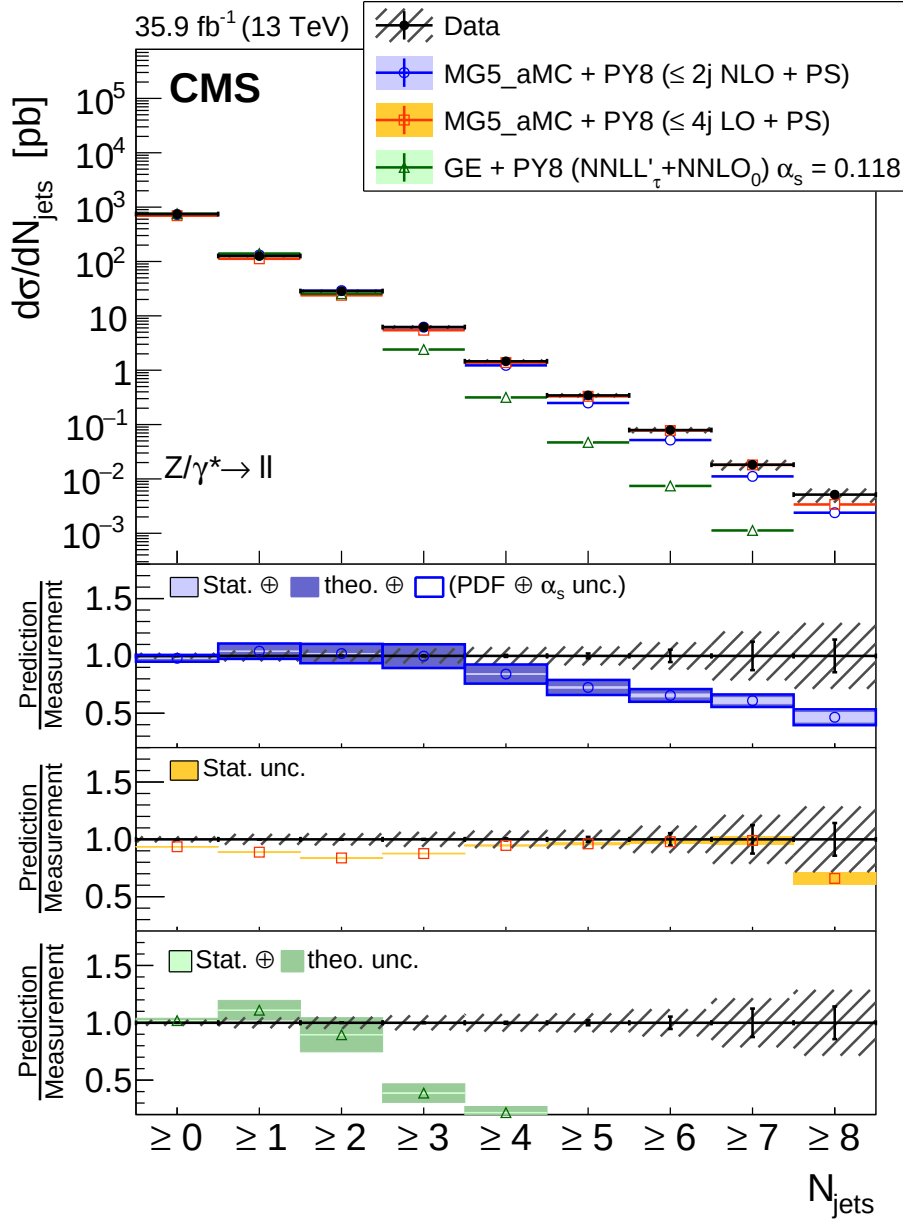
Figure 16: The differential cross section of Z \rightarrow \ell^+\ell^- + \text{jets} production as a function of inclusive jet multiplicity, compared with the predictions calculated with MADGRAPH5_aMC@NLO (LO) + PYTHIA 8, MADGRAPH5_aMC@NLO (NLO) + PYTHIA 8, and GENEVA. The lower panels show the ratios of the theoretical predictions to the measurements. The measurement statistical (systematic) uncertainties are presented with vertical error bars (hashed areas). The boxes around the MADGRAPH5_aMC@NLO (NLO) + PYTHIA 8 to measurement ratio represent the uncertainty in the prediction as listed in the legend. Figure taken from Ref. [256].
