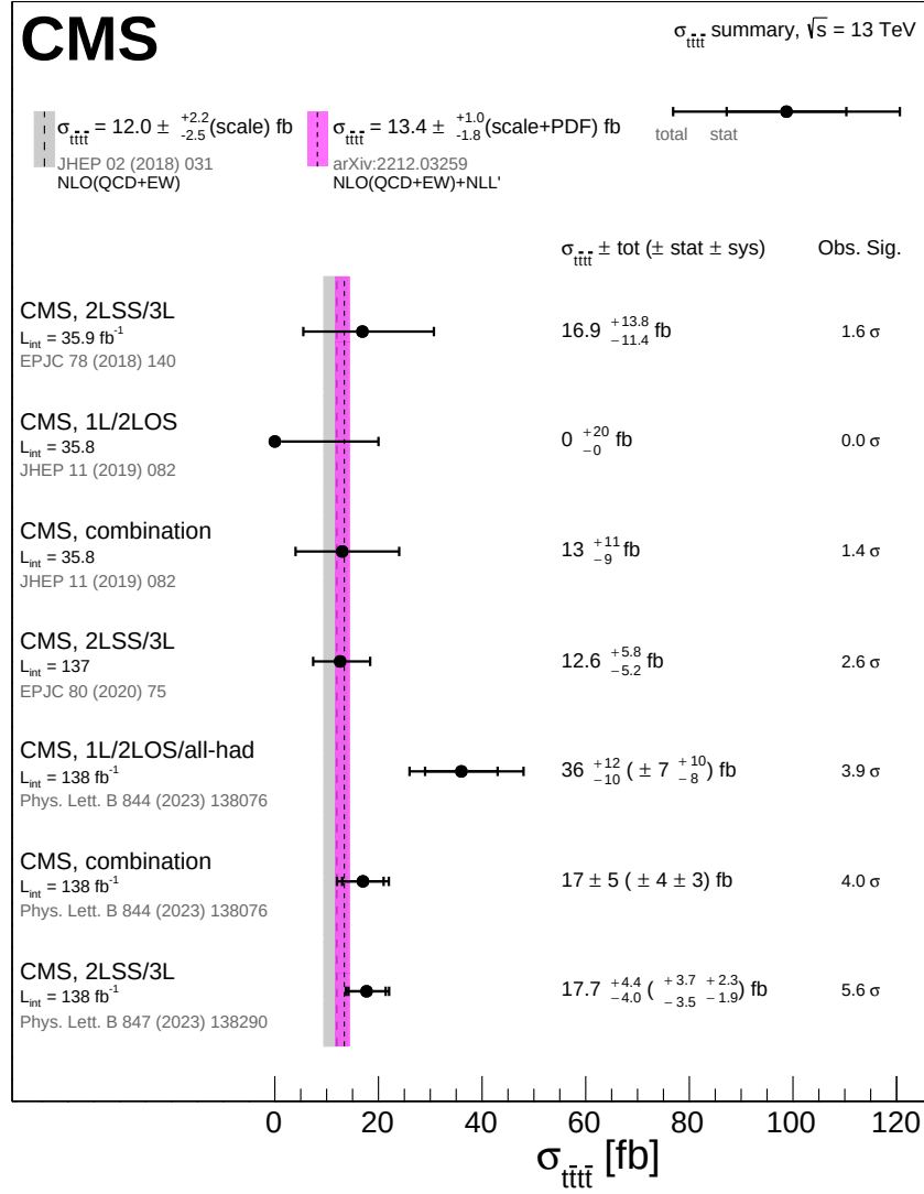
Figure 50: Summary of CMS measurements of the t\bar{t}t\bar{t} production cross section at 13 TeV in various channels. The total (statistical) uncertainty associated with the measurements is represented by the outer (inner) error bars. The cross section measurements are compared with the NLO QCD and EW theoretical calculation. The theoretical band represents uncertainties due to renormalization and factorization scales. Complementary theory predictions are also available in Ref. [493].
