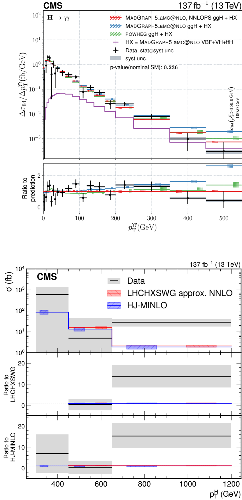
Figure 58: Differential fiducial cross sections for Higgs boson production in the H \rightarrow \gamma\gamma [543] (upper) and H \rightarrow b\bar{b} [554] (lower) decay channels as functions of the transverse momentum of the Higgs boson p_T^H . Figure compiled from Refs. [543, 554].
