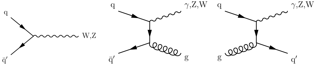
Figure 10: The Feynman diagram for Drell–Yan production of W and Z bosons (left). The Z boson production process involves annihilation of quark-antiquark pairs of same flavour. The W boson production process requires different-flavour quarks, such as u\bar{d} or \bar{u}d pairs. The NLO diagrams with real emission of a jet for the production of single vector bosons and one jet with a final-state gluon jet (middle) or quark jet (right).
