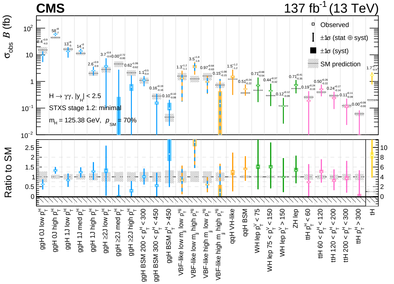
Figure 61: Observed results of the minimal merging scheme STXS fit for H \rightarrow \gamma\gamma at 13 TeV. The best fit cross sections are plotted together with the respective 68% confidence level intervals. Figure taken from Ref. [512].
