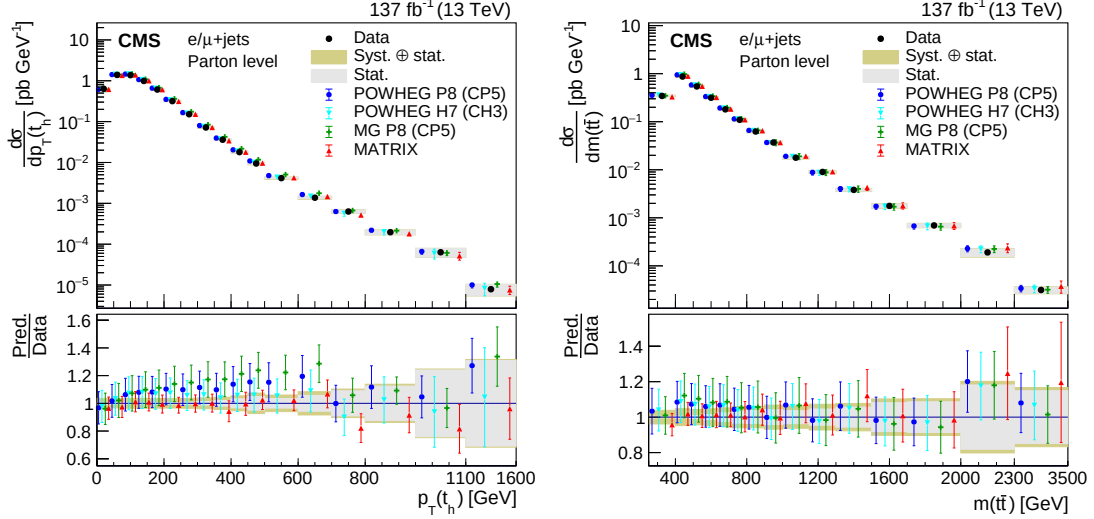
Figure 40: Differential cross sections at the parton level as a function of the hadronically decaying top quark p_T (left) and of the t\bar{t} invariant mass (right). The analysis was performed using t\bar{t} events in the \ell +jets final state. The data are shown as points with grey (yellow) bands indicating the statistical (statistical and systematic) uncertainties. The cross sections are compared with the predictions of POWHEG combined with PYTHIA (P8) or HERWIG (H7), the multiparton simulation MADGRAPH5_aMC@NLO (MG)+PYTHIA FxFx, and the NNLO QCD calculations obtained with MATRIX. The error bars represent the theory uncertainty in the predictions. The ratios of the various predictions to the measured cross sections are shown in the lower panels. Figure from Ref. [419].
