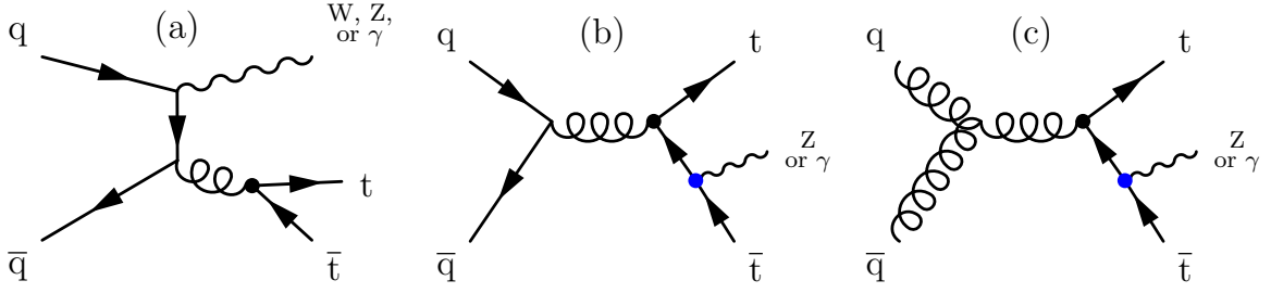
Figure 43: Example Feynman diagrams for the production of t\bar{t} with a vector boson through initial state radiation (a) or a direct coupling to the top quark (b and c). The latter is only possible for neutral bosons V^0 = \gamma, Z .
