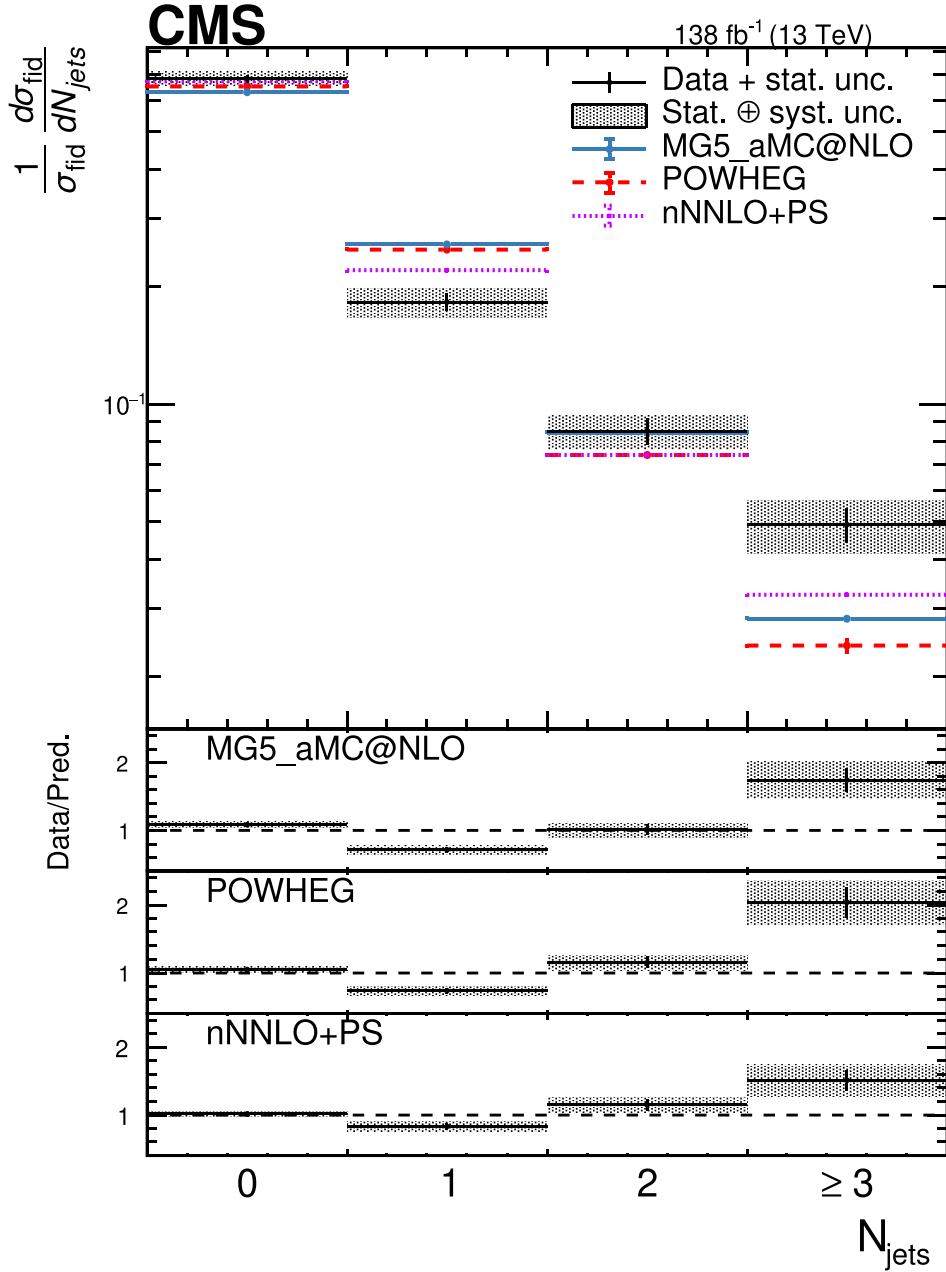
Fig. 27. The differential cross section normalized to the fiducial cross section as a function of the number of jets. The on-shell Z requirement 60 < m_Z < 120 GeV is applied for both Z boson candidates. Points represent the unfolded data, the solid lines the (MADGRAPH5_aMC@NLO q\bar{q} \rightarrow ZZ ) + (MCFM gg \rightarrow ZZ ) + (POWHEG H \rightarrow ZZ ) predictions, and red dashed lines the (POWHEG q\bar{q} \rightarrow ZZ ) + (MCFM gg \rightarrow ZZ ) + (POWHEG H \rightarrow ZZ ) predictions. The MADGRAPH5_aMC@NLO EW ZZ predictions are included. The purple dashed lines represent the nNNLO+PS predictions. Vertical bars on the MC predictions represent the statistical uncertainties. The lower panels show the ratio of the measured to the predicted cross sections. The shaded areas represent the full uncertainties calculated as the sum in quadrature of the statistical and systematic uncertainties and the vertical bars around the data points represent the statistical uncertainties only. The overflow events are included in the last bin of the distributions. Source: Figure and caption taken from Ref. [324].
