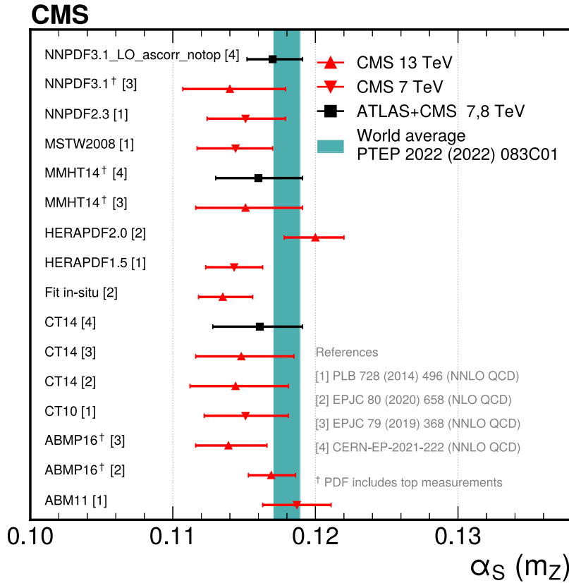
Fig. 51. Summary of \alpha_s determinations from inclusive and differential top quark cross section measurements. The error bars represent the total uncertainty of the measurements. The results obtained with different PDF sets are compared with the world average [127] and the reference \alpha_s in the corresponding PDF set. The 68% confidence intervals are represented by the error bars and the coloured ranges. The PDFs marked with a † include LHC top quark data in their fits.
