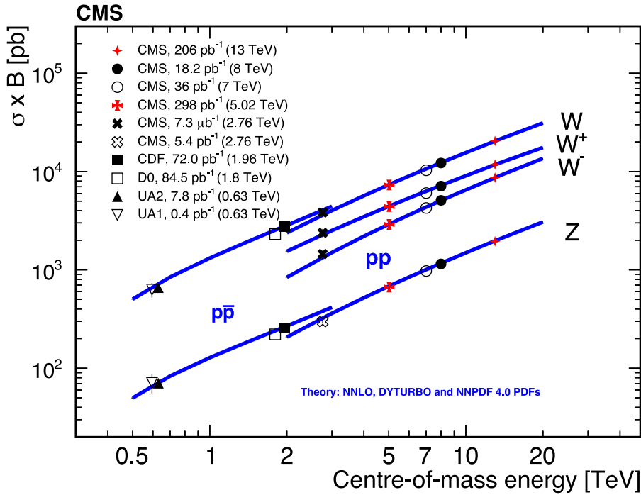
Fig. 13. Summary of the production cross section of weak gauge bosons in pp collisions, measured by CMS, and in p\bar{p} collisions, by the UA1, UA2, CDF, and D0 experiments, plotted against the pp or p\bar{p} centre-of-mass energy ranging from 0.63 to 13 TeV. The measurements are compared with theoretical predictions (blue lines) obtained at NNLO in QCD by using DYTURBO and the NNPDF4.0 PDF set.
