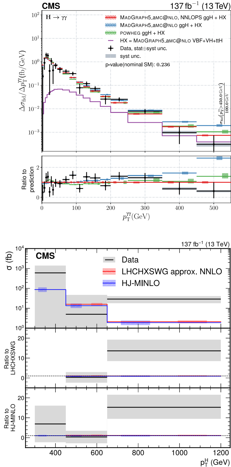
Fig. 58. Differential fiducial cross sections for Higgs boson production in the H \rightarrow \gamma\gamma [543] (upper) and H \rightarrow b\bar{b} [554] (lower) decay channels as functions of the transverse momentum of the Higgs boson p_T^H . Source: Figure compiled from Refs. [543,554].
