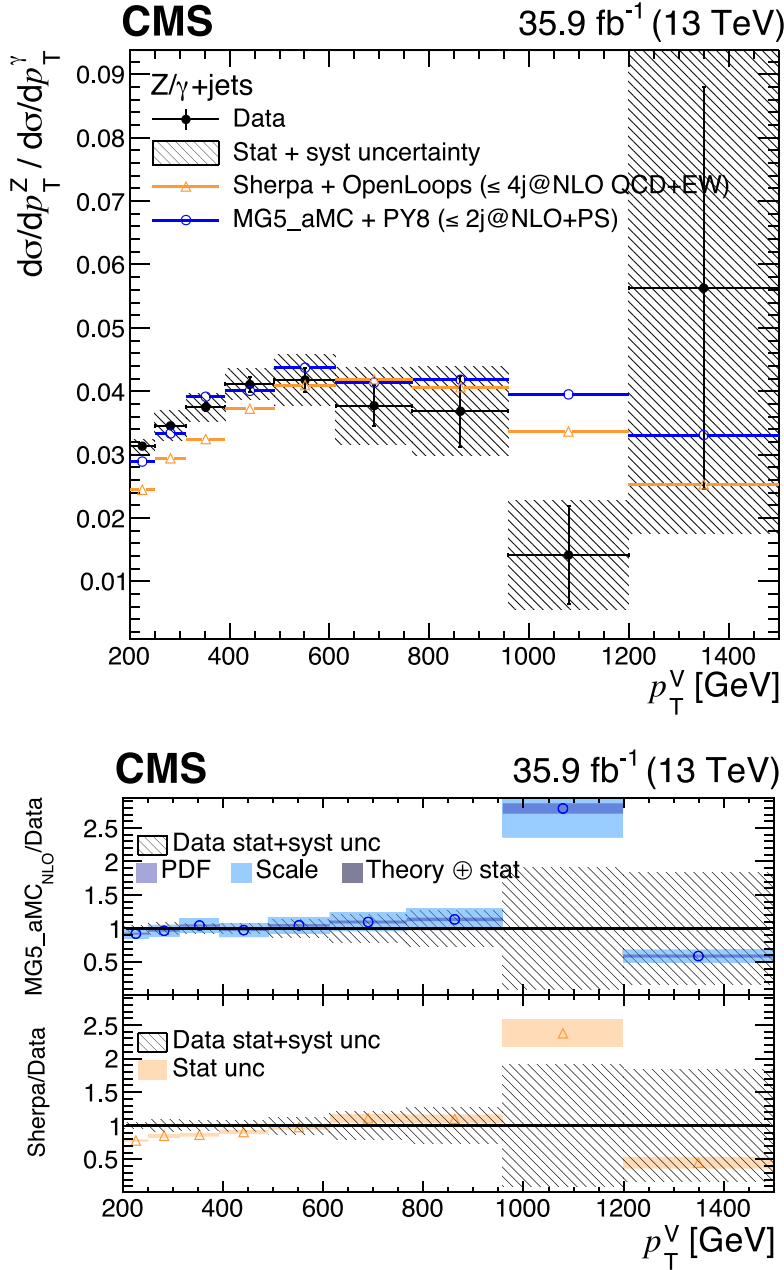
Fig. 18. Differential cross section ratio of Z+jets (with Z \rightarrow \mu^+\mu^- ) to \gamma +jets as a function of the vector boson (V) transverse momentum compared with the theoretical prediction from MADGRAPH5_aMC@NLO and SHERPA + OPENLOOPS. Only bosons produced centrally, with |y| < 1.4 , in association with one or more jets are considered. The panel shows the ratio of the theoretical prediction to the unfolded data. The vertical errors bars around the experimental data points show the statistical uncertainties of the measurements. The hatched band is the sum in quadrature of the statistical and systematic uncertainty components in the measurement. The dark (light) shaded band on the NLO prediction from MADGRAPH5_aMC@NLO represents the PDF (scale) uncertainties, which are treated as uncorrelated between Z+jets and \gamma +jets, whereas the statistical uncertainties are barely visible. The shaded band on the SHERPA + OPENLOOPS calculation is the statistical uncertainty.
