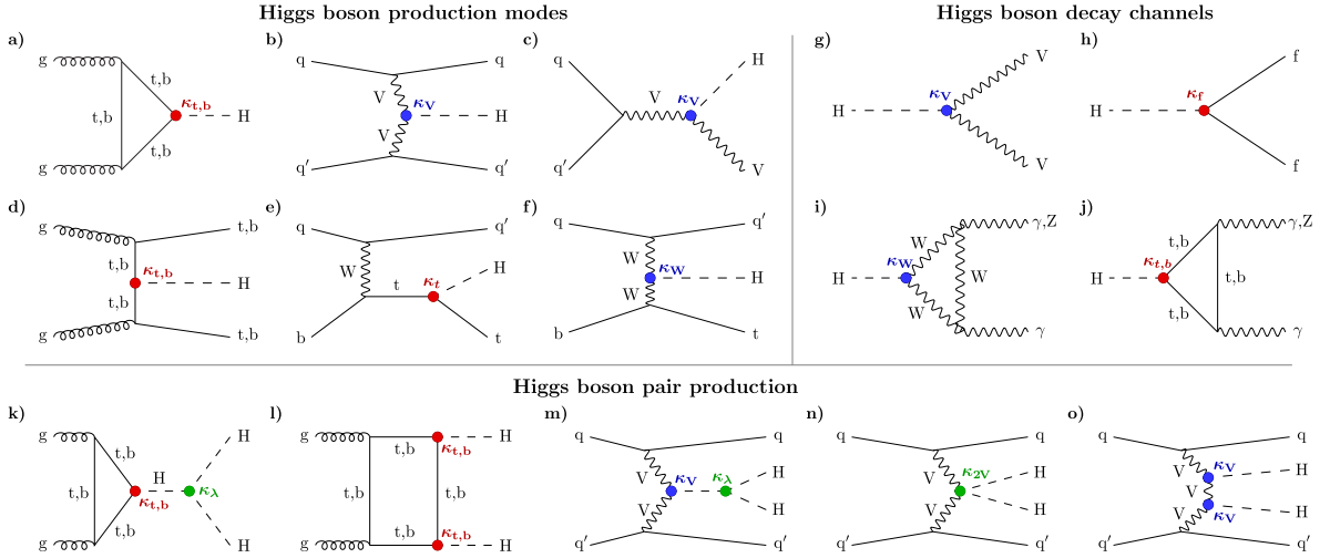
Fig. 54. Higgs boson production in (a) gluon-gluon fusion (ggH), (b) vector boson fusion (VBF), (c) associated production with a W or Z ( V ) boson ( VH ), (d) associated production with a top or bottom quark pair ( ttH or bbH ), (e, f) associated production with a single top quark ( tH ); with Higgs boson decays into (g) heavy vector boson pairs, (h) fermion-antifermion pairs, and (i, j) photon pairs or Z\gamma ; Higgs boson pair production: (k, l) via gluon-gluon fusion, and (m, n, o) via vector boson fusion. The corresponding Higgs boson interactions are labelled with the coupling modifiers \kappa , and highlighted in different colours for Higgs-fermion interactions (red), Higgs-gauge-boson interactions (blue), and multiple Higgs boson interactions (green). The distinction between a particle and its antiparticle is dropped.
