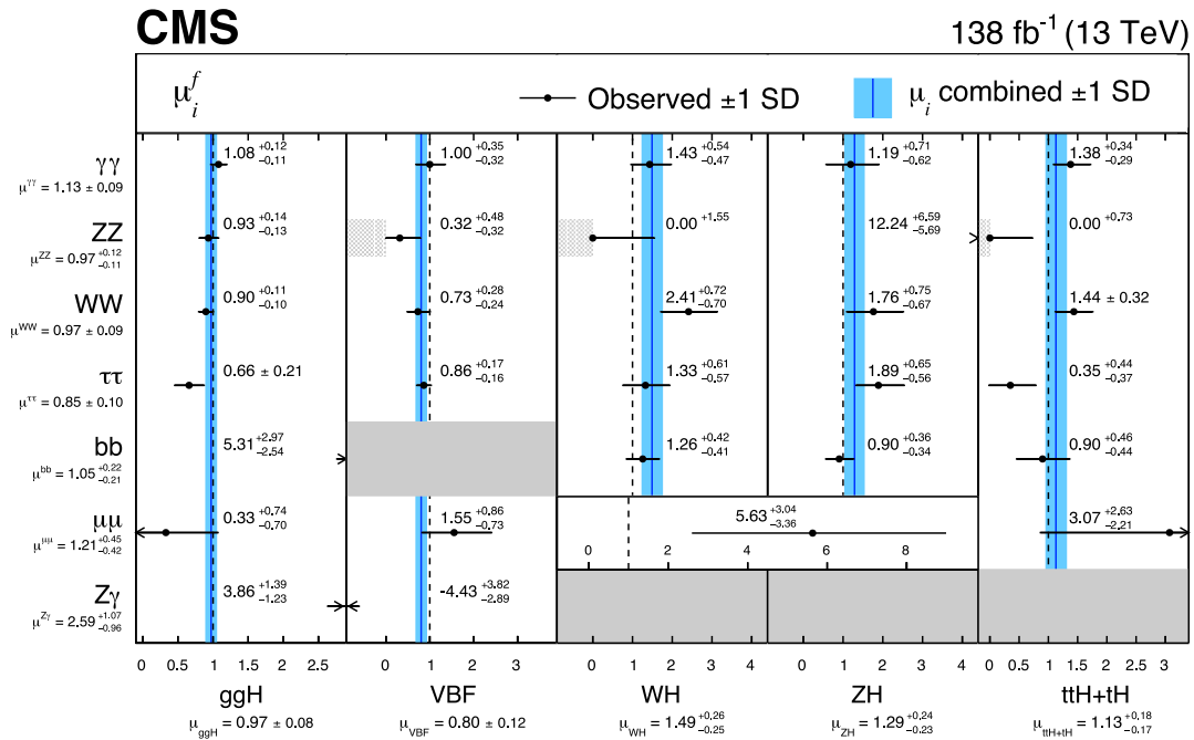
Fig. 55. Signal strength parameters per individual production mode and decay channel \mu_i^f , and combined per production mode \mu_i and decay channel \mu^f . The SM expectation at 1 (dashed vertical lines) is shown as a reference. Light-grey shading indicates that \mu is constrained to be positive. Dark-grey shading indicates the absence of a measurement. The measured value for each production cross section modifier obtained from the combination across the decay channels, \mu_i , is indicated by the blue vertical line. The corresponding 68% CL interval is indicated by the blue bands. The arrows indicate cases where the confidence intervals exceed the scale of the horizontal axis. Source: Figure taken from Ref. [529].
