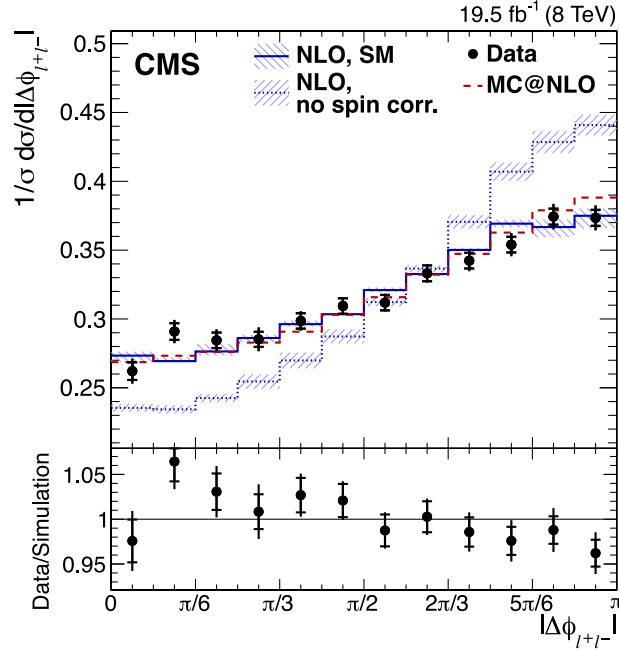
Fig. 42. Normalized differential cross section as a function of the azimuthal opening angle between the two charged leptons in a \tau\bar{\tau} dilepton final state ( |\Delta\phi_{\ell^+\ell^-}| ) from data (points); parton-level predictions from MC@NLO (dashed histograms); and theoretical predictions at NLO with (SM) and without (no spin corr.) spin correlations (solid and dotted histograms, respectively). The ratio of the data to the MC@NLO prediction is shown in the lower panel. The inner and outer vertical bars on the data points represent the statistical and total uncertainties, respectively. The hatched bands represent variations of \mu_R and \mu_F simultaneously up and down by a factor of 2. Source: Figure from Ref. [440].
