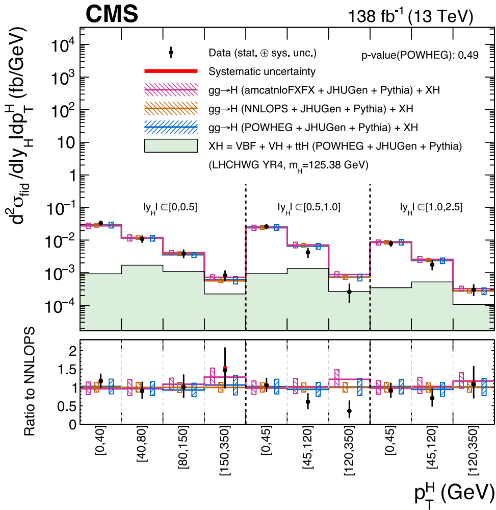
Fig. 60. Double-differential cross sections for Higgs boson production in the H \rightarrow ZZ \rightarrow 4\ell decay channel. The cross section is measured in bins of the rapidity of the Higgs boson |y_H| , as a function of the Higgs boson transverse momentum p_T^H . Source: Figure taken from Ref. [544].
