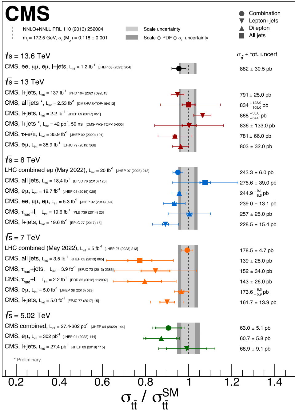
Fig. 39. Summary of CMS top quark-antiquark pair cross section measurements at different \sqrt{s} , normalized to the theory calculation at NNLO+NNLL accuracy. The different final states and \sqrt{s} are respectively represented by various markers and colours. The total (statistical) uncertainty associated with the measurements is represented by the outer (inner) error bars.
