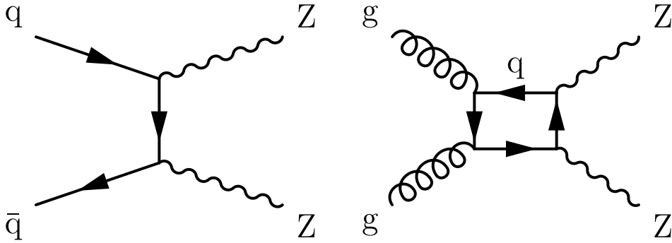
Fig. 21. Feynman diagrams for ZZ diboson production including radiative production (left) and NNLO production via a gluon–gluon initial state (right), which increases the total production cross section significantly.
