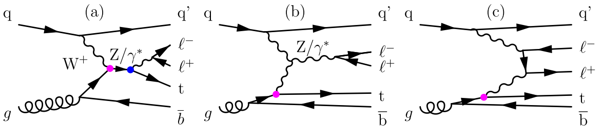
Fig. 44. Example Feynman diagrams for the production of tZq .
