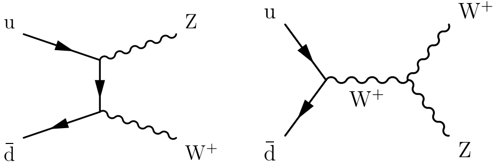
Fig. 20. Feynman diagrams for WZ diboson production. Shown are radiative production (left), where the vector bosons are radiated off a quark, and a TGC production (right), where a W boson is created by q\bar{q} annihilation and splits into W and Z bosons. These diagrams are representative of all diboson production mechanisms that involve radiative or TGC processes. In the case of neutral final states TGCs are forbidden in the SM and only anomalous coupling due to new physics could lead to contributions from that type of diagram.
