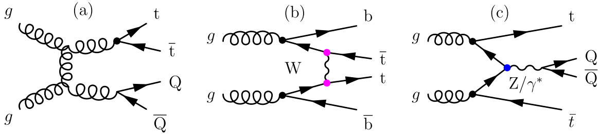
Fig. 47. Feynman diagrams contributing to the associated production of top quarks with heavy-flavoured jets.
