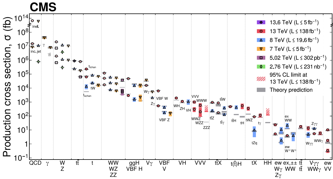
Fig. 1. Cross sections of selected high-energy processes measured by the CMS experiment. Measurements performed at different LHC pp collision energies are marked by unique symbols and the coloured bands indicate the combined statistical and systematic uncertainty of the measurement. Grey bands indicate the uncertainty of the corresponding SM theory predictions. Shaded hashed bars indicate the excluded cross section region for a production process with the measured 95% CL upper limit on the process indicated by the solid line of the same colour.
