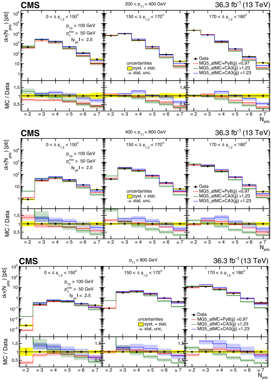
Fig. 4. Differential cross section of jet production as a function of the exclusive jet multiplicity (inclusive for 7 jets) in bins of p_T and \Delta\phi_{12} . The data are compared with the NLO dijet predictions from MADGRAPH5_aMC@NLO: MG5_aMC+Py8 (jj) and MG5_aMC+CA3 (jj), as well as the NLO three-jet prediction of MG5_aMC+CA3 (jjj), where parton showering is performed by PYTHIA 8 (Py8) and CASCADE3 [88] (CA3). The vertical error bars correspond to the statistical uncertainty, the yellow band shows the total experimental uncertainty. The shaded bands show the uncertainty from a variation of the renormalization and factorization scales. The predictions are normalized to the measured inclusive dijet cross section using the scaling factors shown in the legend.
