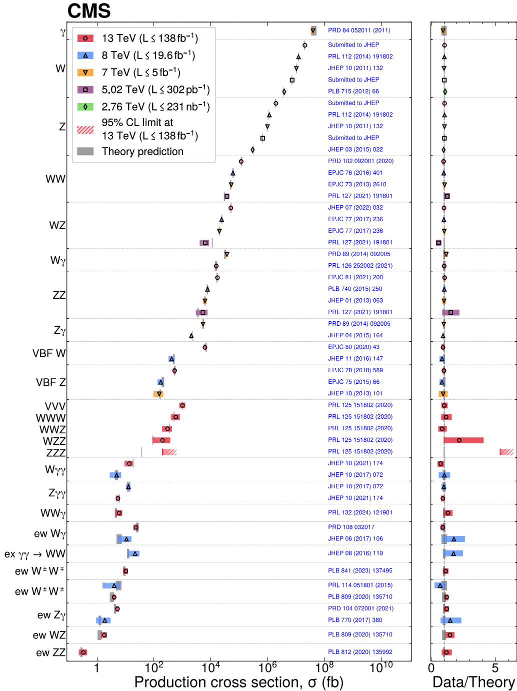
Fig. 63. Summary of electroweak cross section measurements. Measurements performed at different LHC pp collision energies are marked by unique symbols and the coloured bands indicate the combined statistical and systematic uncertainty of the measurement. Grey bands indicate the uncertainty of the corresponding SM theory predictions. Shaded hashed bars indicate the excluded cross section region for a production process with the measured 95% C.L. upper limit on the process indicated by the solid line of the same colour.
