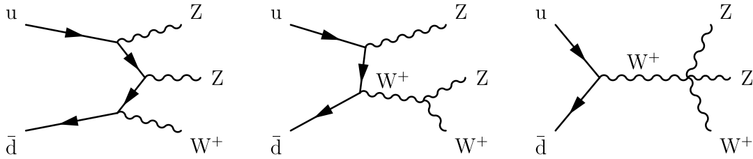
Fig. 28. Triboson WZZ production via diagrams involving radiative production (left), TGCs (centre), and QGCs (right). This set of triboson Feynman diagrams is representative of most triboson signatures, with the caveat that neutral TGCs and some QGC combinations are not allowed in the SM.
