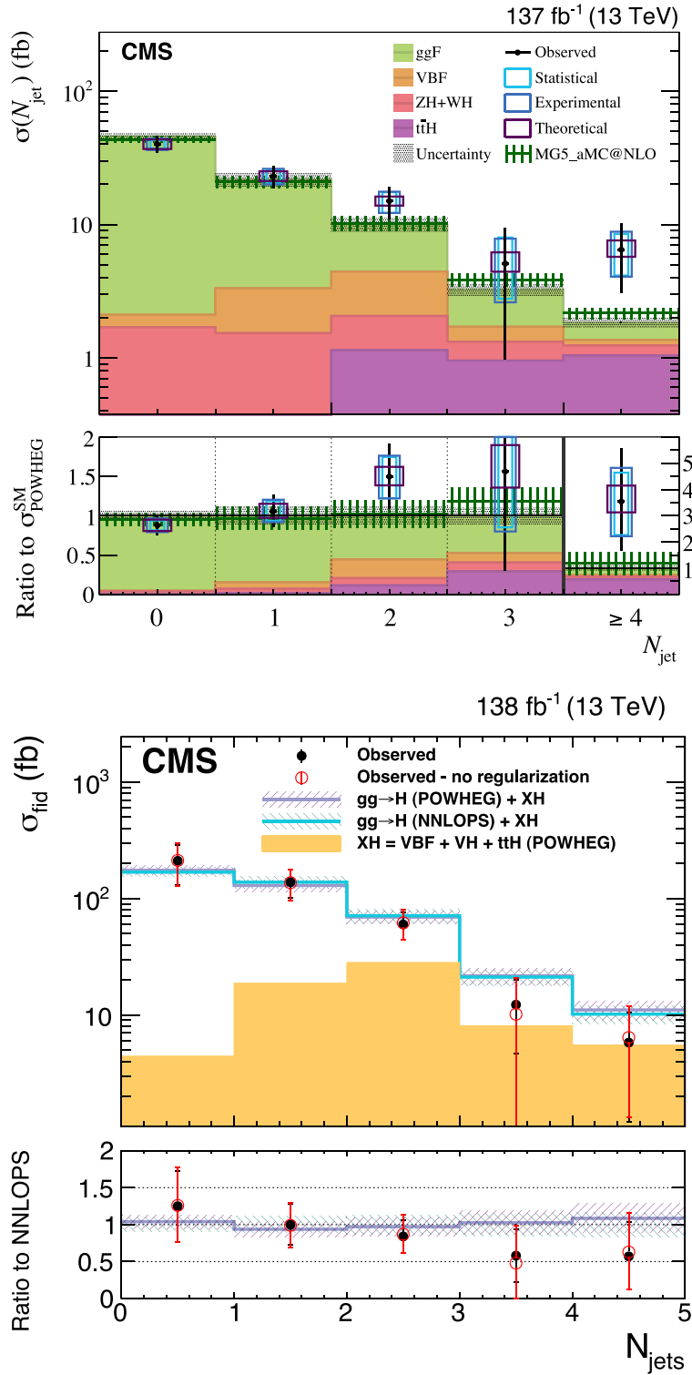
Fig. 59. Differential fiducial cross sections for Higgs boson production as functions of the number of jets in the event, for the H \rightarrow WW [546] (upper) and H \rightarrow \tau\tau [545] (lower) decay modes. Source: Figure compiled from Refs. [543,554].
