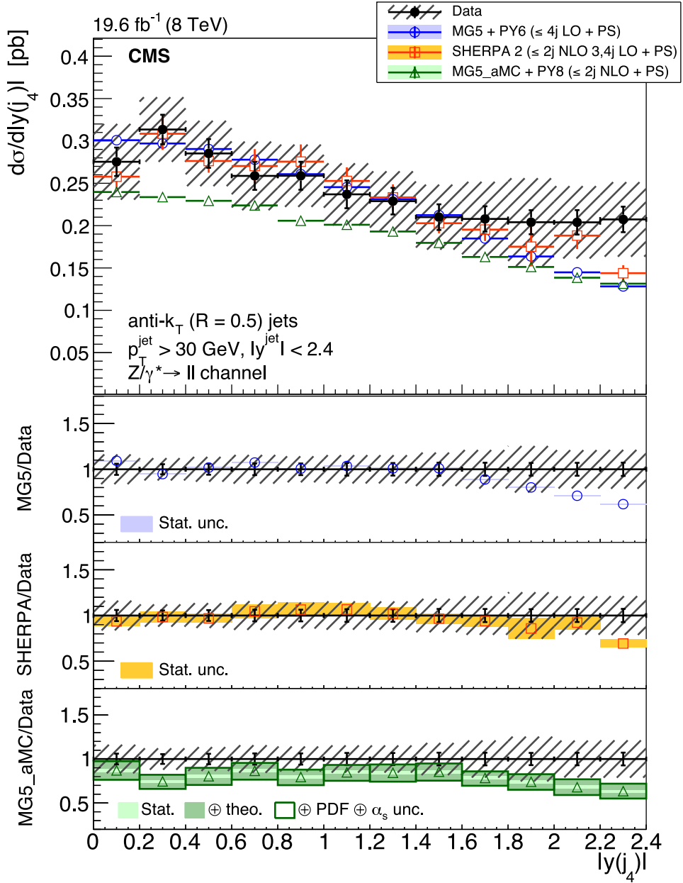
Fig. 17. The differential cross section for Z \rightarrow \ell^+ \ell^- + \text{jets} production as a function of the absolute value of the 4th jet's rapidity compared with the predictions calculated with MADGRAPH 5+PYTHIA 6, SHERPA 2, and MG5_aMC +PYTHIA 8. The lower panels show the ratios of the theoretical predictions to the measurements. Error bars around the experimental points show the statistical uncertainty and the cross-hatched bands indicate the statistical and systematic uncertainties added in quadrature. The boxes around the MG5_aMC + PYTHIA 8 to measurement ratio represent the uncertainty in the prediction, including statistical, theoretical (from scale variations), and PDF uncertainties. The dark green area represents the statistical and theoretical uncertainties only and the light green area represents the statistical uncertainty alone.
