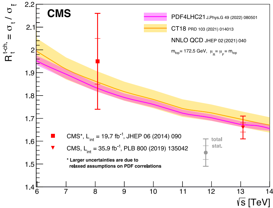
Fig. 36. Summary of the CMS measurements of R_t = \sigma_t / \sigma_{\bar{t}} , the cross section ratio between t -channel top quark and t -channel top antiquark production. The measurements are compared with NNLO QCD calculations using the PDF sets CT18 and PDF4LHC21. The coloured bands represent the uncertainties in the theoretical predictions (scale and PDF uncertainties). The PDF uncertainties are estimated using the PDF4LHC21 prescription [399].
