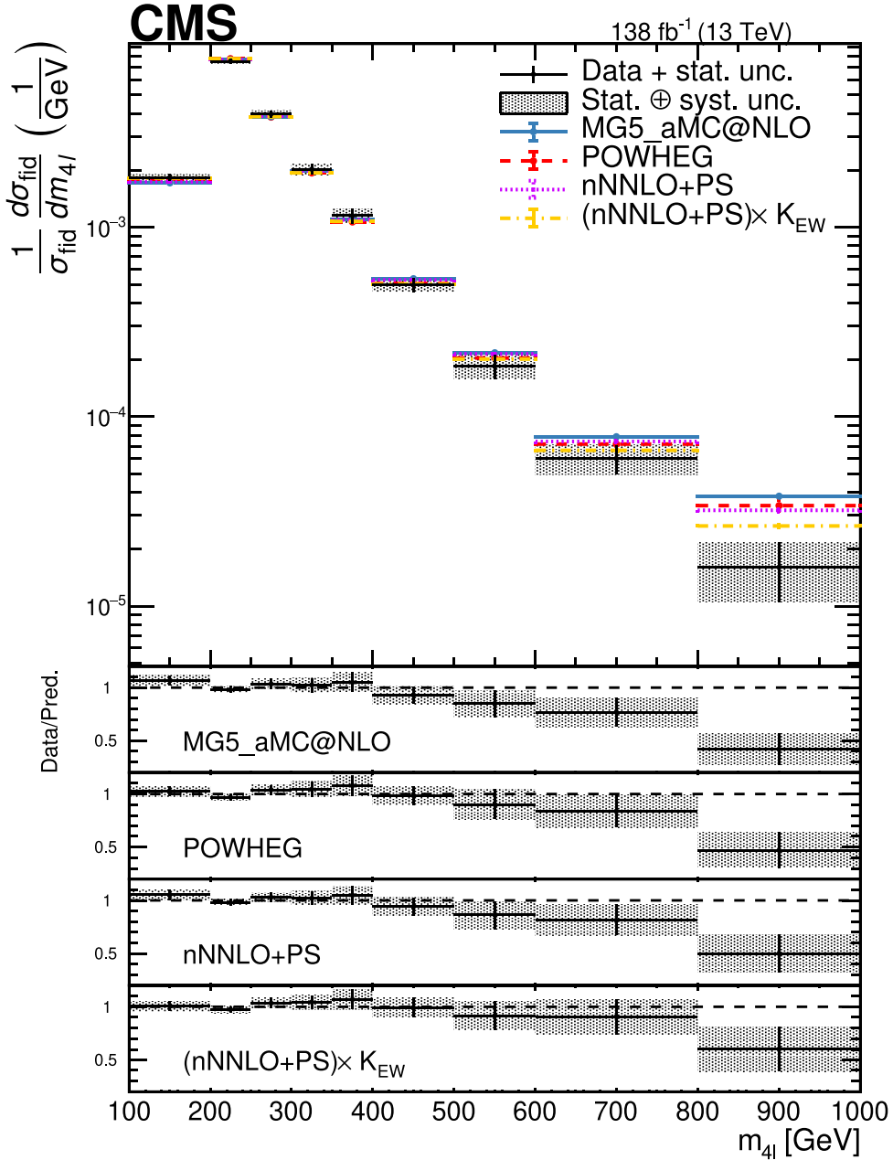
Fig. 25. Differential cross section normalized to the fiducial cross section as a function of m_{4\ell} . The on-shell Z requirement 60 < m_Z < 120 GeV is applied for both Z boson candidates. Points represent the unfolded data, the solid lines the (MADGRAPH5_aMC@NLO q\bar{q} \rightarrow ZZ ) + (MCFM g g \rightarrow ZZ ) + (POWHEG H \rightarrow ZZ ) predictions, and red dashed lines the (POWHEG q\bar{q} \rightarrow ZZ ) + (MCFM g g \rightarrow ZZ ) + (POWHEG H \rightarrow ZZ ) predictions. The MADGRAPH5_aMC@NLO EW ZZ predictions are included. The purple dashed lines represent the nNNLO+PS predictions, and the yellow dashed lines represent the nNNLO+PS prediction with EW corrections applied. Vertical bars on the MC predictions represent the statistical uncertainties. The lower panels show the ratio of the measured to the predicted cross sections. The shaded areas represent the full uncertainties calculated as the sum in quadrature of the statistical and systematic uncertainties and the vertical bars around the data points represent the statistical uncertainties only. The overflow events are included in the last bin of the distributions.
