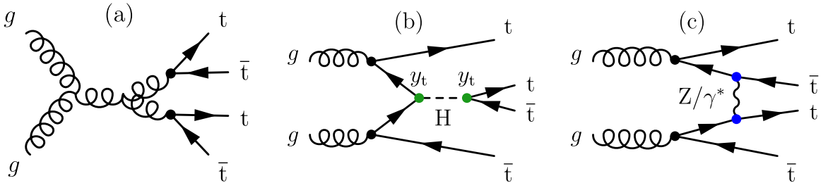
Fig. 49. Representation of different Feynman diagrams contributing to t\bar{t}t\bar{t} production at the LHC. Diagrams that involve strong coupling vertices, shown in (a), are expected to dominate.
