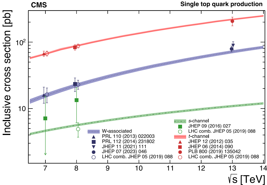
Fig. 35. Single top quark cross section summary of CMS measurements as a function of the pp centre-of-mass energy. Where available the results from the full LHC combination are also overlaid for comparison. The theoretical calculations for t -channel, s -channel, and W -associated production are from Refs. [386–389].
