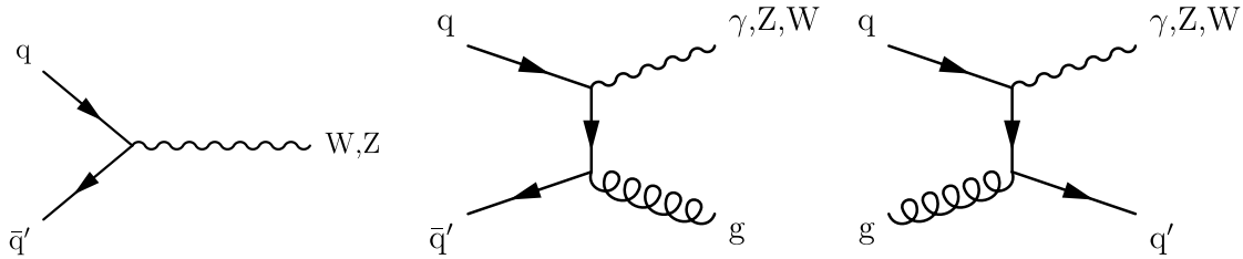
Fig. 10. The Feynman diagram for Drell–Yan production of W and Z bosons (left). The Z boson production process involves annihilation of quark–antiquark pairs of same flavour. The W boson production process requires different-flavour quarks, such as u\bar{d} or \bar{u}d pairs. The NLO diagrams with real emission of a jet for the production of single vector bosons and one jet with a final-state gluon jet (middle) or quark jet (right).
