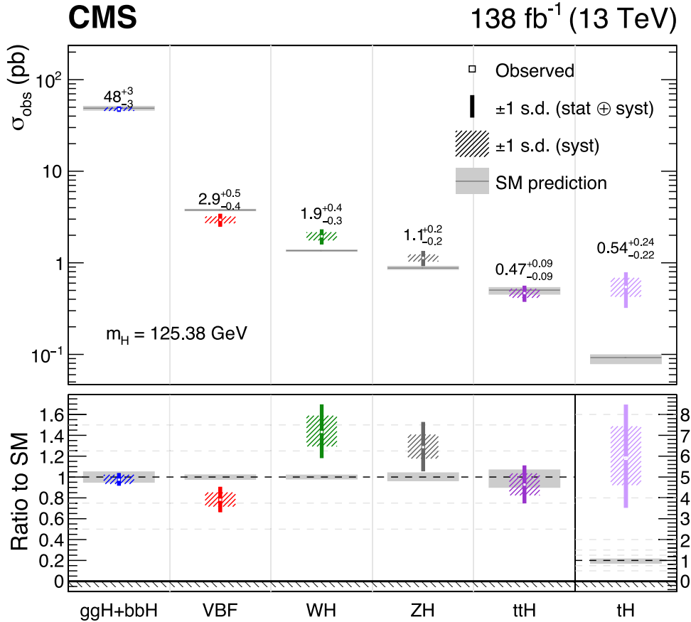
Fig. 56. Measured cross sections for the main Higgs boson production modes. The best fit cross sections are plotted together with the respective 68% confidence level intervals. The systematic components of the uncertainty in each parameter are shown by the coloured boxes. The grey boxes indicate the theoretical uncertainties in the SM predictions. The lower panel shows the ratio of the fitted values to the SM predictions.
