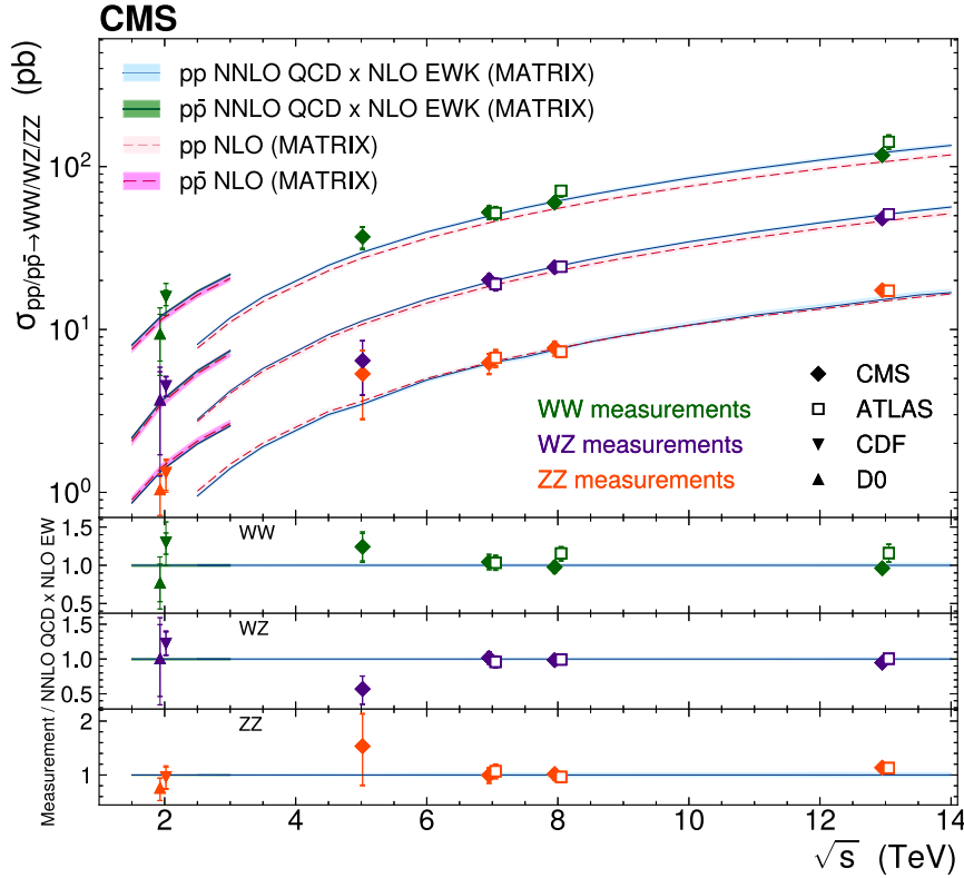
Fig. 23. The total W^+W^- , WZ and ZZ cross sections as functions of the pp centre-of-mass energy. Results from the CMS and ATLAS experiments for pp collisions are compared with the predictions from MATRIX at NNLO in QCD and NLO in EW, and at NLO in QCD. Also shown are results from p\bar{p} collisions at the CDF and D0 experiments compared with MATRIX predictions as above. The inner vertical errors bars around the experimental data points show the statistical uncertainties of the measurements, whereas the outer bars show the total uncertainties. Measurements at the same centre-of-mass energy are shifted slightly along the horizontal axis for clarity.
