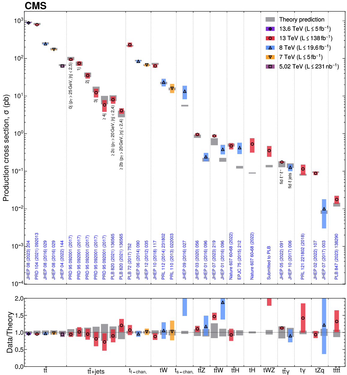
Fig. 53. Summary of production cross section measurements involving top quarks. Measurements performed at different LHC pp collision energies are marked by unique symbols and the coloured bands indicate the combined statistical and systematic uncertainty of the measurement. Grey bands indicate the uncertainty of the corresponding SM theory predictions. Shaded hashed bars indicate the excluded cross section region for a production process with the measured 95% C.L. upper limit on the process indicated by the solid line of the same colour.
