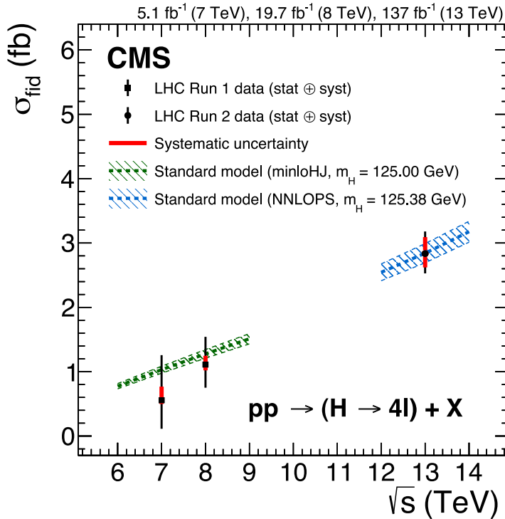
Fig. 57. The measured inclusive fiducial cross section for H \rightarrow ZZ \rightarrow 4\ell as a function of \sqrt{s} . The acceptance is calculated using HRes [547,548] at 7 and 8 TeV, and POWHEG at 13 TeV, and the total gluon fusion cross section and uncertainty are taken from Ref. [549]. The SM predictions and measurements are calculated at m_H = 125.0 GeV for \sqrt{s} = 6 –9 TeV, and at m_H = 125.38 GeV for 12–14 TeV. Source: Figure taken from Ref. [509].
