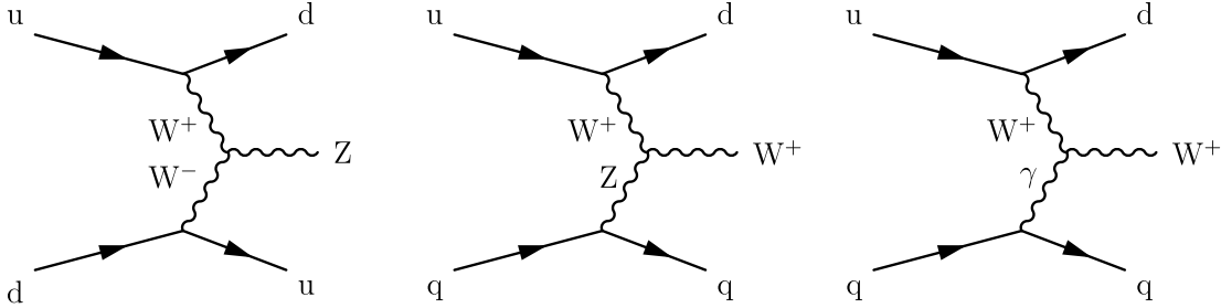
Fig. 31. Feynman diagrams for vector boson fusion production of z (left) and w bosons (middle) via the WWZ TGC vertex and w via the WW \gamma TGC vertex (right).
