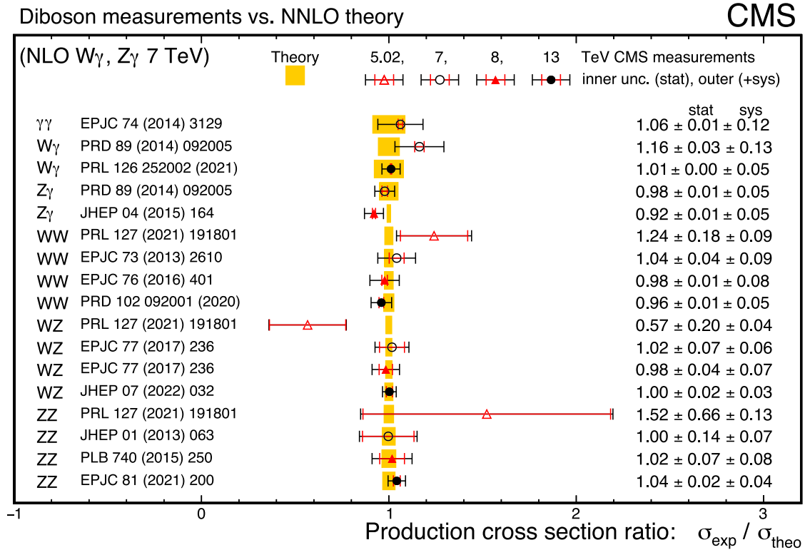
Fig. 22. Summary of cross section measurements for diboson production shown as a ratio over the NNLO or NLO QCD predictions. The yellow bands indicate the uncertainties in the theoretical predictions and the error bars on the points are the statistical uncertainties, whereas the outer bars are the combined statistical and systematic uncertainties.
