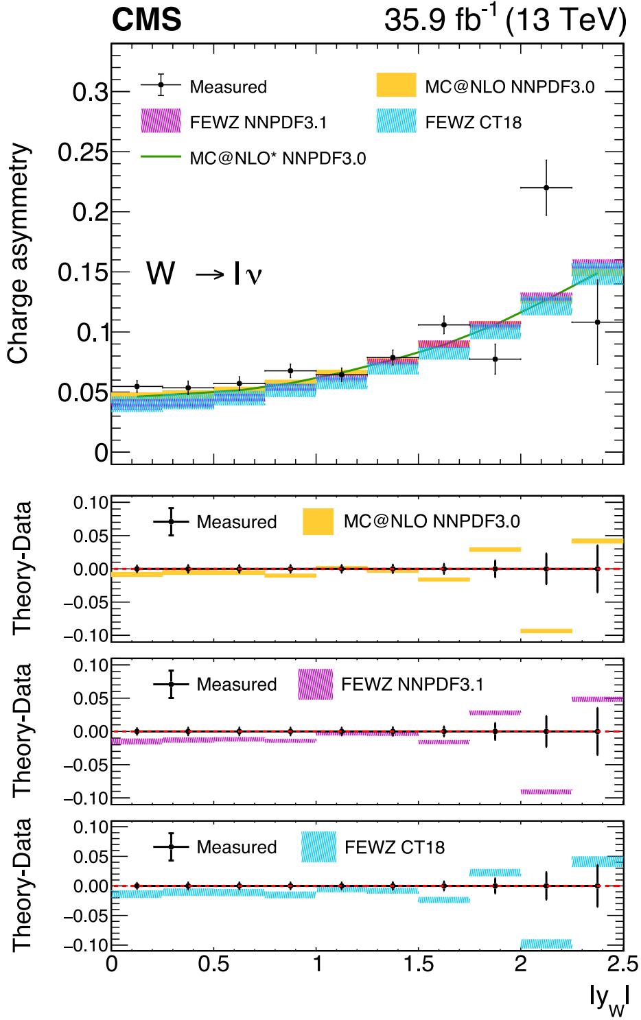
Fig. 15. Measured W boson charge asymmetry as a function of |y_W| from the combination of the electron and muon channels (black dots), compared with different theoretical predictions. The vertical errors bars around the experimental data points show the total uncertainty of the measurements. The yellow band represents the default generator used in this analysis, MG5_aMC with the NNPDF3.0 PDF set, the pink band represents the FEWZ generator with the NNPDF3.1 PDF set, and the cyan band represents the FEWZ generator with the CT18 PDF set. The uncertainty bands of the prediction include the PDF uncertainties only, which are dominant with respect to \alpha_s , or renormalization and factorization scale variations for this quantity.
