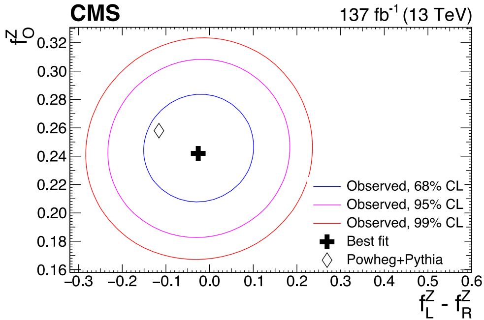
Fig. 26. Confidence regions in the f_0^Z vs f_L^Z - f_R^Z parameter plane for the Z boson polarization. The results are obtained with no additional requirement for the charge of the W boson. The blue, magenta, and red contours present the 68, 95, and 99% confidence levels, respectively. The cross indicates the best fit to the observed data and the diamond shows the result of the POWHEG + PYTHIA simulation.
