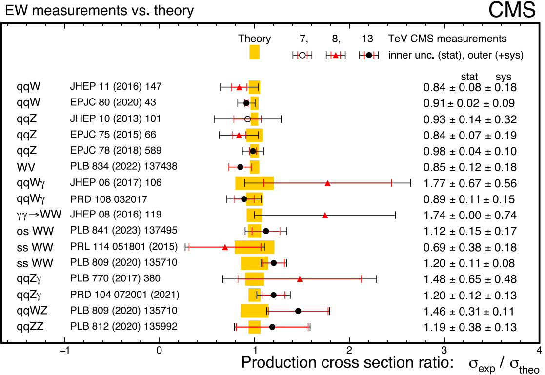
Fig. 33. Summary of cross section measurements of EW single or diboson production processes including vector boson fusion, vector boson scattering, and scattering via exclusive processes. Production of pairs of W bosons can occur in same-sign (ss) W^{\pm}W^{\pm} , opposite-sign (os), W^{\pm}W^{\mp} , or exclusive production where photons are radiated from the incoming protons and form W^{\pm}W^{\mp} pairs via EW scattering. Results are displayed as a ratio of the experimental measurement over the SM prediction. The yellow bands indicate the uncertainties in the theoretical predictions and the error bars on the points are the experimental uncertainties, with the outer bar being the combined statistical and systematic uncertainty.
