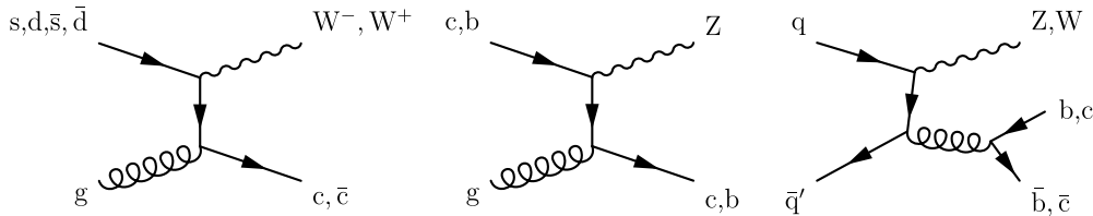
Fig. 19. Production of W or Z bosons with heavy-flavour quarks. Examples of lowest order Feynman diagrams include W + charm (left), Z + charm or bottom (middle), W or Z production with two heavy-flavour quarks (right).
