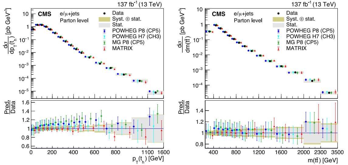
Fig. 40. Differential cross sections at the parton level as a function of the hadronically decaying top quark p_T (left) and of the t\bar{t} invariant mass (right). The analysis was performed using t\bar{t} events in the \ell +jets final state. The data are shown as points with grey (yellow) bands indicating the statistical (statistical and systematic) uncertainties. The cross sections are compared with the predictions of POWHEG combined with PYTHIA (P8) or HERWIG (H7), the multiparton simulation MADGRAPH5_aMC@NLO (MG)+PYTHIA FxFx, and the NNLO QCD calculations obtained with MATRIX. The error bars represent the theory uncertainty in the predictions. The ratios of the various predictions to the measured cross sections are shown in the lower panels.
