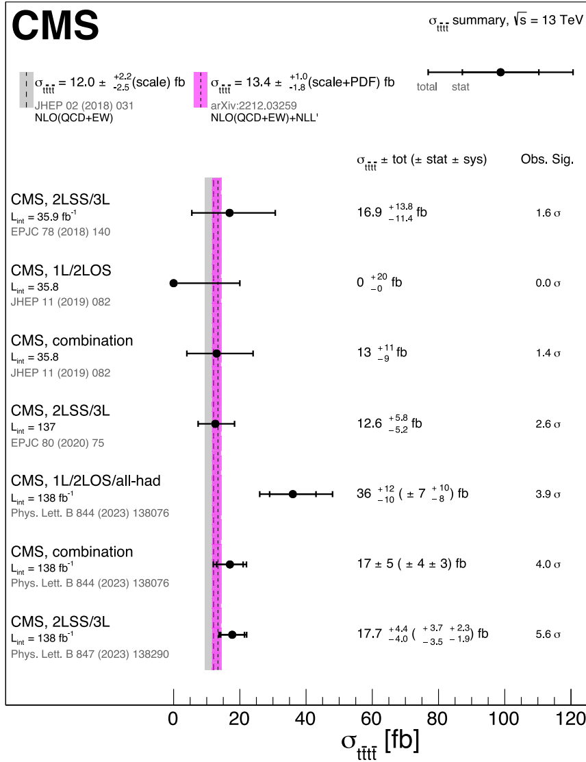
Fig. 50. Summary of CMS measurements of the t\bar{t}\bar{t} production cross section at 13 TeV in various channels. The total (statistical) uncertainty associated with the measurements is represented by the outer (inner) error bars. The cross section measurements are compared with the NLO QCD and EW theoretical calculation. The theoretical band represents uncertainties due to renormalization and factorization scales. Complementary theory predictions are also available in Ref. [493].
