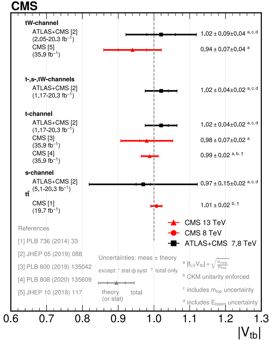
Fig. 52. Summary of |V_{tb}| determinations from top quark events using different techniques. The values measured and the corresponding references are given in the figures. The error bars represent separately different uncertainties, as described in the legend. In the LHC combinations, the reference theory cross section used in the t - and s -channel measurements is computed at NLO QCD accuracy [387] with the PDF4LHC prescription for the PDF uncertainty using CT10nlo, MCSTW2008nlo, and NNPDF2.3nlo [500], whereas in the tW channel the theory reference is computed at NNLO+NNLL QCD accuracy [501] using the MSTW2008 NNLO PDF [112]. A line at |V_{tb}| = 1 is used as a common reference.
