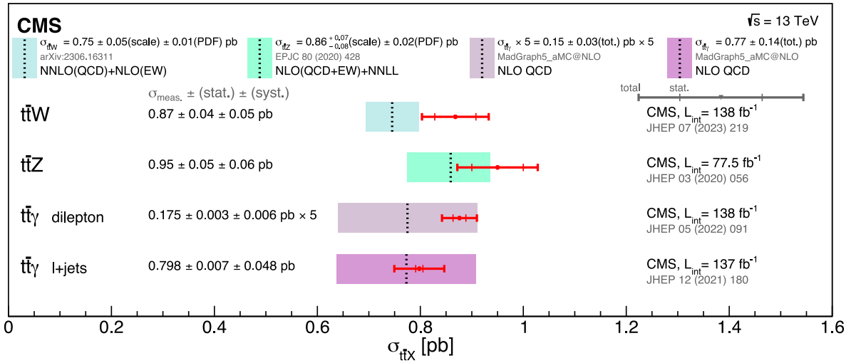
Fig. 45. Summary of CMS t\bar{t}W and t\bar{t}V^0 cross section measurements with respect to the SM prediction. The horizontal bars display separately the statistical and the total uncertainties of the experimental measurements. The uncertainty associated to the theory predictions is represented by shaded bands and includes the variations of the renormalization and factorization scales and parton density functions.
