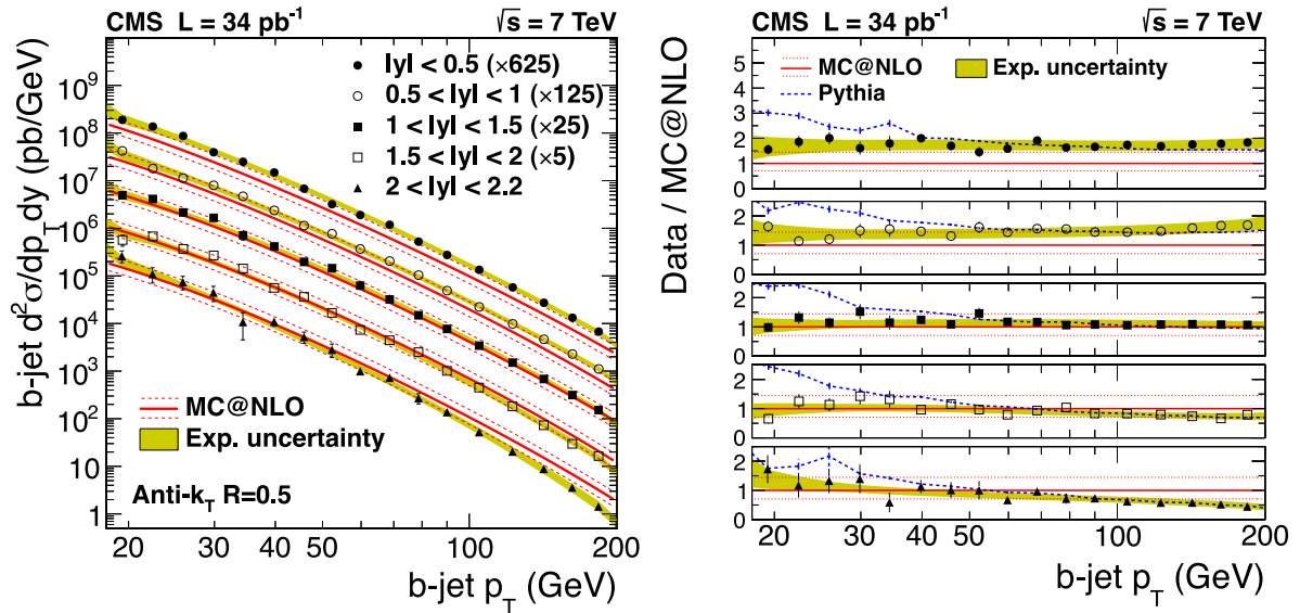
Fig. 5. Measured b jet cross section from the jet analysis, multiplied by the arbitrary factors shown in the figure for easier viewing, compared to the MC@NLO calculation (left) and as a ratio to the MC@NLO calculation (right). The experimental systematic uncertainties are shown as a shaded band and the statistical uncertainties as error bars. The MC@NLO uncertainty is shown as dotted lines. The PYTHIA prediction is also shown in the right panel.
