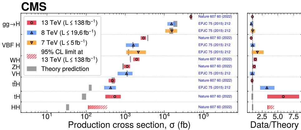
Fig. 66. Summary of Higgs boson production cross section measurements.
