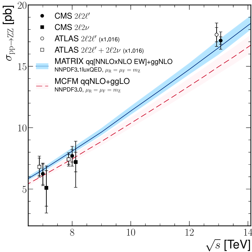
Fig. 24. The total ZZ cross section as a function of the pp centre-of-mass energy. Results from the CMS and ATLAS [315–317] experiments are compared with the predictions from MATRIX and MCFM, as described in the text. The ATLAS measurements were performed with a Z boson mass window of 66–116 GeV, instead of 60–120 GeV used by CMS, and are corrected for the resulting 1.6% difference in acceptance. The inner vertical errors bars around the experimental data points show the statistical uncertainties of the measurements, whereas the outer bars show the total uncertainties. Measurements at the same centre-of-mass energy are shifted slightly along the horizontal axis for clarity.
