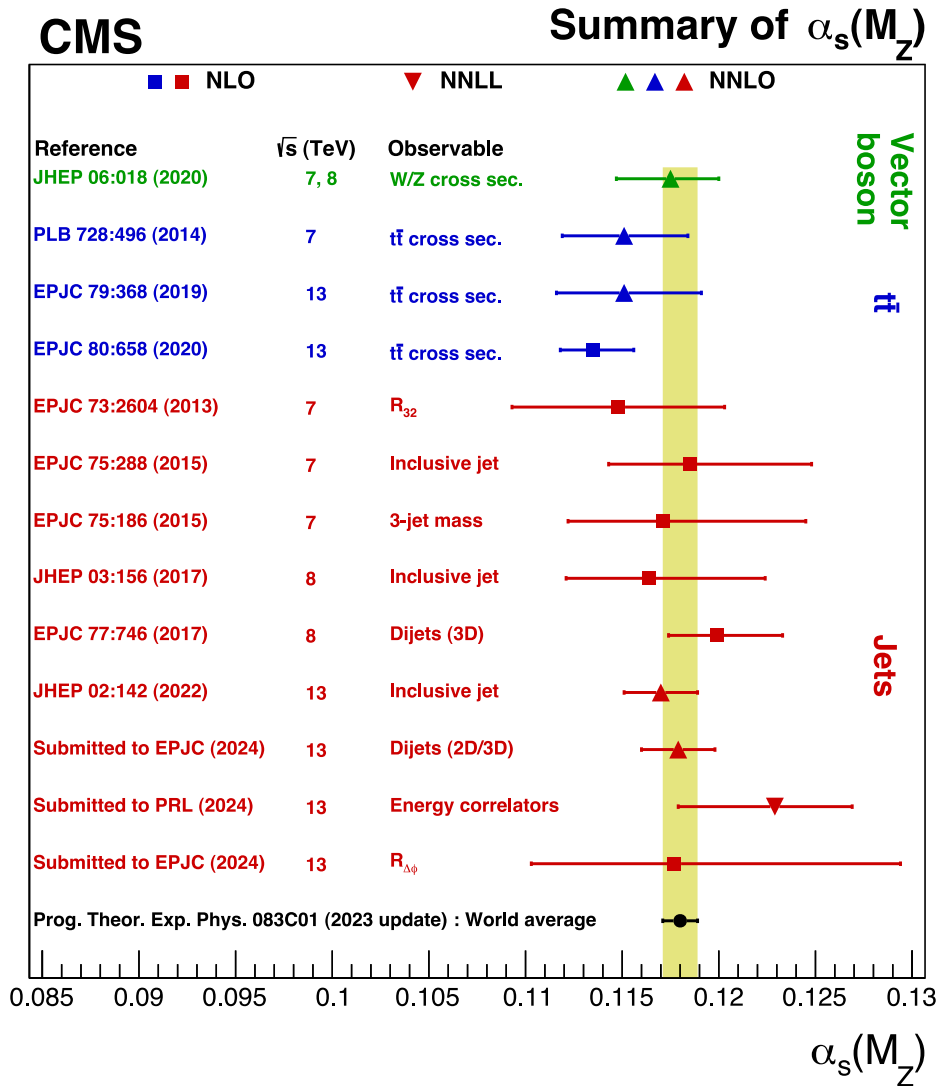
Fig. 7. A summary of \alpha_s(m_Z) extractions from the CMS experiment compared with the 2023 PDG world-average. For each measurement, p\bar{p} collision energy and the QCD perturbative order of the \alpha_s(m_Z) extraction are listed. Results are grouped by the type of the final state used: vector boson, t\bar{t} , and jets.
