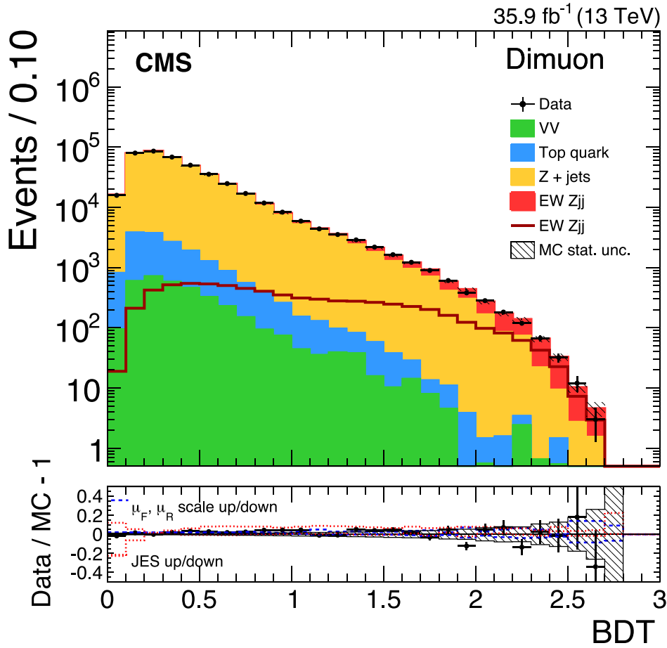
Fig. 32. Distribution for a BDT discriminant used to select VBF Z events in dimuon events. The contributions from the different background sources and the signal are shown stacked, with data points superimposed. The vertical errors bars around the experimental data points show the total uncertainties. The expected signal-only contribution is also shown as an open histogram. The lower panel shows the relative difference between the data and expectations, as well as the uncertainty envelopes for the jet energy scale, and renormalization and factorization scale uncertainties.
