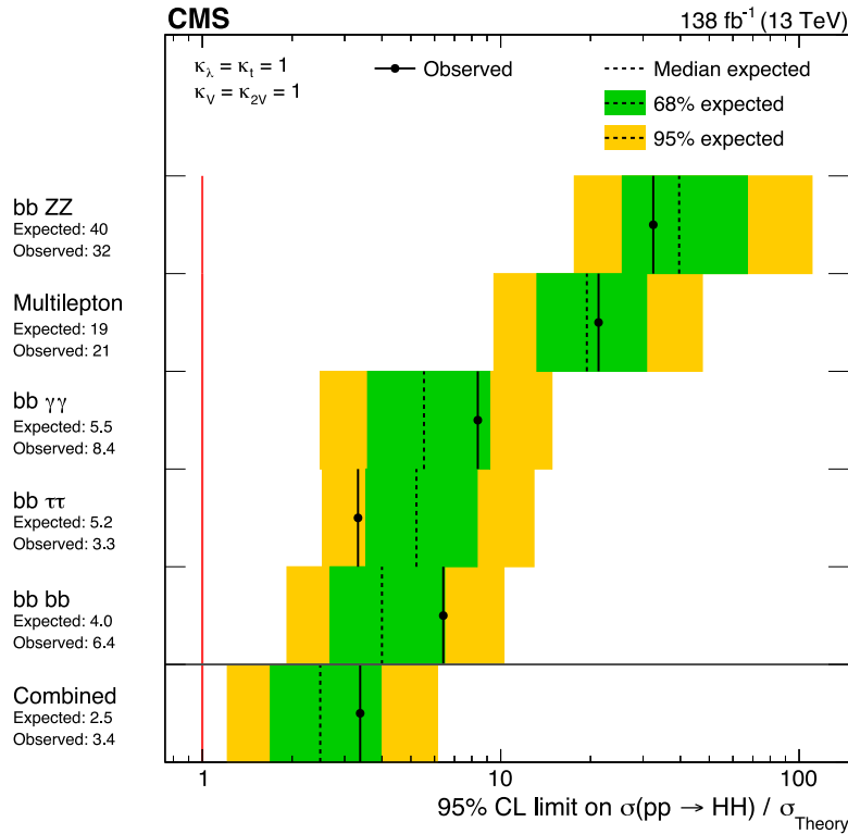
Fig. 62. The expected and observed upper limits on the production of Higgs boson pairs. The results are expressed as a ratio to the SM prediction for the cross section ( \sigma(pp \rightarrow HH)/\sigma_{\text{SM}} ). A vertical red line at \sigma(pp \rightarrow HH)/\sigma_{\text{SM}} = 1 is drawn to guide the eye. The search modes are ordered, from upper to lower, by their expected sensitivities from the least to the most sensitive. The overall combination of all searches is shown by the lowest entry.
