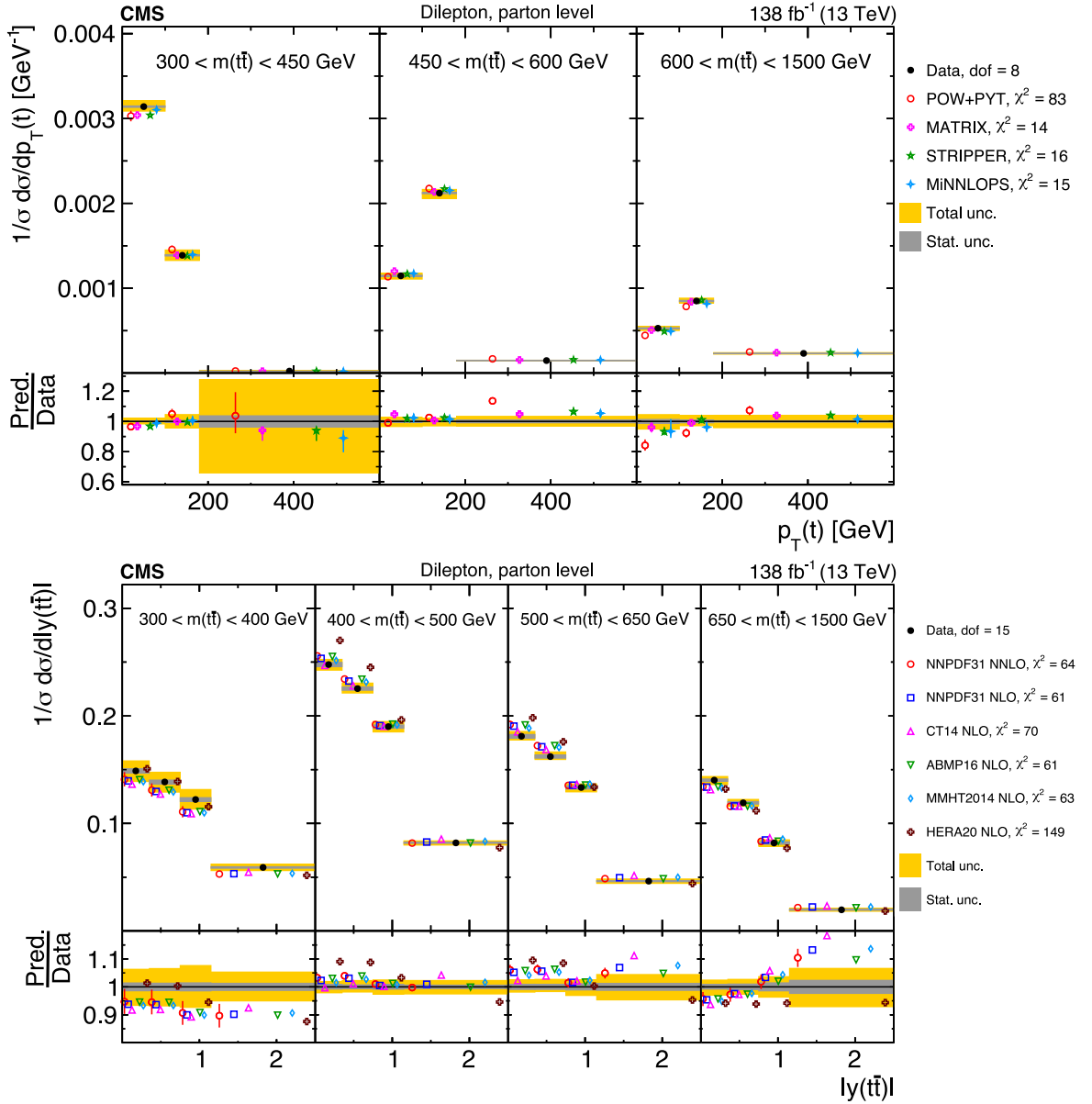
Fig. 41. Normalized differential cross sections as a function of p_T(t) in bins of m(t\bar{t}) (upper), and as a function of y(t\bar{t}) in bins of m(t\bar{t}) (lower). The data, shown as bullets with grey and yellow bands indicating the statistical and total uncertainties, are compared with the prediction from POWHEG+PYTHIA 8 and various theoretical predictions (see text). The error bars represent the theory uncertainty in some of the predictions. The lower panel in each figure shows the ratios of the predictions to the data.
