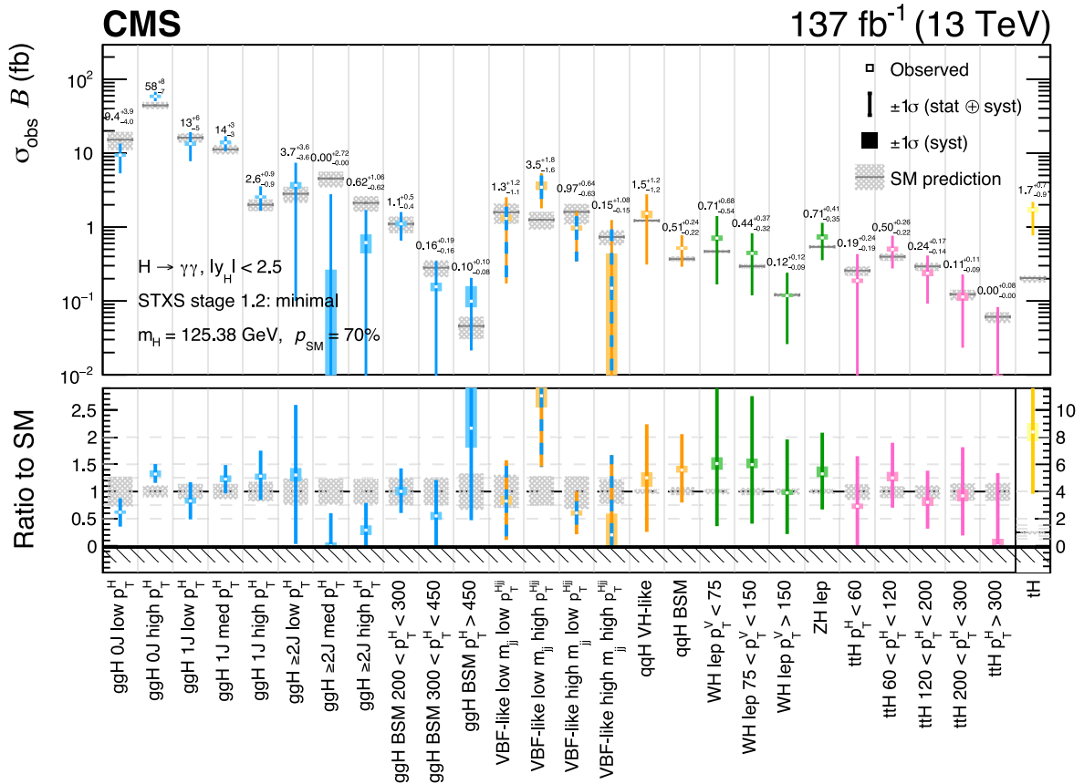
Fig. 61. Observed results of the minimal merging scheme STXS fit for H \rightarrow \gamma\gamma at 13 TeV. The best fit cross sections are plotted together with the respective 68% confidence level intervals.
