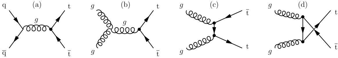
Fig. 37. Leading order Feynman diagrams for t\bar{t} production.
