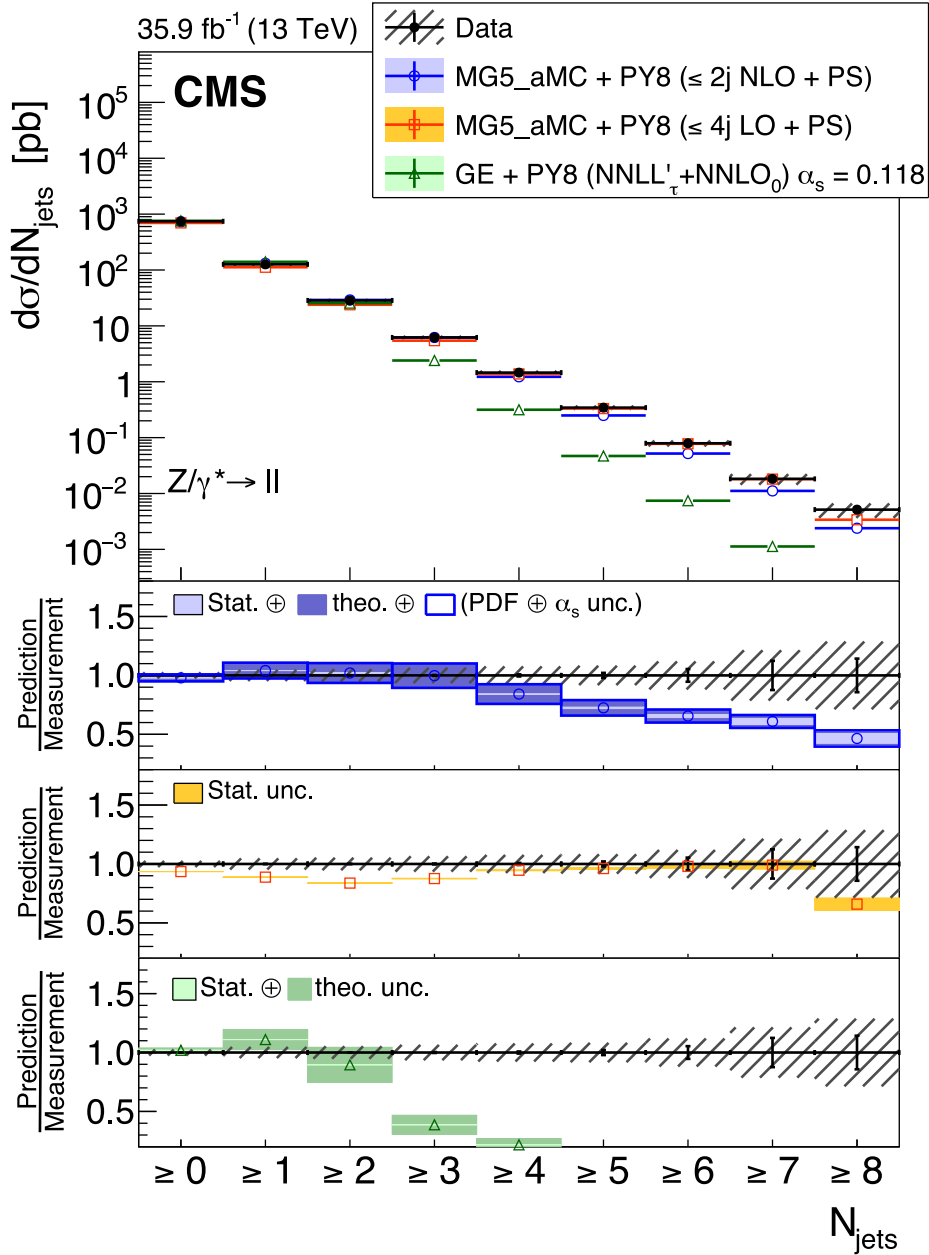
Fig. 16. The differential cross section of Z \rightarrow \ell^+ \ell^- + \text{jets} production as a function of inclusive jet multiplicity, compared with the predictions calculated with MADGRAPH5_aMC@NLO (LO) + PYTHIA 8, MADGRAPH5_aMC@NLO (NLO) + PYTHIA 8, and GENEVA. The lower panels show the ratios of the theoretical predictions to the measurements. The measurement statistical (systematic) uncertainties are presented with vertical error bars (hashed areas). The boxes around the MADGRAPH5_aMC@NLO (NLO) + PYTHIA 8 to measurement ratio represent the uncertainty in the prediction as listed in the legend.
