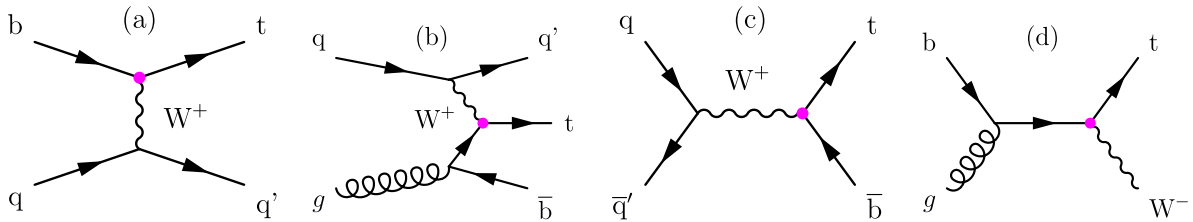
Fig. 34. Feynman diagrams illustrating the pure EW contributions to single top quark production at the LHC at Born level. Charge conjugate states are implied. From left to right: the t -channel production, (a) with and (b) without a b quark in the initial state; (c) the s -channel; and (d) the tW -production. In all diagrams the tWq vertex is marked with a purple dot.
