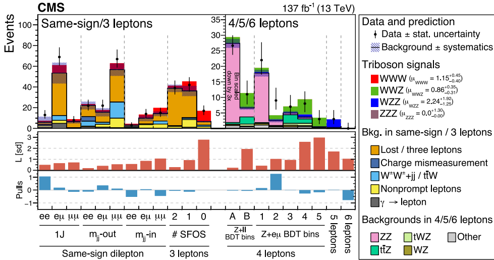
Fig. 29. Comparison of the observed numbers of events to the predicted yields. For the WWW and WWZ channels, the results from boosted decision tree (BDT) based selections are used. For the other results different categorizations based on the number of jets, whether dijet masses are inside or outside a selection window used to identify the boson, and specific lepton combinations or the number of same-flavour, opposite-sign (SFOS) leptons are shown. The VVV signal is shown stacked on top of the total background. The points represent the data and the error bars show the statistical uncertainties. The expected significance L in the middle panel represents the number of standard deviations (sd) with which the null hypothesis (no signal) is rejected. The lower panel shows the pulls for the fit result.
