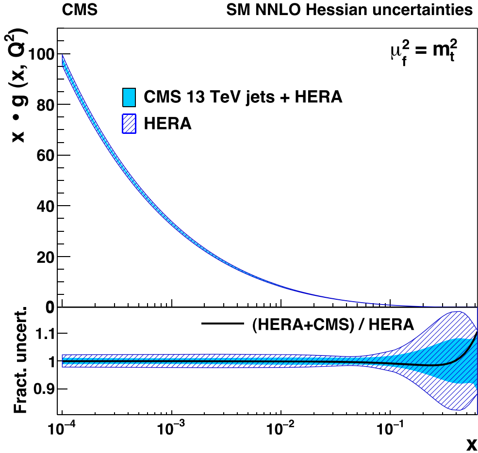
Fig. 6. The gluon distribution, shown as a function of x for the factorization scale \mu_f = m_t . The filled (hatched) band represents the results of the NNLO fit using HERA DIS and the CMS inclusive jet cross section at \sqrt{s} = 13 TeV (using the HERA DIS data only). The PDFs are shown with their total uncertainty. In the lower panel, the comparison of the relative PDF uncertainties is shown for each distribution. The solid line corresponds to the ratio of the central PDF values of the two variants of the fit.
