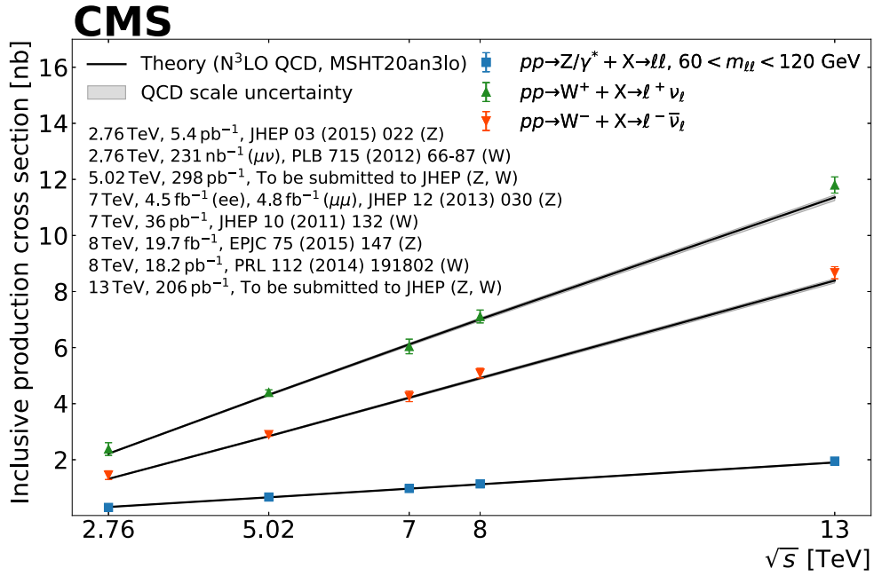
Fig. 12. Summary of the production cross section of weak gauge bosons, measured by CMS, plotted against the pp centre-of-mass energy ranging from 2.76 to 13 TeV. The error bars around the experimental data points represent the total uncertainty of the measurement. The measurements are compared with theoretical predictions (black lines) obtained at N 3 LO in QCD using the MSHT20an 3 LO PDF set. The grey band shows the envelope from renormalization and factorization scale variations.
