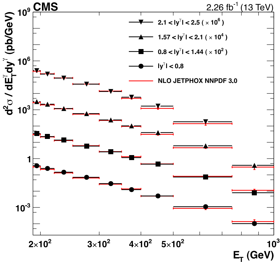
Fig. 11. Differential cross sections for isolated-photon production in four photon rapidity intervals. The points show the measured values and their total uncertainties; the lines represent the NLO JETPHOX predictions with the NNPDF3.0 PDF set.
