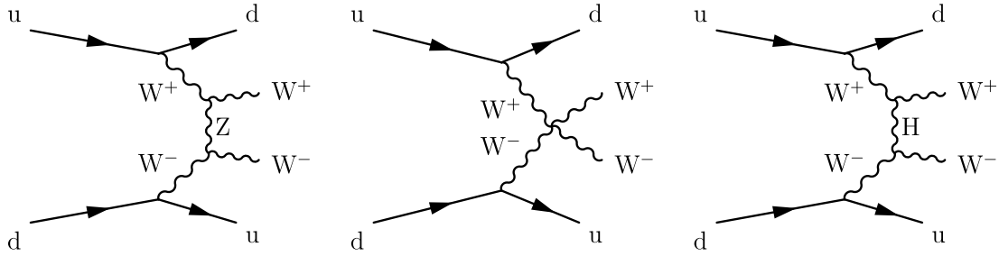
Fig. 30. Production of oppositely charged w bosons via vector boson scattering. Example Feynman diagrams include: scattering via z boson and two TGC vertices (left), a QGC vertex (middle), and scattering via a Higgs boson in t -channel (right).
