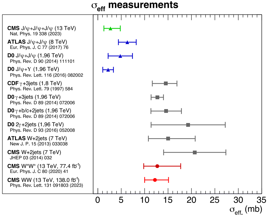
Fig. 9. Selected measurements of the effective DPS cross section in pp collisions at the LHC by the CMS and ATLAS experiments, and in p\bar{p} collisions at the Tevatron by the CDF and D0 experiments. The horizontal bars indicate the combined statistical and systematic uncertainty for each measurement.
