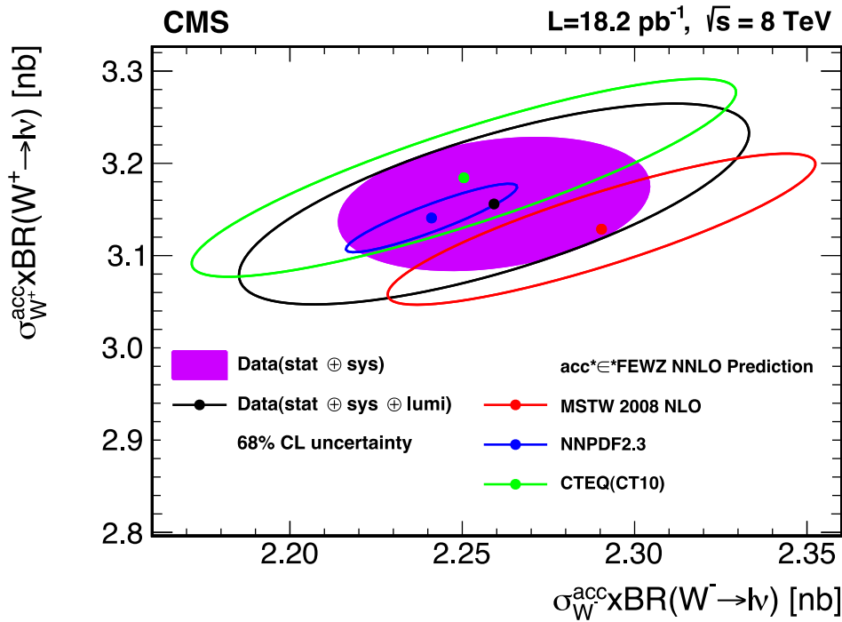
Fig. 14. Measured and predicted W^+ versus W^- production fiducial cross sections times branching fractions. The ellipses illustrate the 68% CL coverage for total uncertainties (open) and excluding the integrated luminosity uncertainty (filled). The uncertainties in the theoretical predictions correspond to the PDF uncertainty components only and are evaluated for three PDF sets: NNPDF2.3, CTEQ CT10, and MSTW 2008 NLO. Source: Figure taken from Ref. [231].
