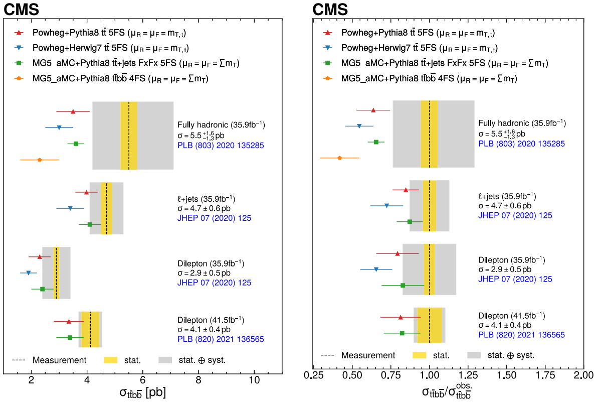
Fig. 48. Summary of t\bar{t}b\bar{b} cross section measurements. The left plot depicts the measurements performed in the full phase space using different final states and data sets, compared with different MC predictions. The right plot shows the ratio between the theoretical and measured cross. The statistical and total uncertainties on the measurements are represented by different shaded bands, while the uncertainty on the predictions are represented by error bars.
