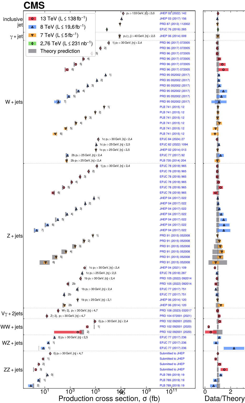
Fig. 64. Summary of measurements of jet cross sections and electroweak processes in association with jets.
