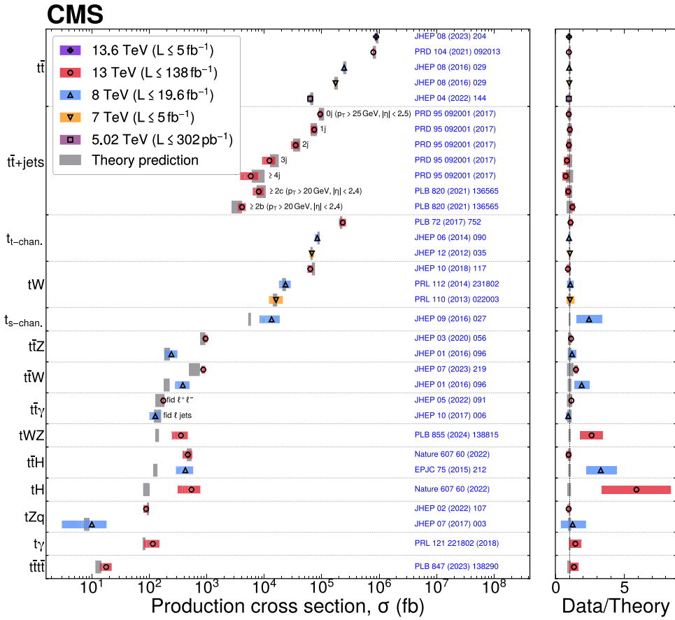
Fig. 65. Summary of top quark production cross section measurements.
