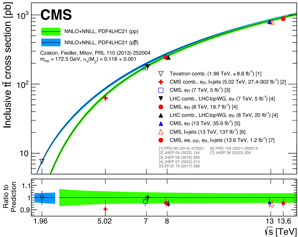
Fig. 38. Summary of top quark-antiquark pair cross section measurements by the CMS Collaboration in comparison with the theory calculation at NNLO+NNLL accuracy. The Tevatron measurements are also shown. The lower panel displays the ratio between the different measurements and the theory prediction. The coloured bands represent the theory uncertainty, while the error bars represent the uncertainty on the measurements.
