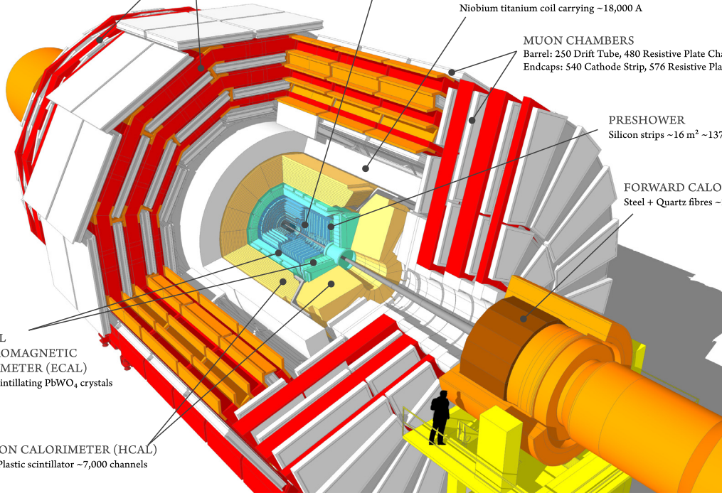
Fig. 2. The CMS detector for the data-taking period 2017–2018.
