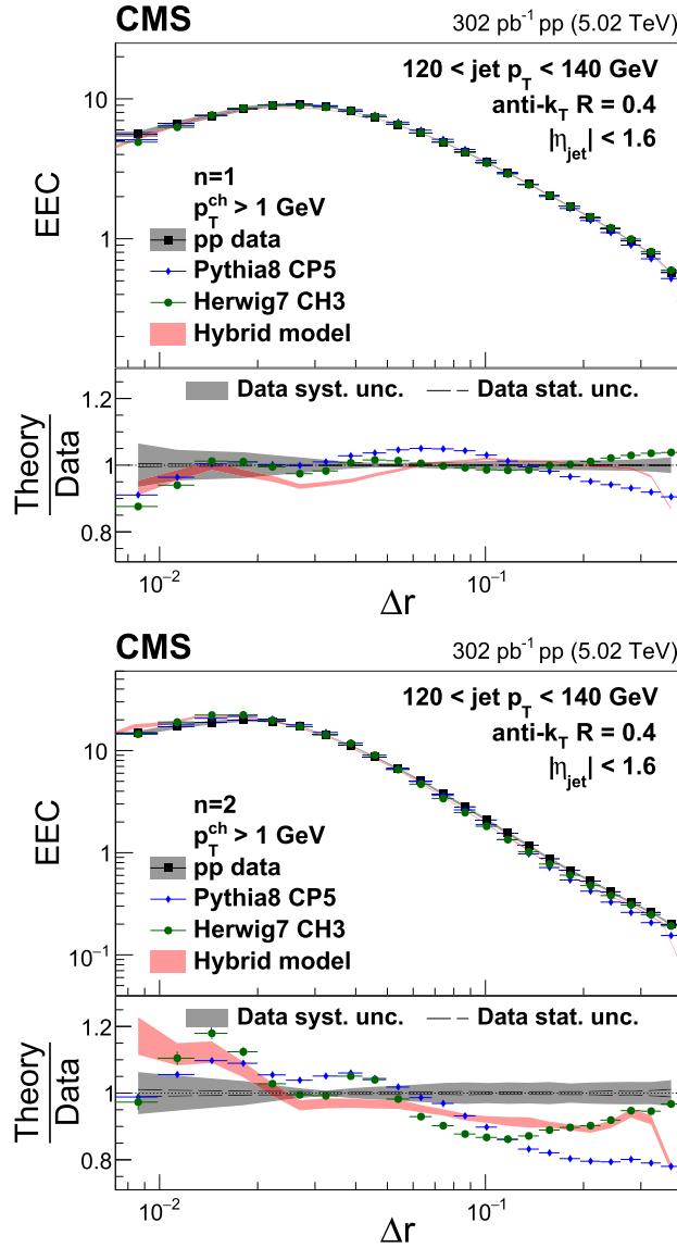
Fig. 6. Comparison of PYTHIA [58], HERWIG [61,62], and the hybrid model [82–84] calculations to the observed energy-energy correlators for p_T^{\text{ch}} > 1 GeV, 120 < p_{T,\text{jet}} < 140 GeV and n = 1 (upper) and n = 2 (lower) in pp collisions. In the lower panels, the experimental uncertainties are indicated by the bands around unity.
