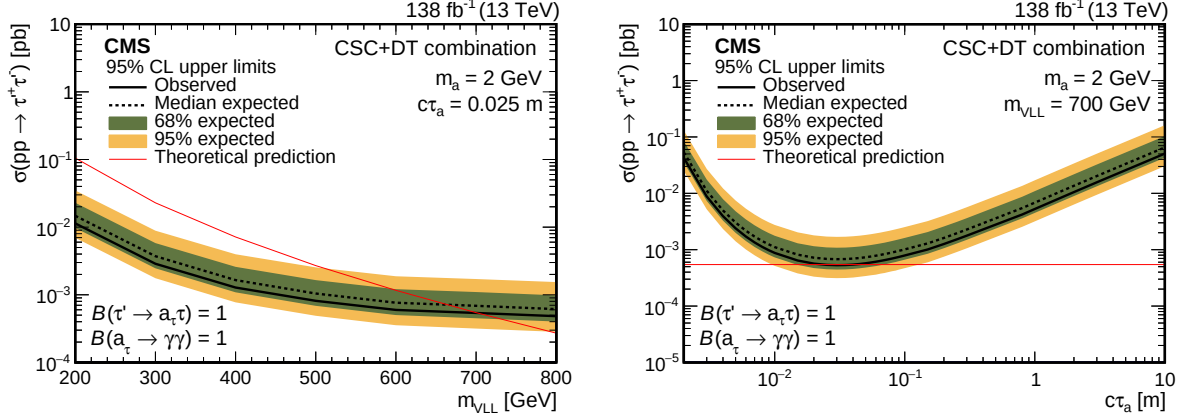
Figure 5: The 95% CL observed and expected upper limits on the VLL production cross section as a function of the VLL mass for the pseudoscalar boson mean proper decay length c\tau_a = 0.025 m (left), and as a function of c\tau_a for VLL mass of 700 GeV (right). The pseudoscalar boson mass is 2 GeV. The NLO theoretical prediction [36] is shown as a red line.
