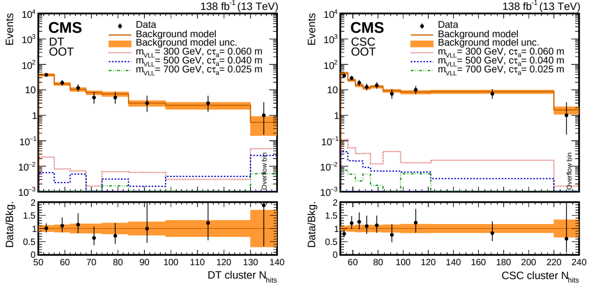
Figure 4: Distributions of the number of hits in the cluster ( N_{\text{hits}} ) for the DT (left) and CSC (right) cluster categories in the out-of-time (OOT) region. The black markers represent the data. The solid orange line and associated orange band show the background prediction and corresponding uncertainty. The red dotted, blue dashed and green dashed-dotted lines denote different signal hypotheses for a pseudoscalar boson with a mass of 2 GeV. The last histogram bin contains all overflow events. The lower panel in each plot shows the ratio of the data to the estimated background.
