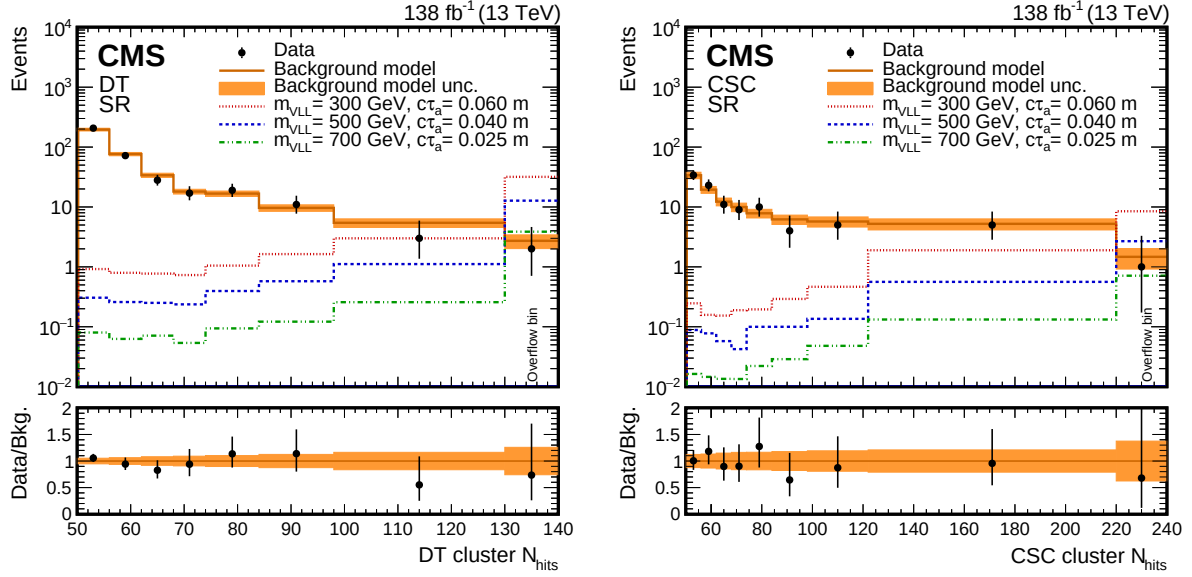
Figure 3: Distributions of the number of hits in the cluster ( N_{\text{hits}} ) for the DT (left) and CSC (right) cluster categories in the signal region (SR). The black markers represent the data. The solid orange line and associated orange band show the background prediction and corresponding uncertainty. The red dotted, blue dashed and green dashed-dotted lines denote different signal hypotheses for a pseudoscalar boson with a mass of 2 GeV. The last histogram bin contains all overflow events. The lower panel in each plot shows the ratio of the data to the estimated background.
