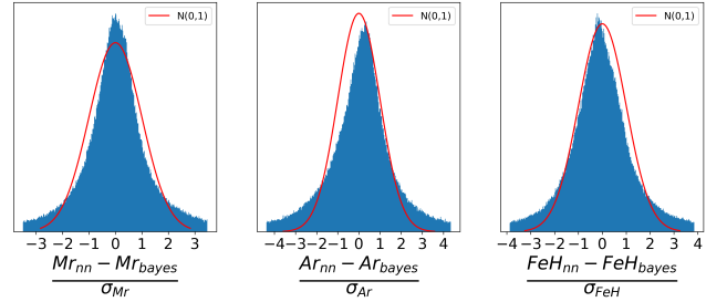
Figure 13. Histograms of residuals between NN and Bayesian estimates for M_r (left), A_r (middle), and [\text{Fe}/\text{H}] (right). The red curves show a normal distribution ( N(0, 1) ) for comparison.
