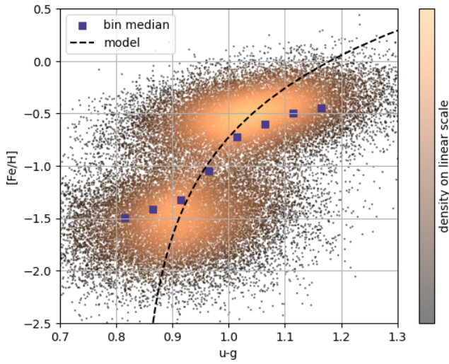
Figure 29. Binormal toy model illustrating the bias in photometric metallicity estimation caused by significant errors in u - g color. Analogous to Figure 28 except it uses a distribution made of two equal-size concatenated samples from the Gaussian distributions centered on [\text{Fe}/\text{H}] = -1.5 and [\text{Fe}/\text{H}] = -0.5 , and with \sigma equal to 0.3 dex and 0.2 dex, respectively.
