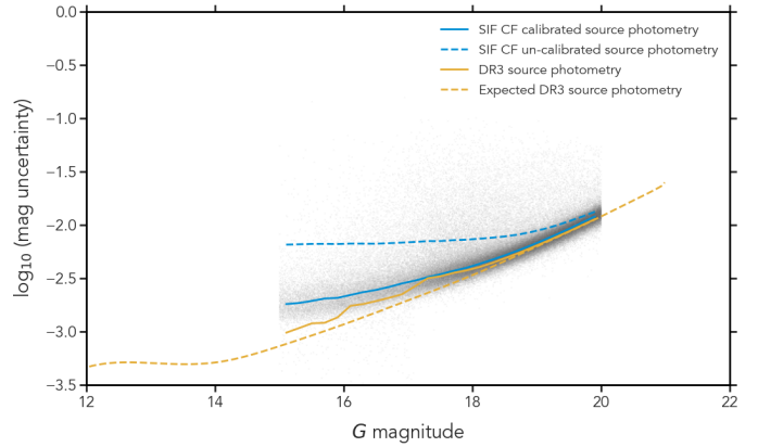
Fig. 5. Median G magnitude uncertainty versus G magnitude. G magnitude uncertainty for all calibrators with data density in grey, see the legend and text for a description of the various overlaid curves.
