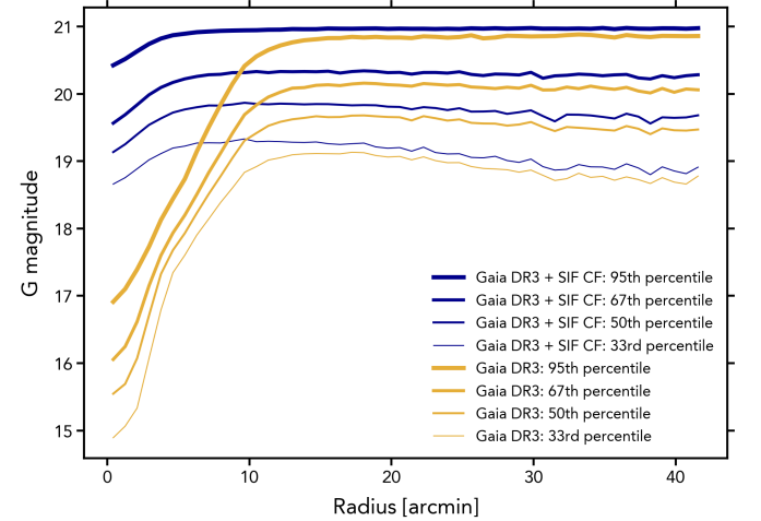
Fig. 16. Quantiles of the magnitude distribution versus distance to cluster centre. 33% (thin line), 50%, 67%, and 95% (thick line) for Gaia DR3 sources (yellow) and the combined catalogue (dark blue).
