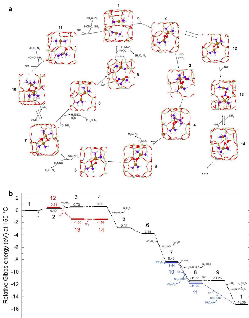
Figure 9. a) Proposed pathways of the NH 3 -SCR-DeNO x reaction connecting the most probable intermediates (based on experimental observations and computations). Reaction intermediates are shown as ball-and-stick models while the CHA cage is shown as a wireframe. For better clarity and visibility of the intermediates, a part of the CHA cage is removed. Oxygen atoms are colored red, nitrogen blue, hydrogen white, copper brown, silicon light yellow, and aluminum grey; b) Relative Gibbs energies of the stable intermediates with colors depicting different pathways or branches of the cycle.
