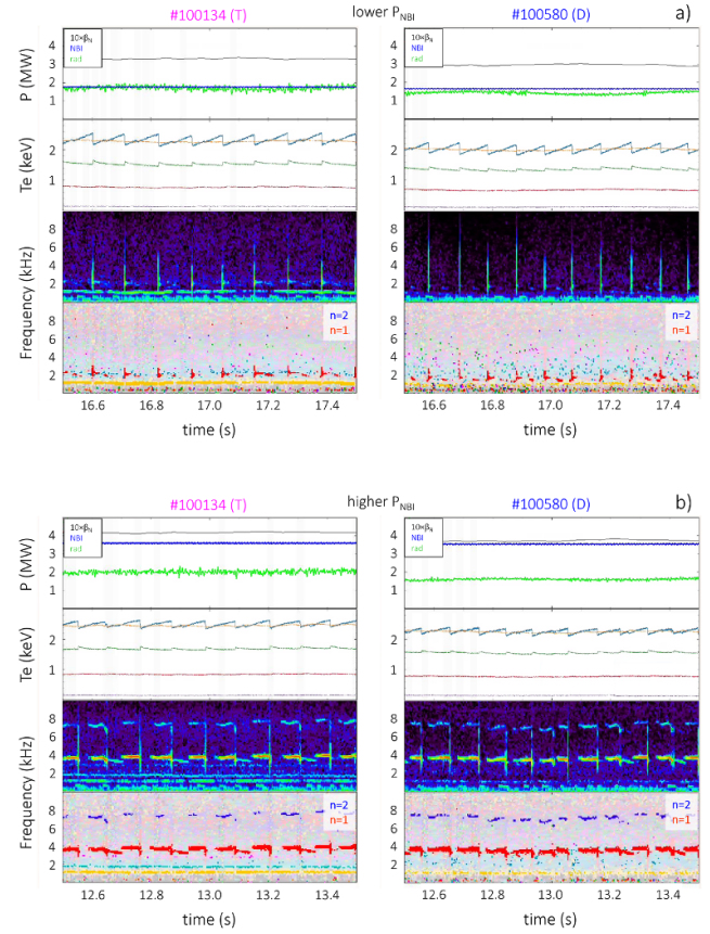
Figure 21. MHD analysis of the T pulse (left) and the D pulse (right). From top to bottom: total radiated power (green line), NBI power (blue line), electron temperature at different radii, spectrogram and toroidal mode number analysis from Mirnov coils.
