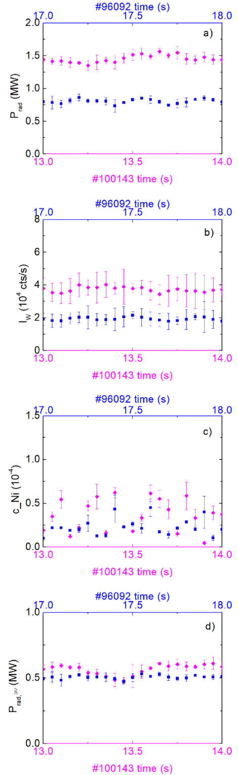
Figure 6. (a) The total radiated power, (b) I_W , (c) c_{Ni} and (d) divertor radiated power P_{rad,div} in the time of interest for the T pulse #100143 ( t = 13 – 14 s) and for the D pulse #96092 ( t = 17 – 18 s).
