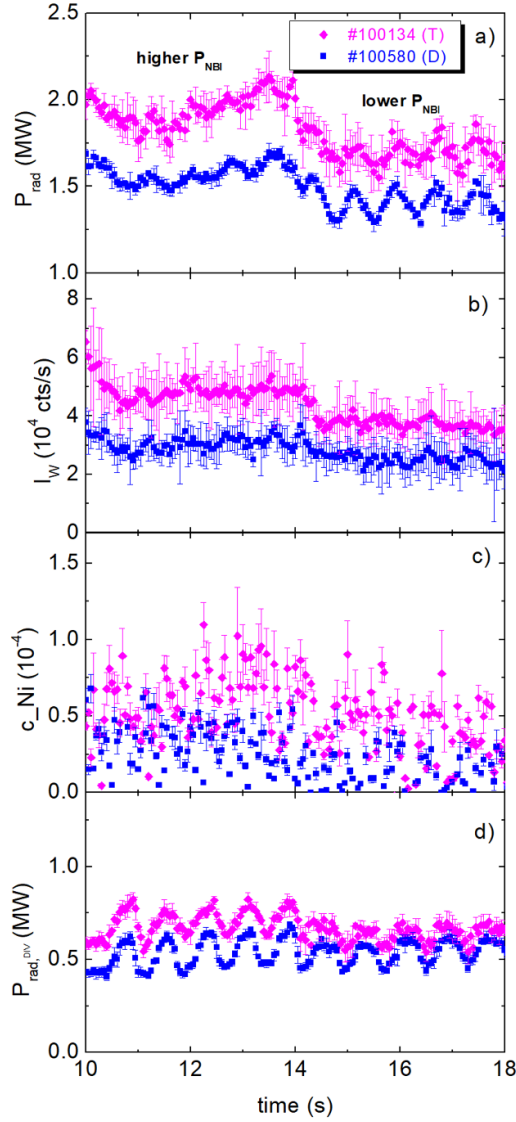
Figure 17. Time evolution of (a) the radiated power, (b) I_w , (c) c_{Ni} and (d) the divertor radiated power in the T pulse #100134 and the D pulse #100580 corresponding to two NBI power level steps.
