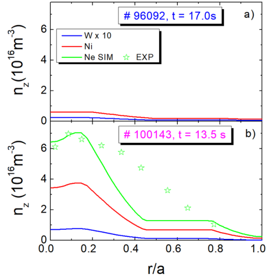
Figure 12. The COREDIV nickel (red line), tungsten (blue line) and neon (green line), density profiles for (a) the D pulse at t = 17 s and (b) the T pulse at t = 13.5 s. The stars correspond to experimental Ne density profiles determined from the CX diagnostic.
