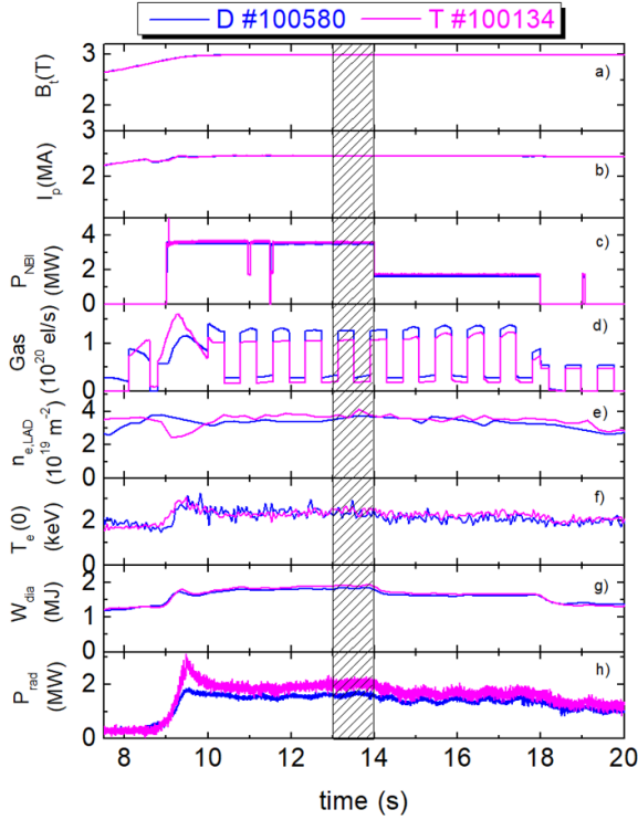
Figure 13. Time evolution of (a) the magnetic field B_t , (b) plasma current I_p , (c) the NBI heating power P_{NBI} , (d) major gas injection level, (e) the line average electron density n_{e,lad} , (f) the central electron temperature T_e(0) , (g) the diamagnetic energy W_{dia} , and (h) the total radiated power P_{rad} , for D (blue, #100580) and T (magenta, #100134) discharges. The two vertical black bars indicate the time of interest in both pulses, at t = 13 – 14 s.
