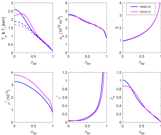
Figure 14. Comparison of the main dimensional ( n_e , T_e , T_i ) and dimensionless plasma profiles ( \rho^* , \nu^* , q , \beta_n ) averaged in time between t = 13 – 14 s in D (#100580) and T (#100134) discharge as a function of the normalized radius.
