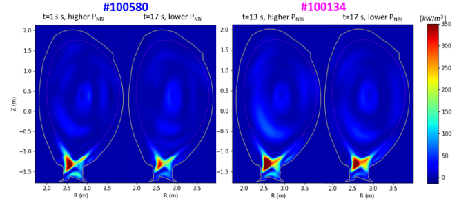
Figure 15. Tomographic reconstruction of the radiated power density in pulse #100580 for the D plasmas and in pulse #100134 for the T plasmas, for higher NBI power level at t = 13 s and lower NBI power level at t = 17 s, respectively.
